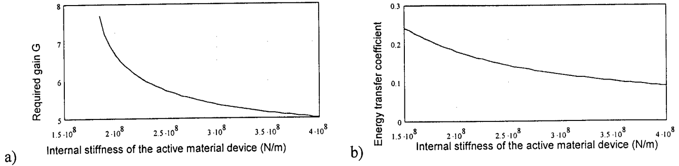
Figure 10 Variation of the required gain G and energy transfer coefficient with the internal stiffness of the actuator, considering the displacement amplification efficiency \eta_m=0.8 .
