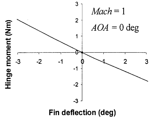
Figure 3 Moment-deflection diagram for AOA = 0°
