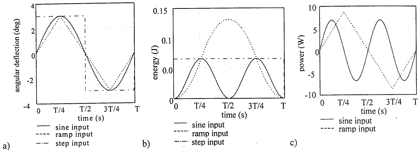
Figure 5 Variation of the required actuation energy and power within a cycle: a) input signal; b) required energy within a cycle; c) required power within a cycle
