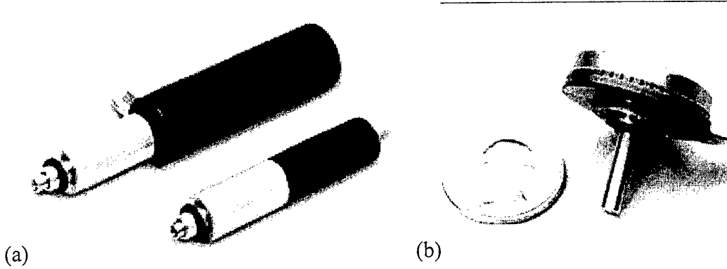
Figure 7 a) Burleigh Inchworm Linear Motors; b) Piezo Systems Ultrasonic Motor
