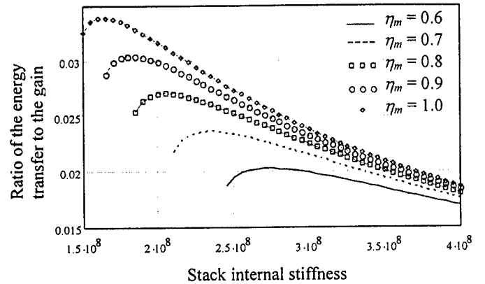
Figure 11 Variation of the optimum metric R=E'_e/G with the internal stiffness and the displacement amplification mechanism efficiency
