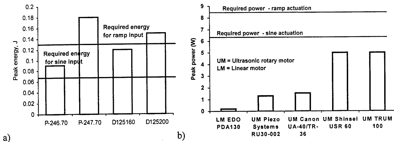
Figure 9 Present commercially available actuators meeting the missile fin reduced envelope energy requirements: a) comparison of the direct actuation devices deliverable energy with the required energy for sine and ramp input; b) comparison of the smart materials motors maximum deliverable power with the required power for sine and ramp excitations
