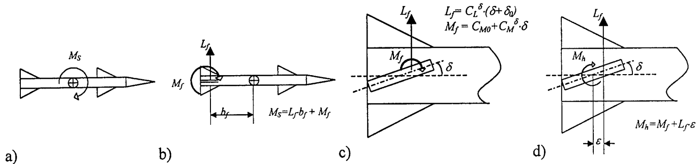
Figure 2 Steering moment delivery through missile fin deflection, at zero AOA
