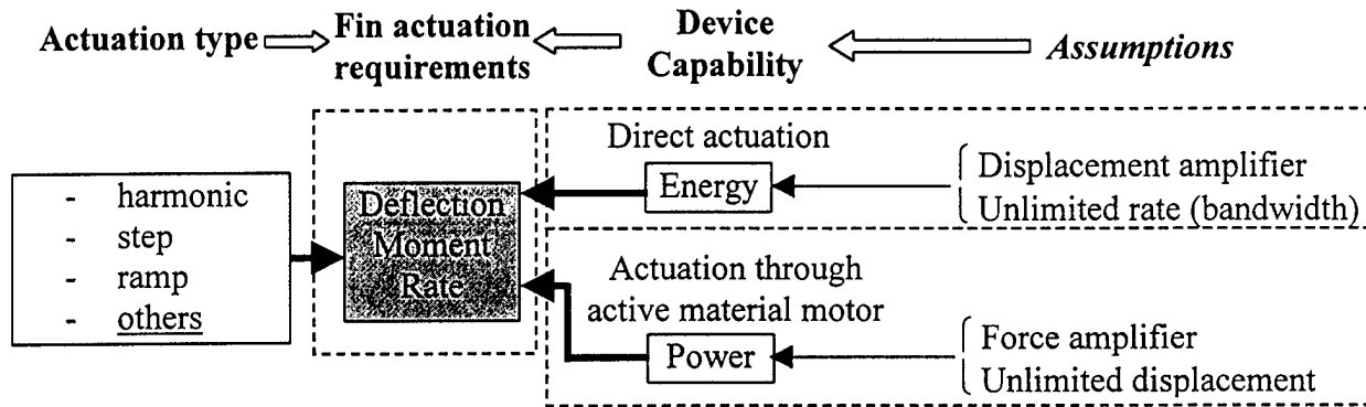
Figure 4 Meeting the requirements involves input signal design and smart-materials device capabilities
