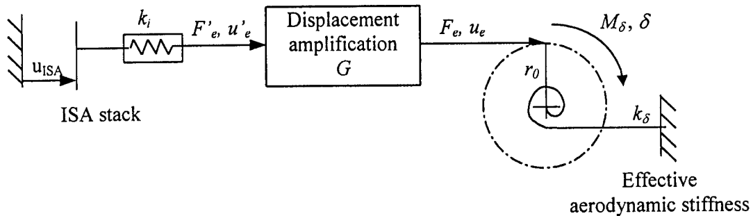
Figure 8 Schematic drawing of the displacement amplification process
