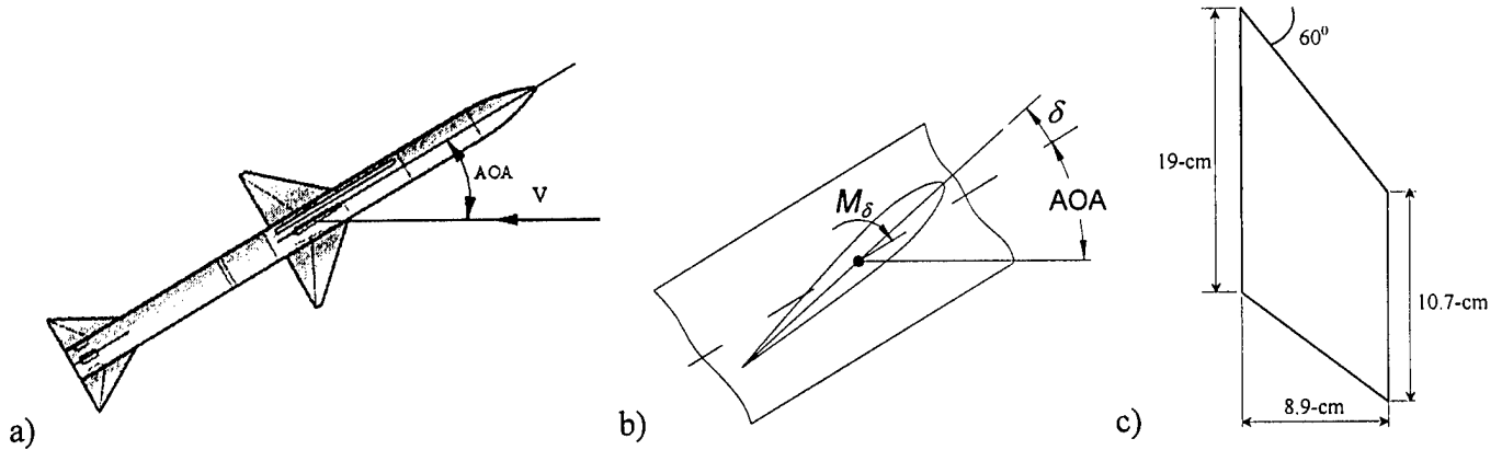
Figure 1 Missile control surface loads modeling: a) missile in flight; b) moment and deflection; c) fin plan form.
