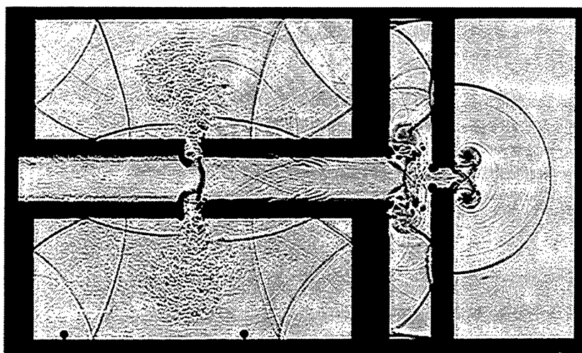
b) t = 0.260 ms
