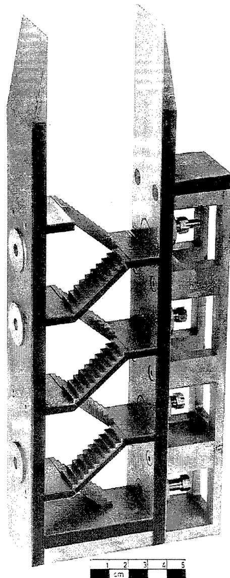
Figure 30. Stairwell models
