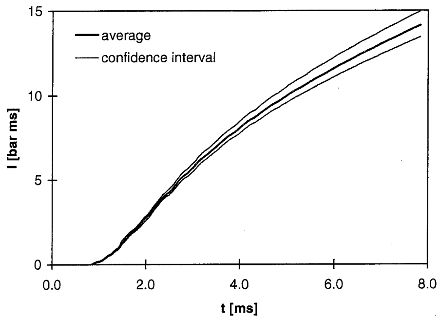
Figure 63. Ensemble-averaged overpressure impulse and corresponding confidence bandwidth at gage 9 for the standard configuration. Ensemble of eight tests.
