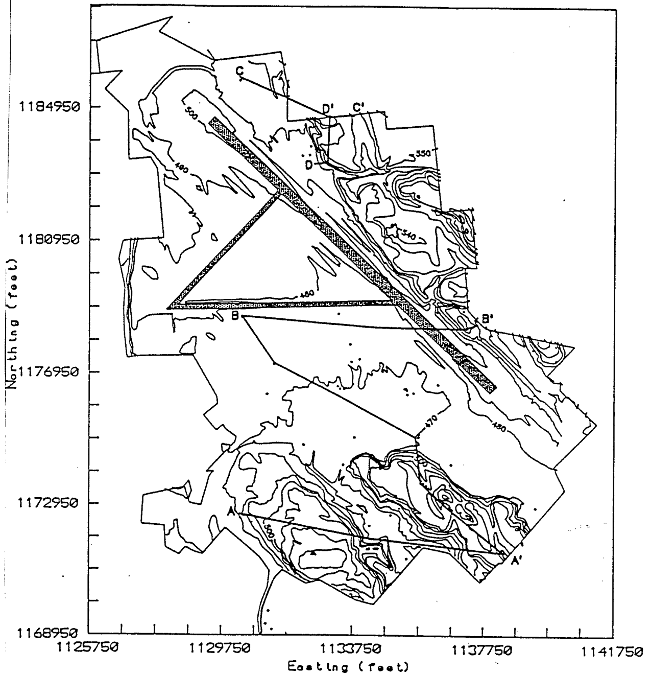
Geologic Cross-section locations for the GAFB Hydrogeology Study. Points are well locations.
