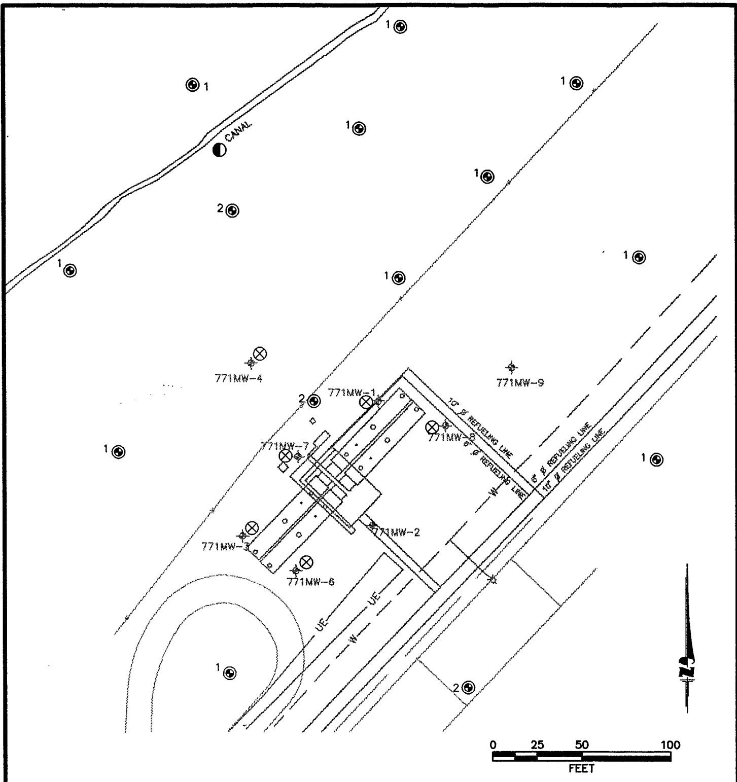
FIGURE 3.3 PROPOSED GEOPROBE SAMPLING AND/OR MONITORING POINT INSTALLATION LOCATIONS Pumphouse 5 Intrinsic Remediation TS Griffiss AFB, New York PARSONS ENGINEERING SCIENCE, INC. Denver, Colorado
