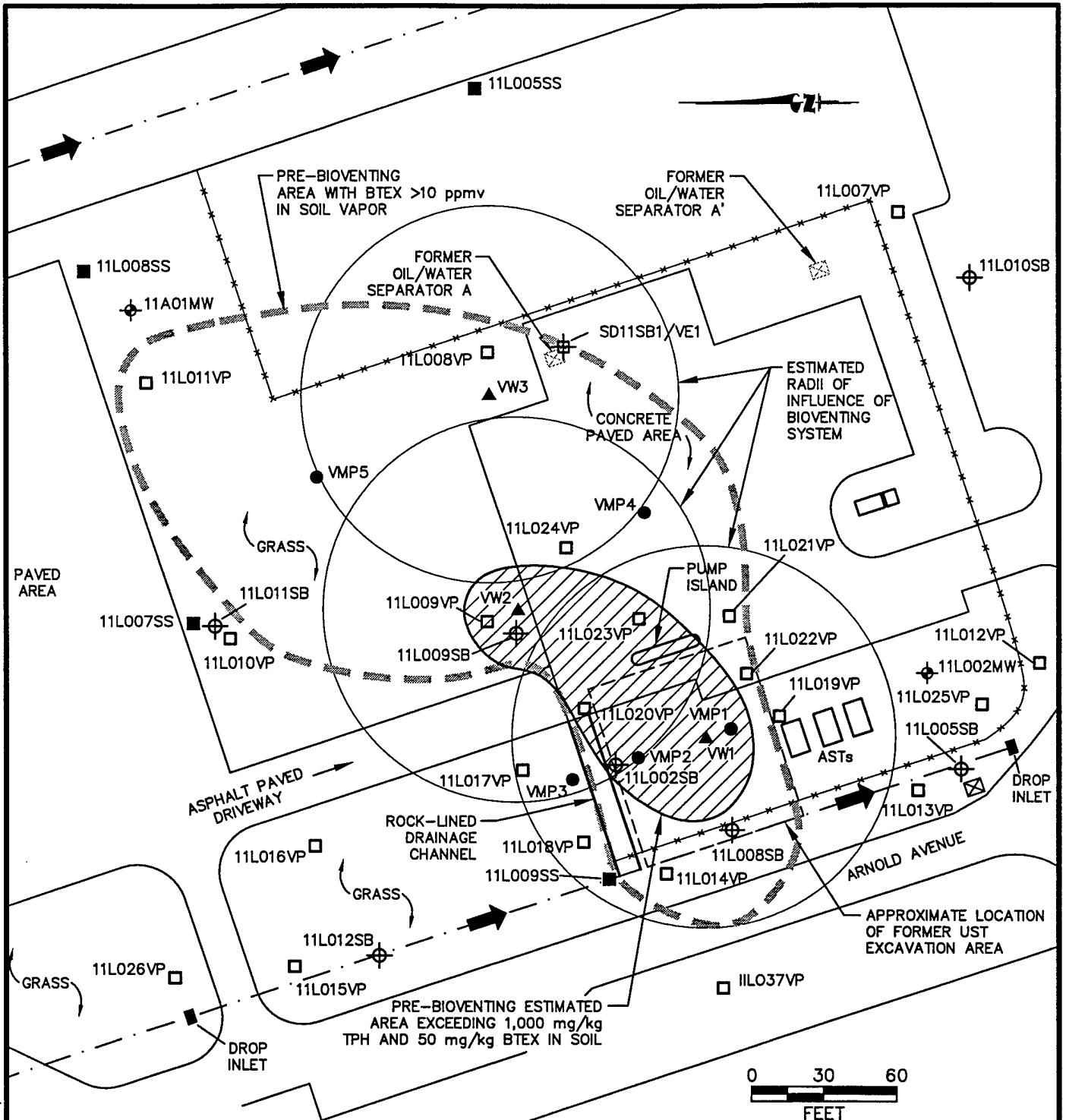
FIGURE 2.4 SITE MAP AND PREVIOUS SAMPLING LOCATIONS IN THE UST EXCAVATION AREA AND ADJOINING AREAS IRP Site SD-11 AGE Maintenance Area Beale AFB, California PARSONS ENGINEERING SCIENCE, INC. Denver, Colorado
