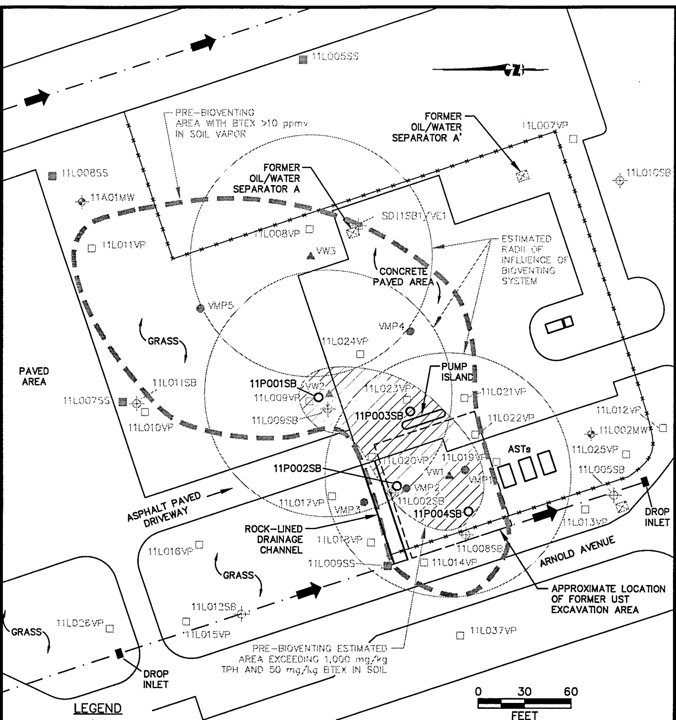
FIGURE 3.1 PROPOSED CONFIRMATION SOIL SAMPLING LOCATIONS
