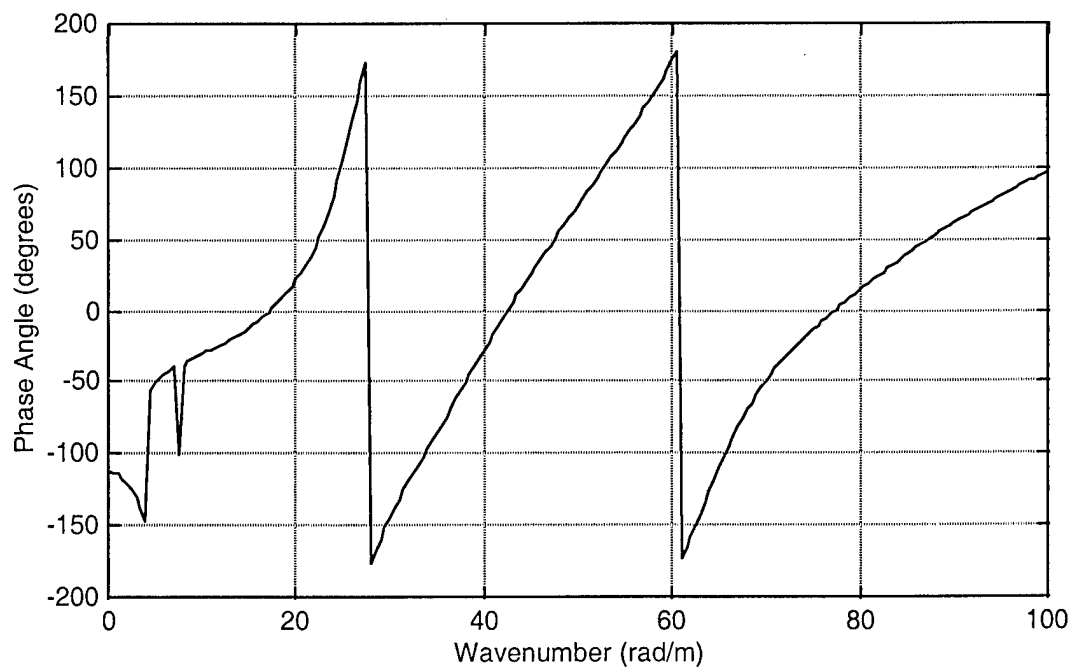
Figure 26. Transfer Function of a Triple Plate with Fluid Load (Equation (671)) at 1000 Hz
