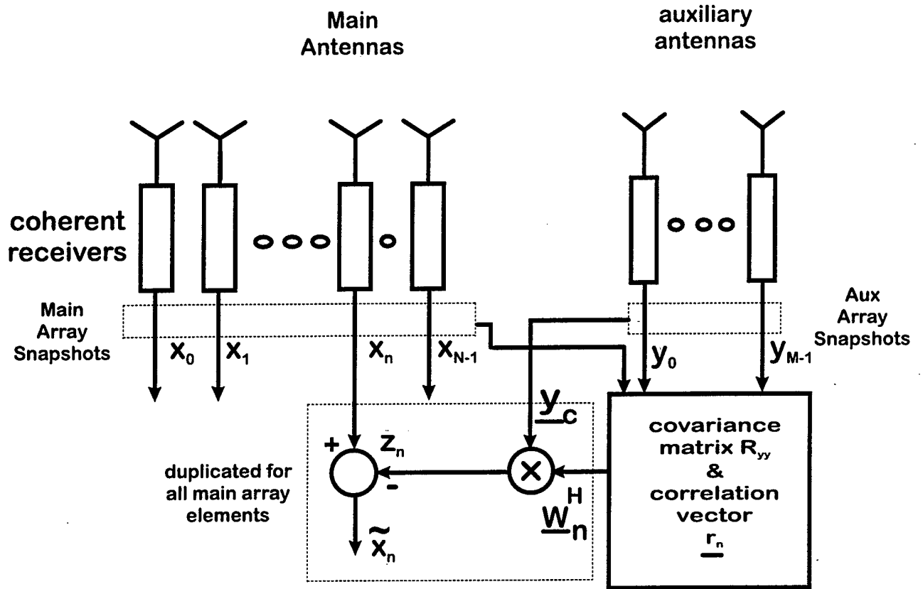
Figure 4. Schematic diagram of an interference cancellation algorithm .
