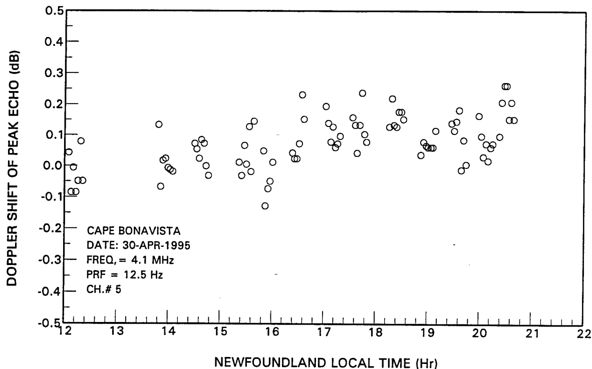
Figure A.6 Variation of Doppler shift of the peak ionospheric clutter.
