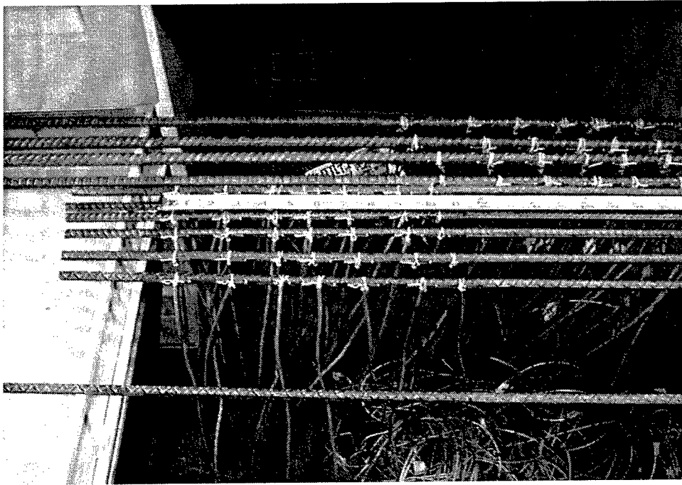
Figure 3. Strain gaged reinforcement
