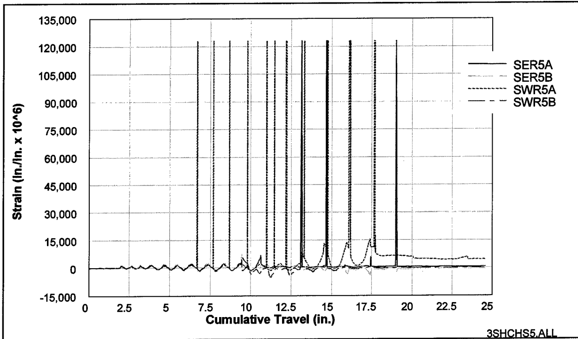
Figure C6. Strains measured 4.0 in. above and below cold joint, 3SHCH
