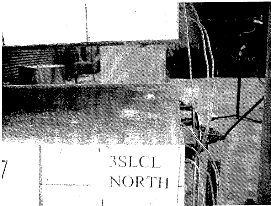
Figure 14. Closeup view of 3SLCL failure plane
