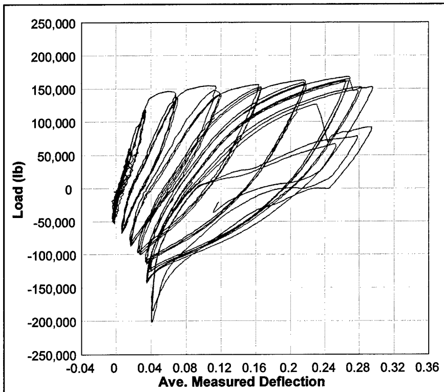
Figure 46. Load-deflection curve for repaired model in experiment 5SHCH
