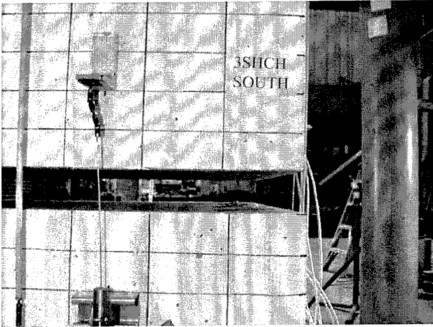
Figure 23. Postexperiment view of 3SHCH failure plane
