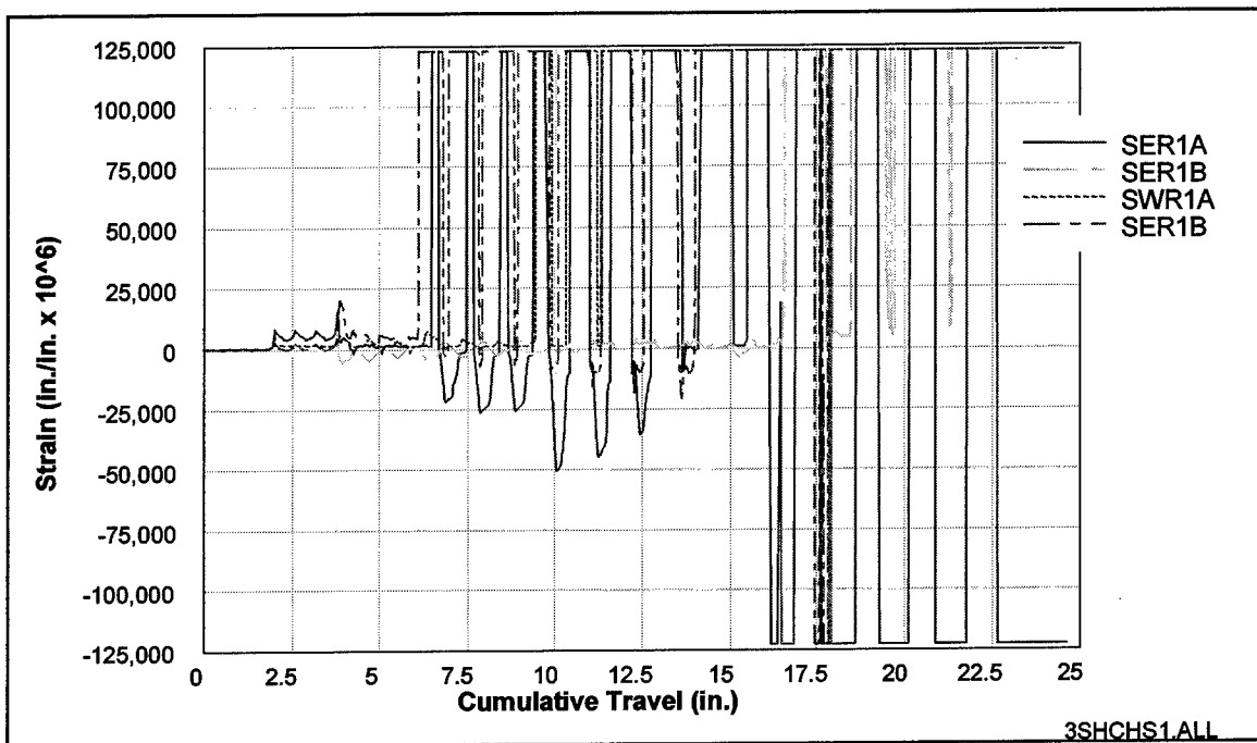
Figure C2. Strains measured 0.5 in. above and below cold joint, 3SHCH
