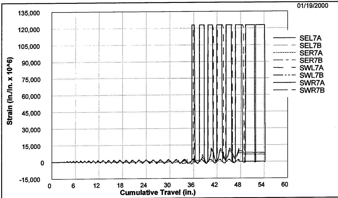
Figure C66. Strains measured 8.5 in. above and below cold joint, 5SLCL
