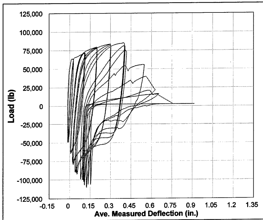
Figure 30. Load-deflection curve for experiment 4SHCM
