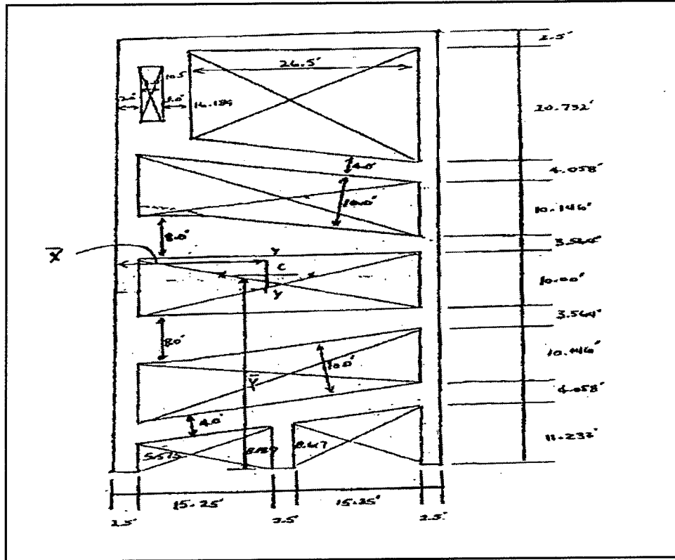
Figure 54. Schematic of critical section at 395-ft elevation
