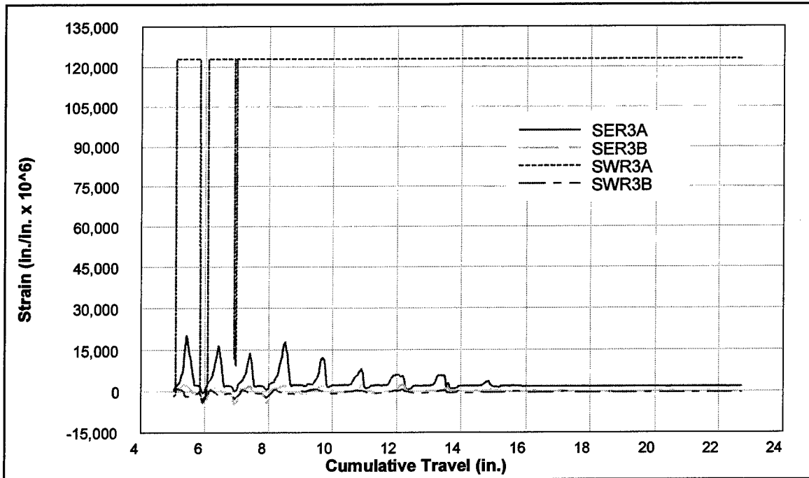
Figure C25. Strains measured 2.0 in. above and below cold joint, 3SLCL
