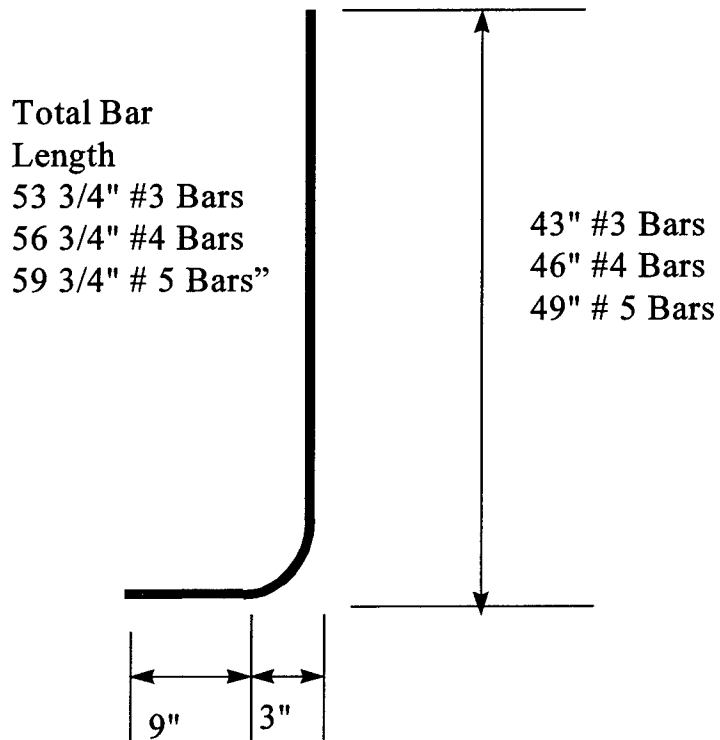
Figure A6. Dimensions of lower rebar
