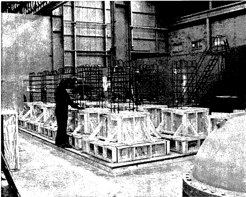
Figure 9. Reinforcement of top half of models
