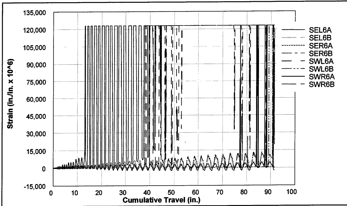
Figure C49. Strains measured 6.5 in. above and below cold joint, 5SHCL
