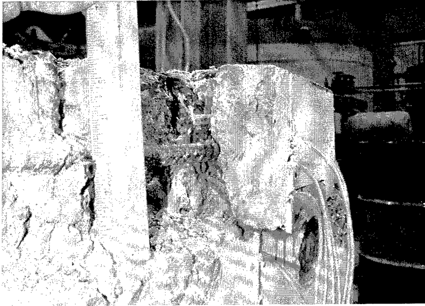
Figure 37. View of 5SLCH failure plane cover concrete spall
