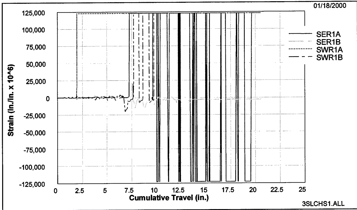
Figure C16. Strains measured 0.5 in. above and below cold joint, 3SLCH
