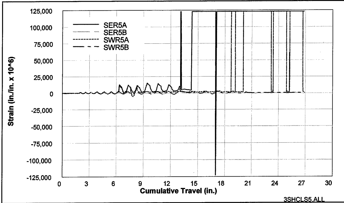
Figure C13. Strains measured 4.0 in. above and below cold joint, 3SHCL
