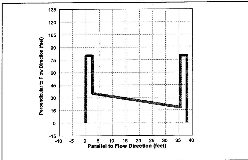
Figure 55. Outline of simplified critical section at 395-ft elevation
