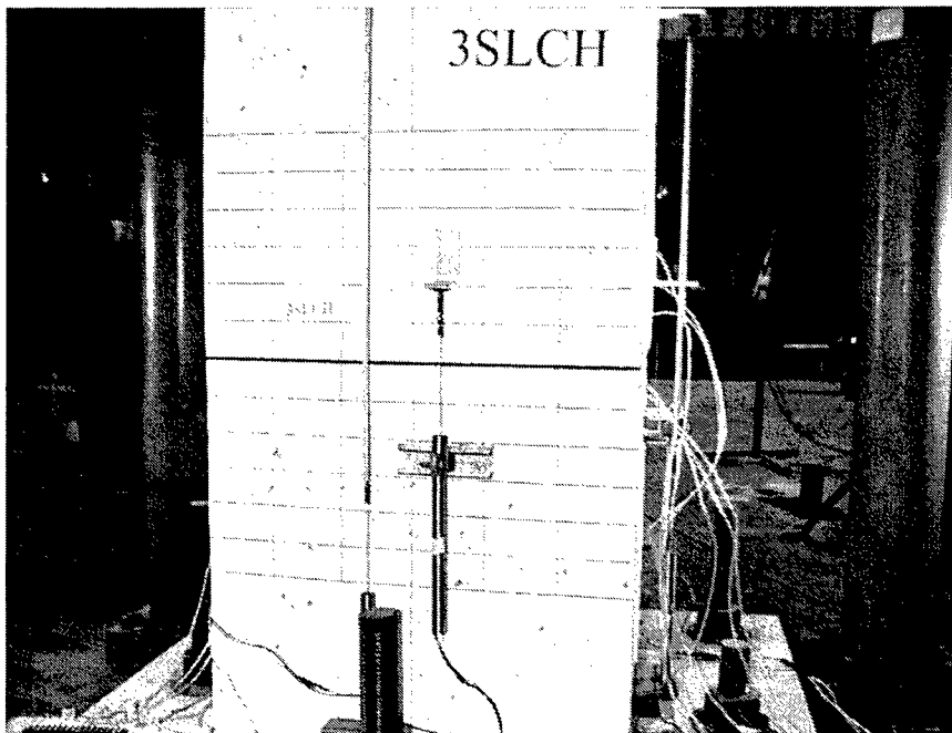
Figure 16. West view of 3SLCH failure plane
