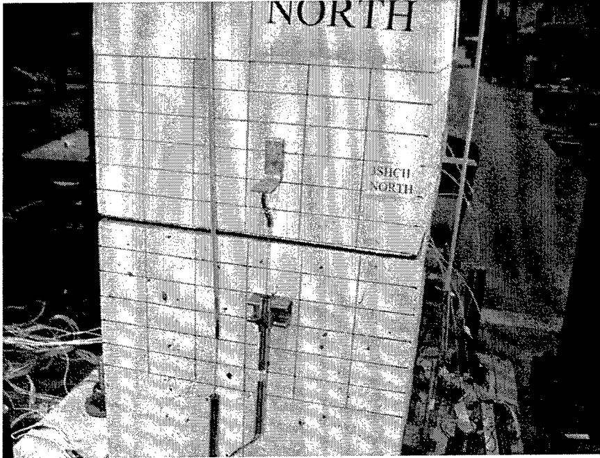
Figure 22. North view of 3SHCH failure plane
