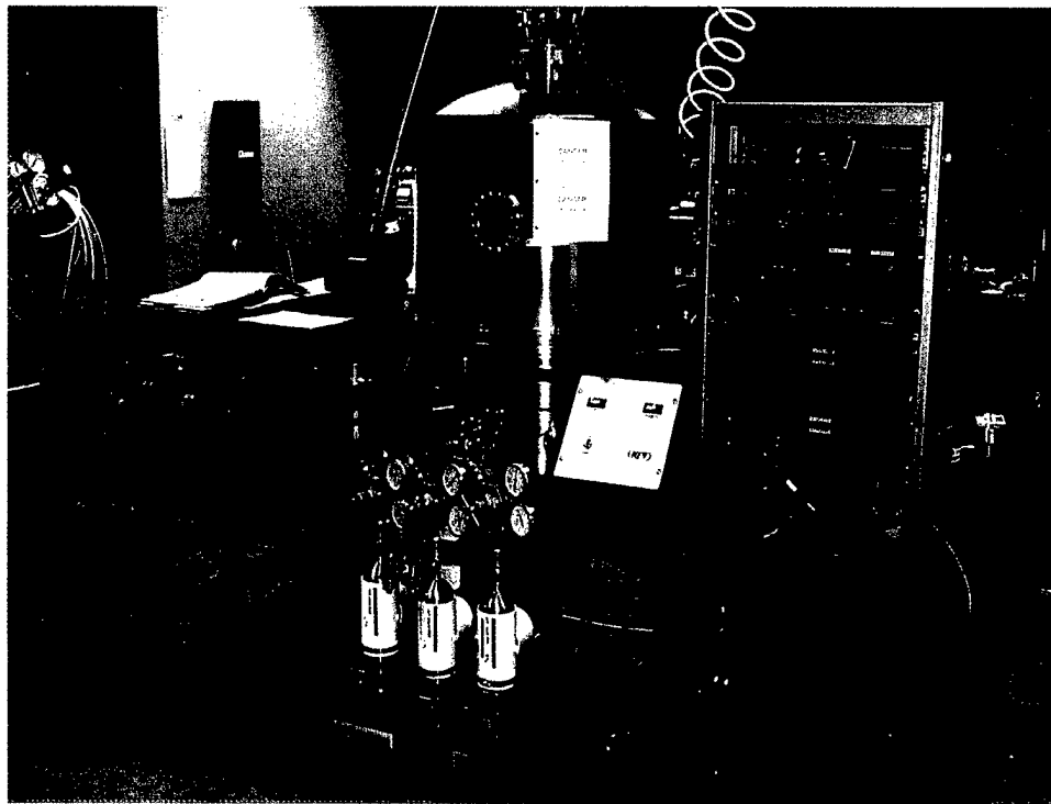
Figure 2: Photograph of the IBAD laboratory. The 3 e-beam evaporators and ion beam gun are mounted on flanges on the floor plate of the 36-inch vacuum chamber. The upper 24 inches of the chamber can be lifted to expose the e-gun crucibles and the rotating temperature controlled target holder. Two 6-kw e-beam power supplies and scanning controls are in the rack at the right. The single 15-kw e-beam supply is visible behind the rack. Three gas supplies are available from the blue panel and a fourth gas can be supplied from the cylinder on the left. The sloping panel at left is the ion beam controls and the white panel is the vacuum and chamber lift controls. A 10-inch Crypump and its compressor are obscured under and behind the chamber.
