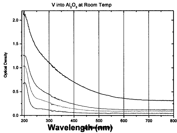
Figure 12: Al 2 O 3 implanted with Vanadium
