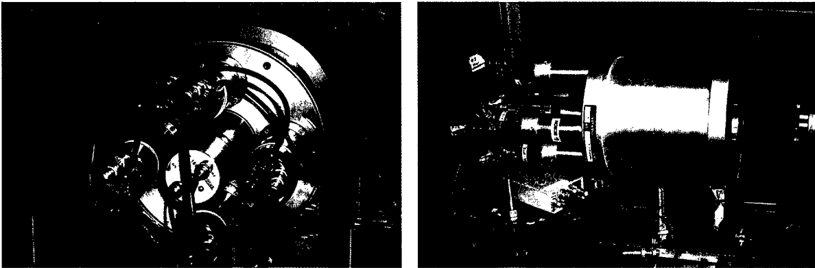
Figure 5: The detector array developed at AAMU and dedicated to depth profiling hydrogen content in IBAD films and other solid materials. The hydrogen concentration in a target is proportional to the number of 4.44 MeV gamma rays produced by the nuclear reaction {}^1\text{H}({}^{15}\text{N}, \alpha\gamma){}^{12}\text{C} when the target is bombarded with a {}^{15}\text{N} ion beam. Background is rejected by a coincidence scheme such that a few ppm hydrogen may be detected.
