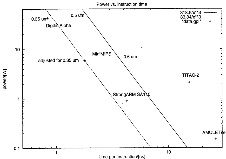
Figure 1: Comparison of E * t^2 figures for different microprocessors. The solid line represents the iso- E * t^2 line for the MiniMIPS in loglog scale. The dotted line is the iso- E * t^2 adjusted for 0.35 micron technology. The points closer to the origin correspond to better performance.
