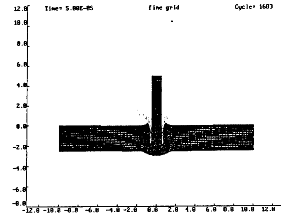
(f) Fine Grid - Deformation at 50 \mu s
