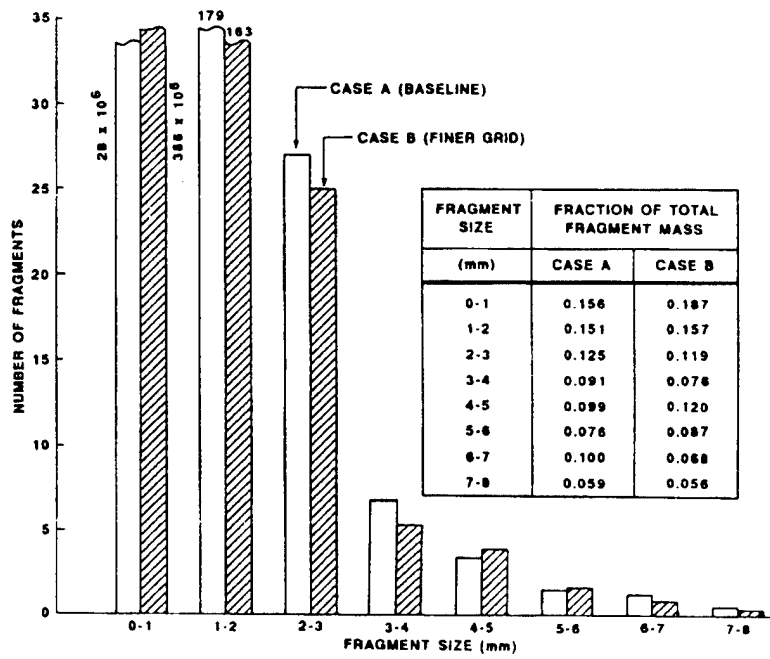
Figure 8. Fragment Size Distribution vs. Grid Size [25].
