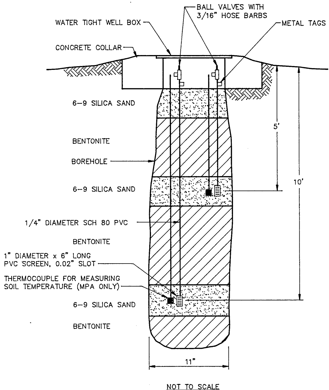
FIGURE 3.3 SITE 16 MONITORING POINT CONSTRUCTION DETAIL EDWARDS AFB, CALIFORNIA ENGINEERING-SCIENCE, INC. Denver, Colorado ES
