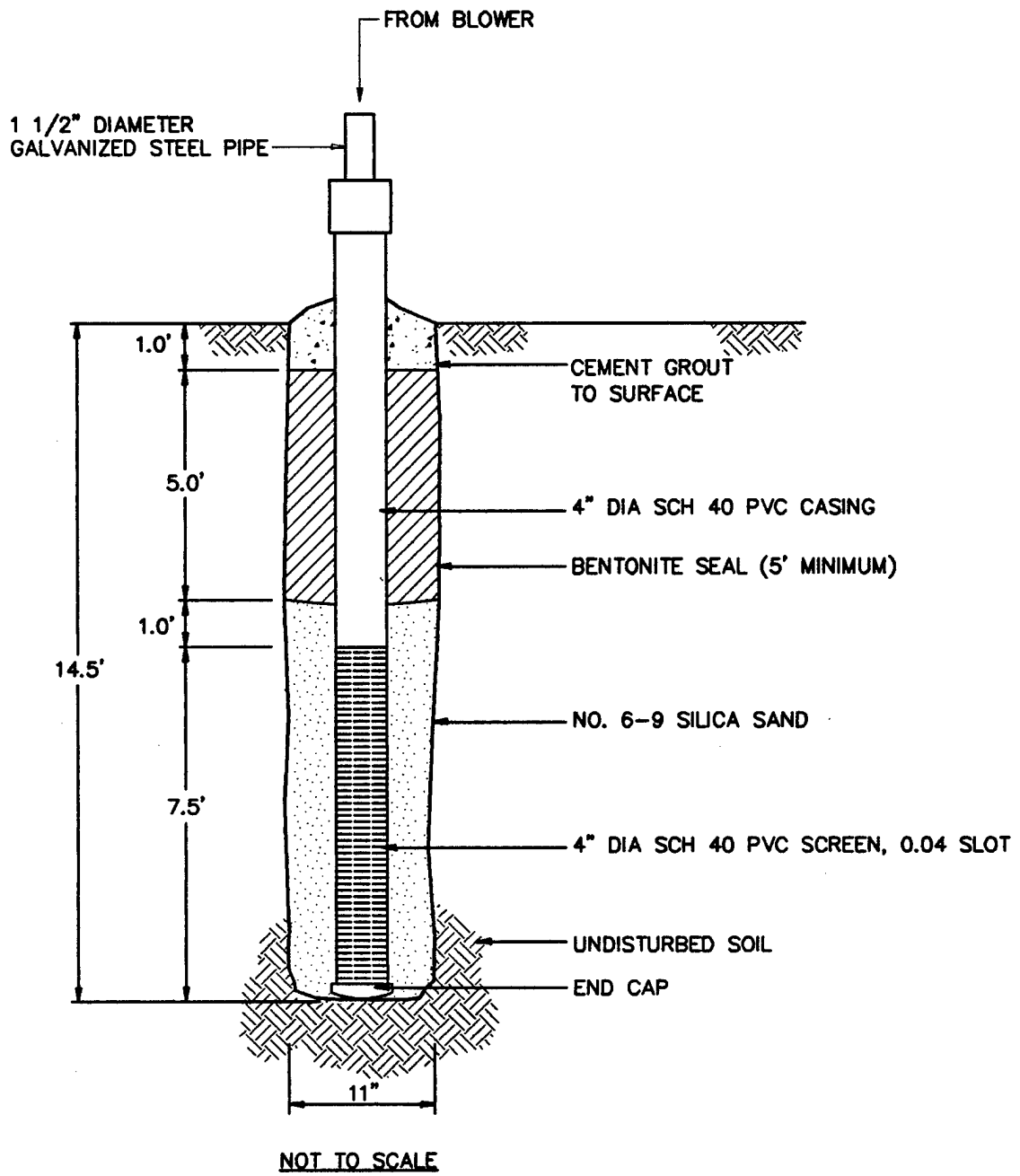
FIGURE 2.3 SITE 21 RECORD DRAWING INJECTION VENTING WELL CONSTRUCTION EDWARDS AFB, CALIFORNIA ENGINEERING-SCIENCE, INC. Denver, Colorado ES
