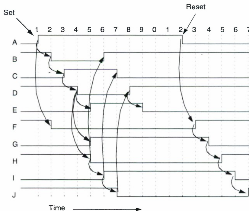
Figure 6-2. Relative timing diagram for the pulse-generator circuit. The signals A through J are labeled in Figure 6-1. The arrows indicate how the signals propagate through the circuit.
