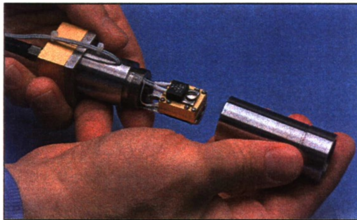
Figure 1-1. Photograph of optical head of a microchip-laser-pumped periodically poled lithium niobate optical parametric generator (OPG) with OPG cover removed.
