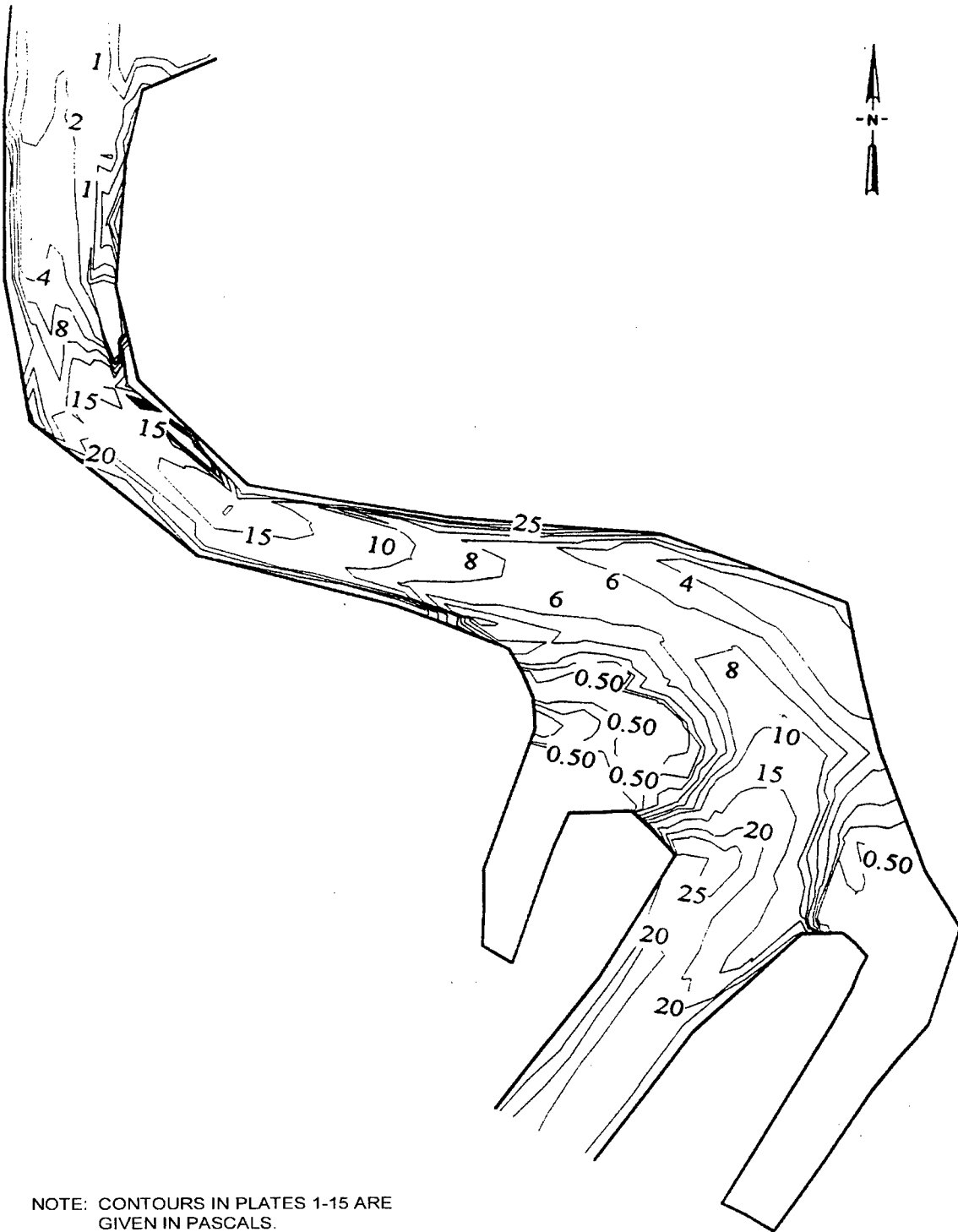
COMPUTED BED SHEAR STRESS CONTOURS REACH 1, PREDREDGING, LOW-WATER DATUM 100-YEAR FLOOD DISCHARGE
