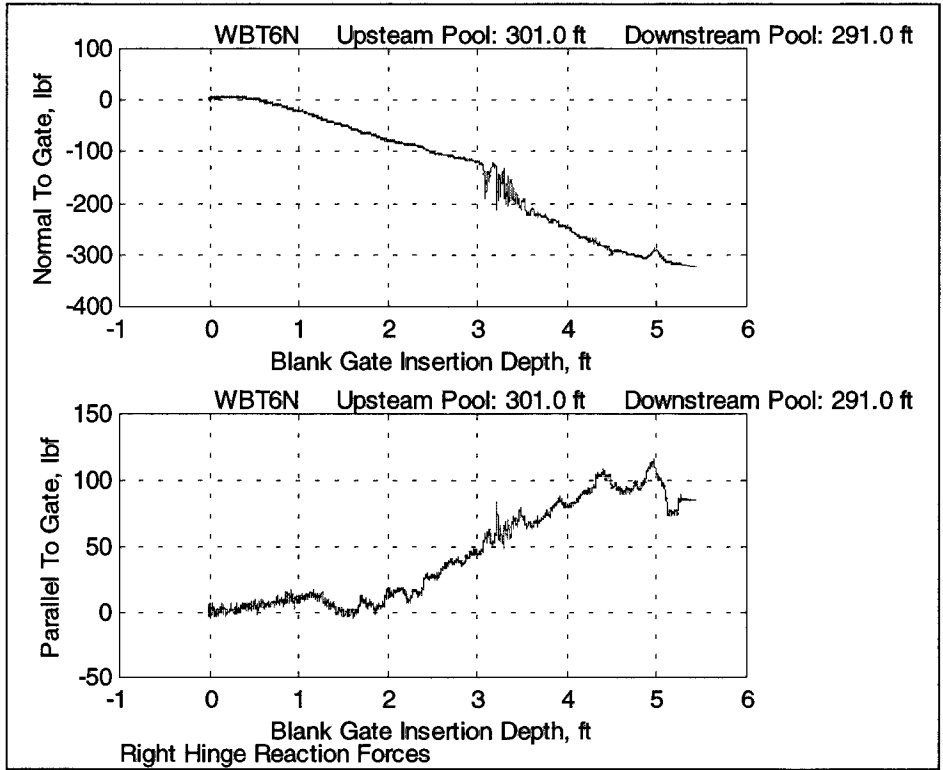
Figure 48. Right hinge reactions for test OLMWBT6N
