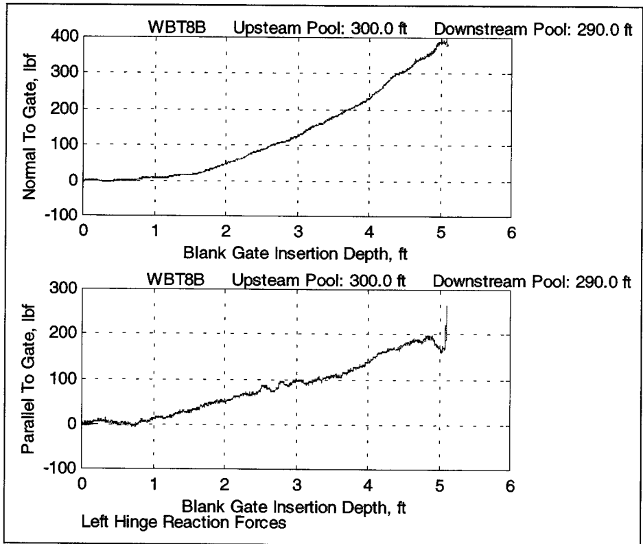
Figure 57. Left hinge reactions for OLMWBT8B
