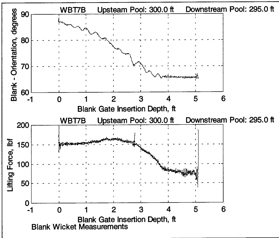
Figure 55. Lifting force and blank orientation for test OLMWB7B
