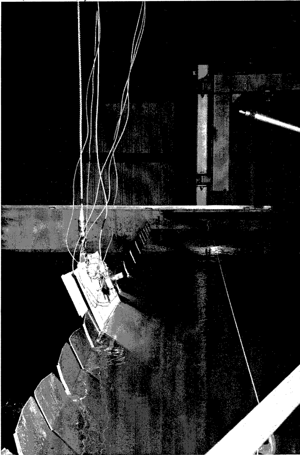
Figure 17. View of the blank, seated on wicket gate #5 at an angle of 65 deg, prior to removal. Headwater 300; Tailwater 295; 5-ft differential
