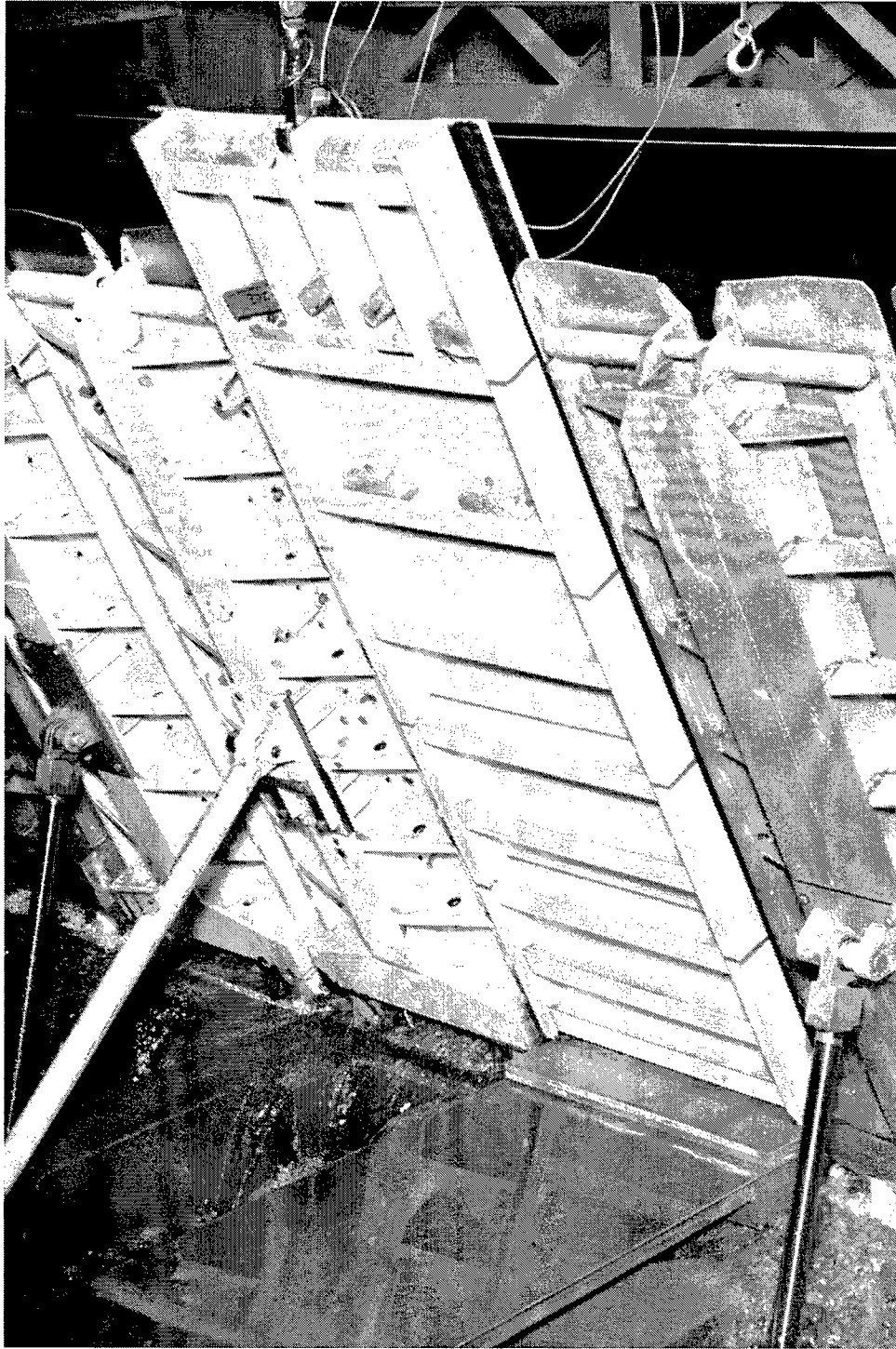
22294-043.jpg Figure 26. View from the walk, looking upstream at the blank seated on wicket gate #5, showing the weights located in the top three channels. Dry bed photograph
