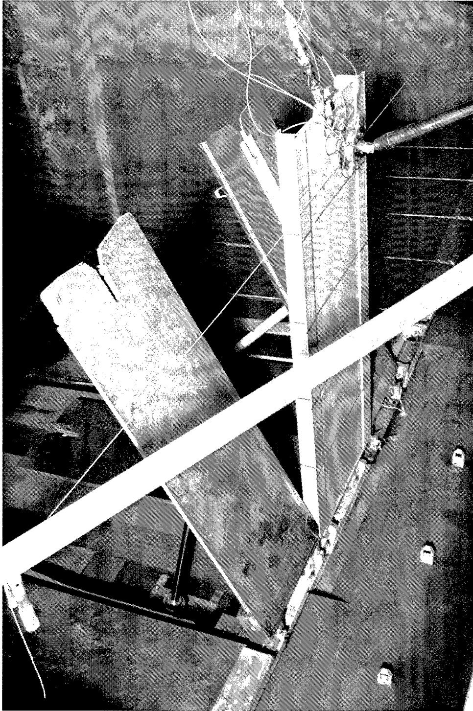
0004-027.jpg Figure 2. View from the walk, looking downstream at the blank seated on wicket gate #5 at an angle of 90 deg. Dry bed photograph
