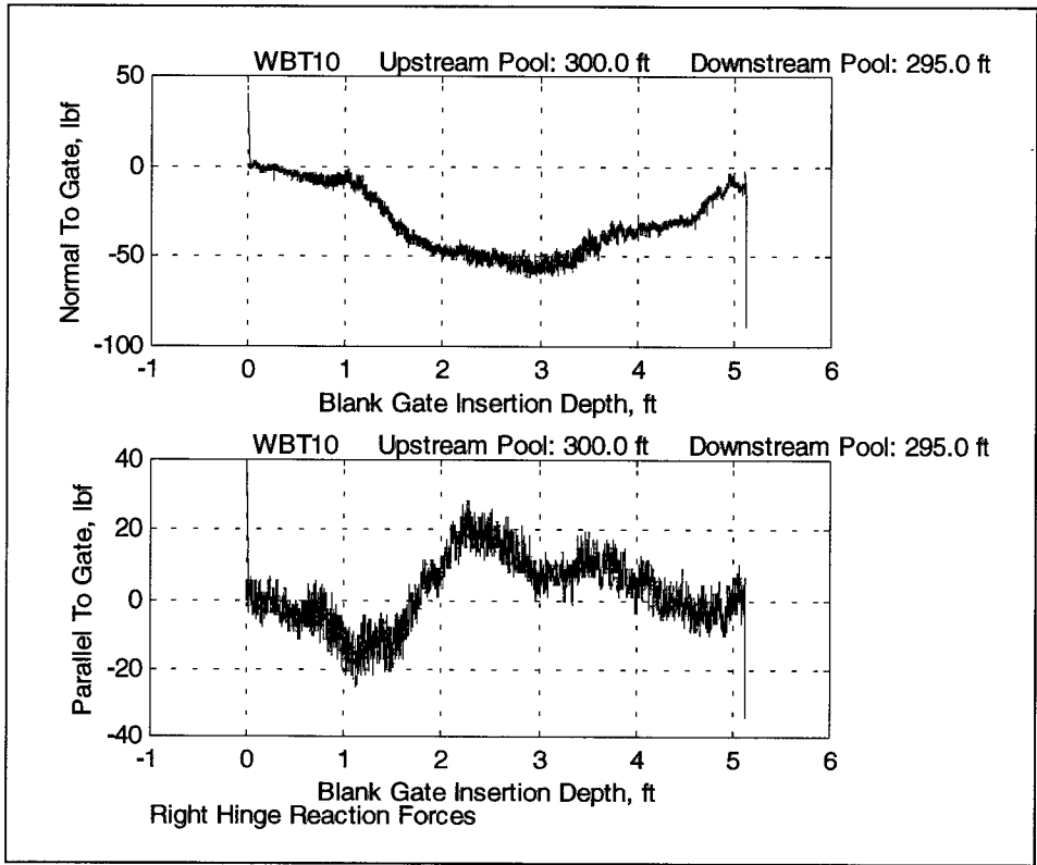
Figure 28. Right hinge reactions for OLMWBT1
