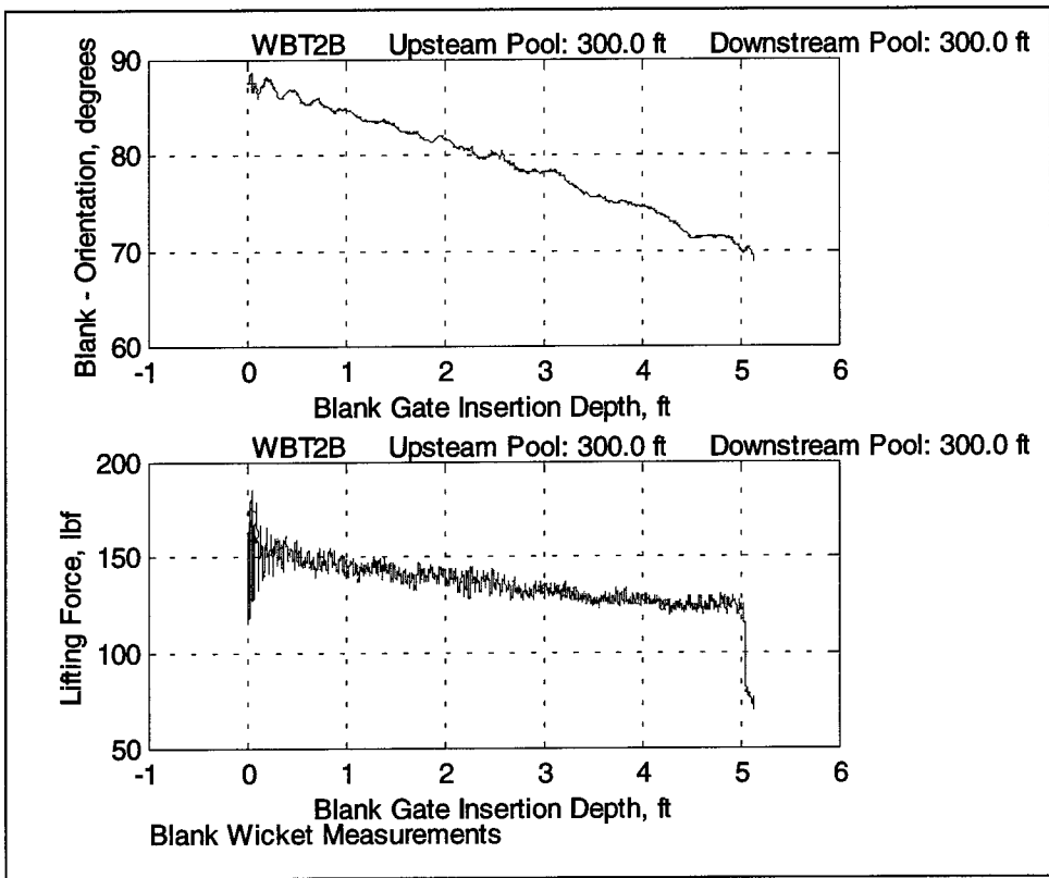
Figure 35. Lifting force and blank orientation for test OLMWBT2B
