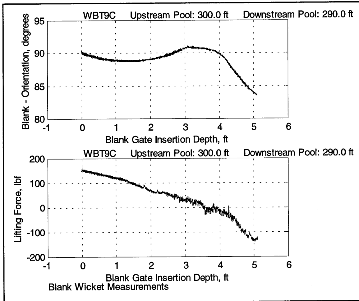
Figure 63. Lifting force and blank orientation for test OLMWBT9C
