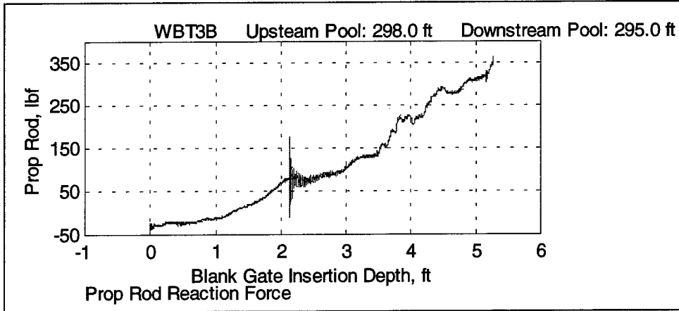
Figure 38. Prop rod force for test OLMWBT3B
