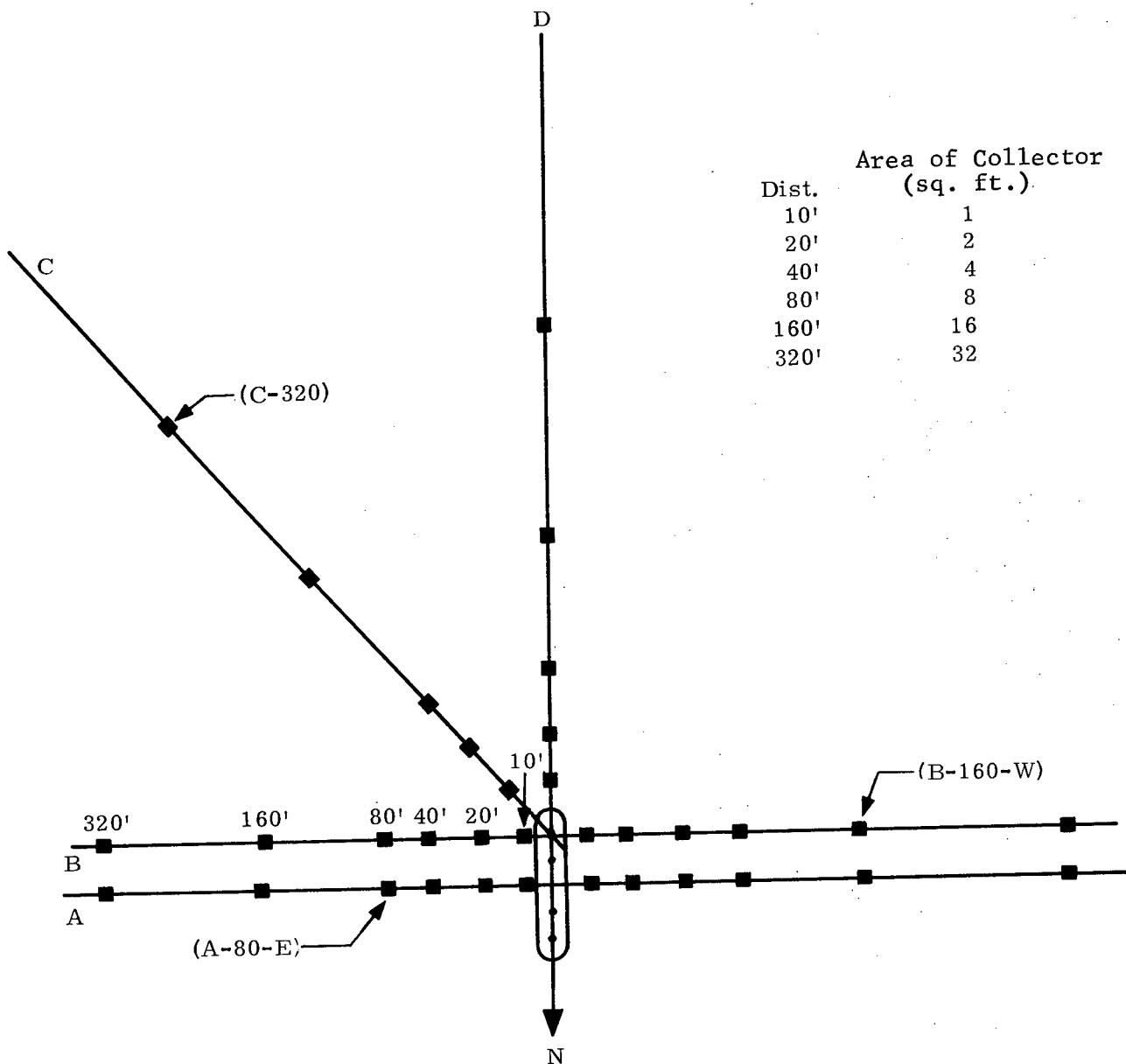
Figure 4. Pick ax earth dam sample collection pads
