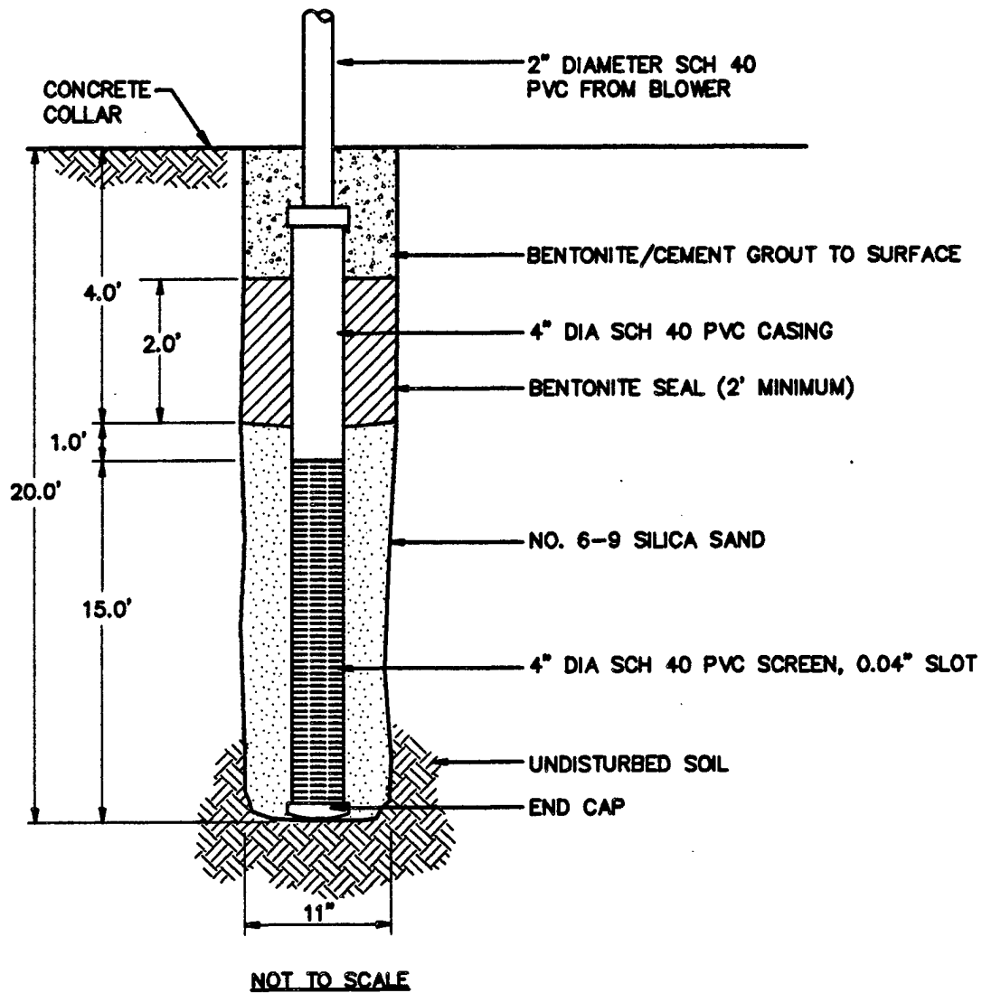
FIGURE 3.2 PROPOSED INJECTION VENT WELL CONSTRUCTION DETAIL SITE 6B, TANK 191 US Coast Guard Support Center Kodiak Kodiak, Alaska ENGINEERING-SCIENCE, INC. Denver, Colorado
