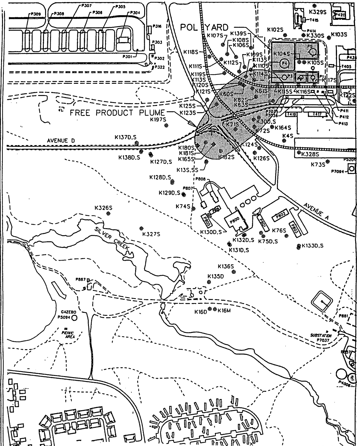
LEGEND # EXISTING MONITORING WELL LOCATIONS (APPROXIMATE) SOURCE: PILOT-SCALE FREE PRODUCT RECOVERY STUDY R.E. WRIGHT ASSOCIATES, SEPTEMBER 1991 FIGURE 1-2 PROJECT 9044 - POL SITE FREE PRODUCT PLUME MAP PRE-DESIGN REPORT K. I. SAWYER AIR FORCE BASE MARQUETTE, MICHIGAN
