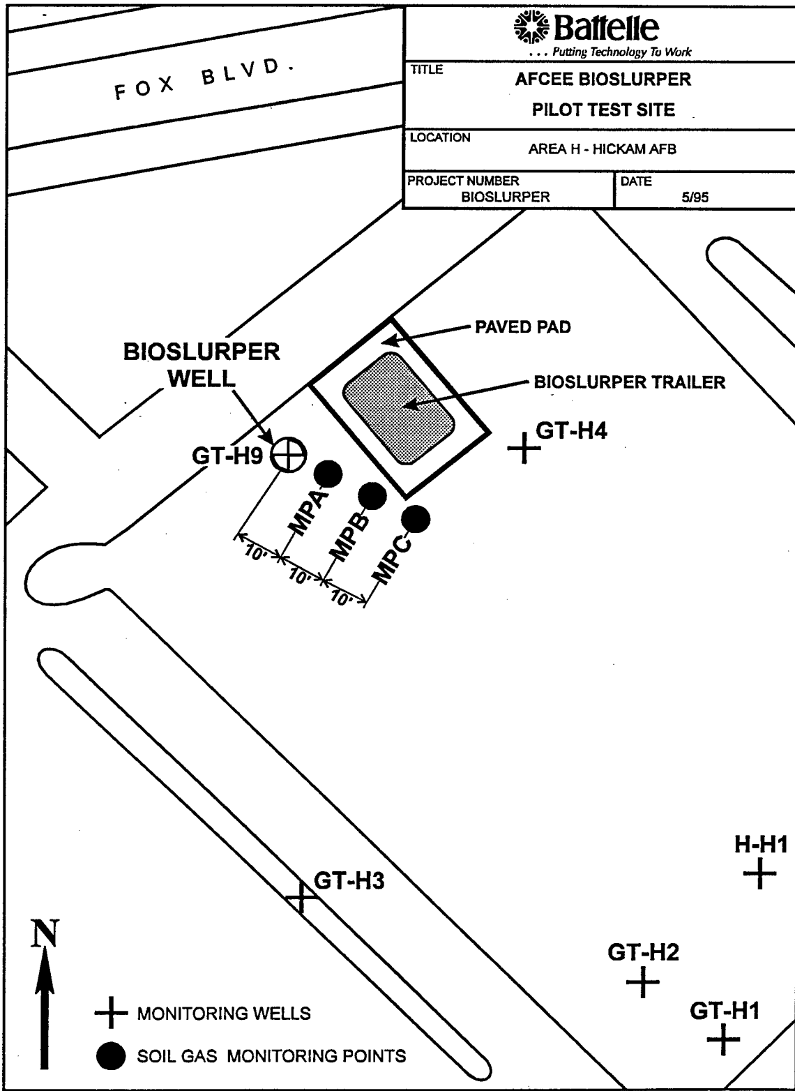
Figure 1. Schematic Diagram Showing Locations of Bioslurper Well, Soil Gas Monitoring Points, and Monitoring Wells at Area H, Hickam AFB, HI
