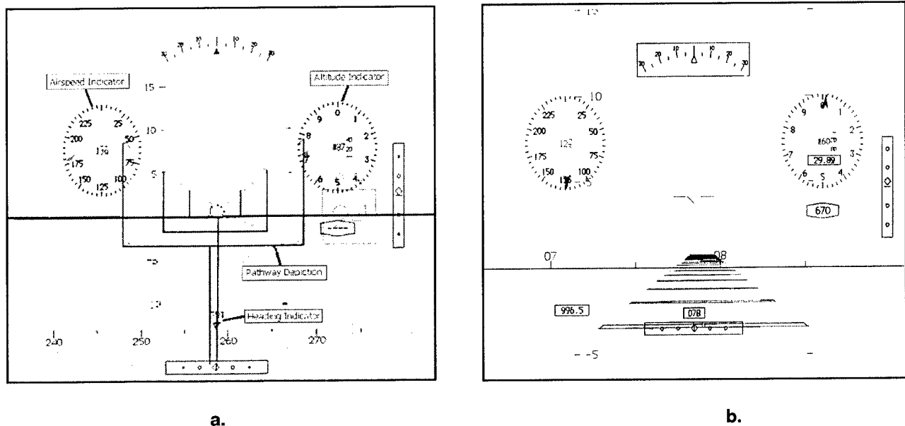
Figure 1. a) Goal post pathway design showing pathway, airspeed, altitude, and heading indications. b) Paving stone pathway design.
