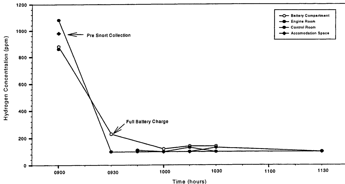
Figure 4. H_2 concentrations: prior to snort; at maximum battery charge; and, two hours after maximum battery charge.
