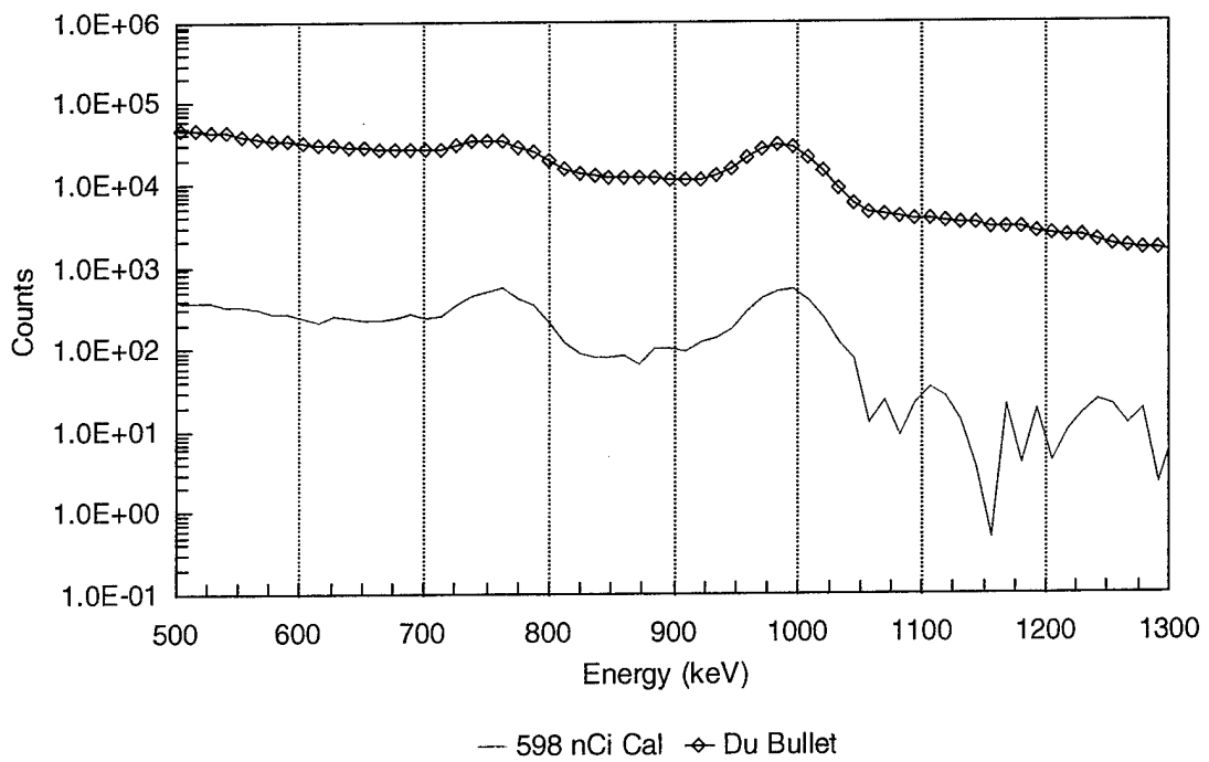
Figure 5: MicroSpec II Energy Spectra
