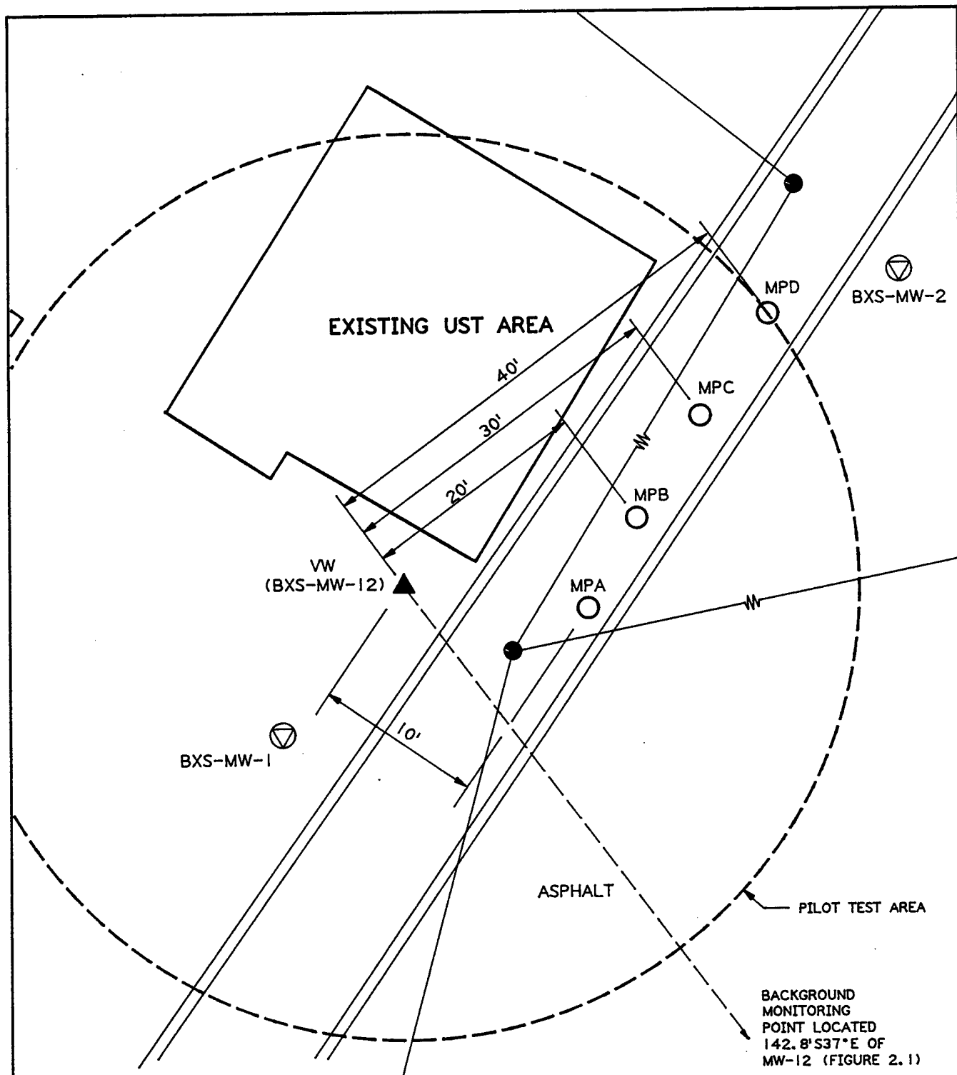
FIGURE 3.1 PROPOSED VENT/MONITORING POINT LOCATIONS BXSS UST AREA VANDENBERG AFB CALIFORNIA ENGINEERING-SCIENCE, INC. Denver, Colorado
