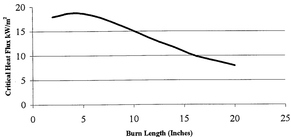
FIGURE 21. INVERSE RELATIONSHIP BETWEEN FLAME PROPAGATION AND CRITICAL RADIANT FLUX
