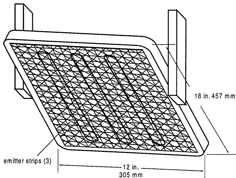
FIGURE A-3a. AIR-PROPANE RADIANT PANEL
