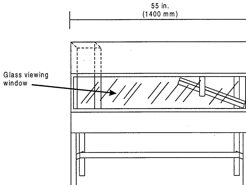
FIGURE A-1. RADIANT PANEL TEST CHAMBER
