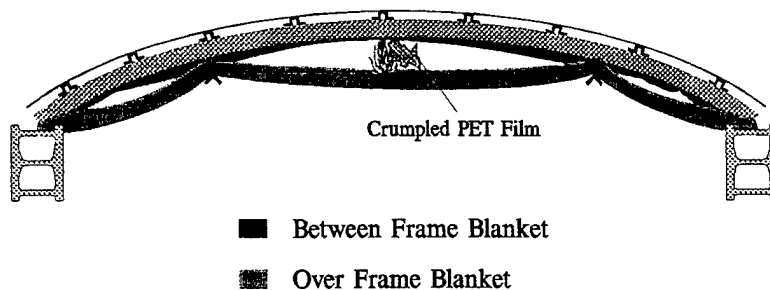
FIGURE 9. INITIAL MOCK-UP TEST CONFIGURATION USING A B747 FUSELAGE SECTION
