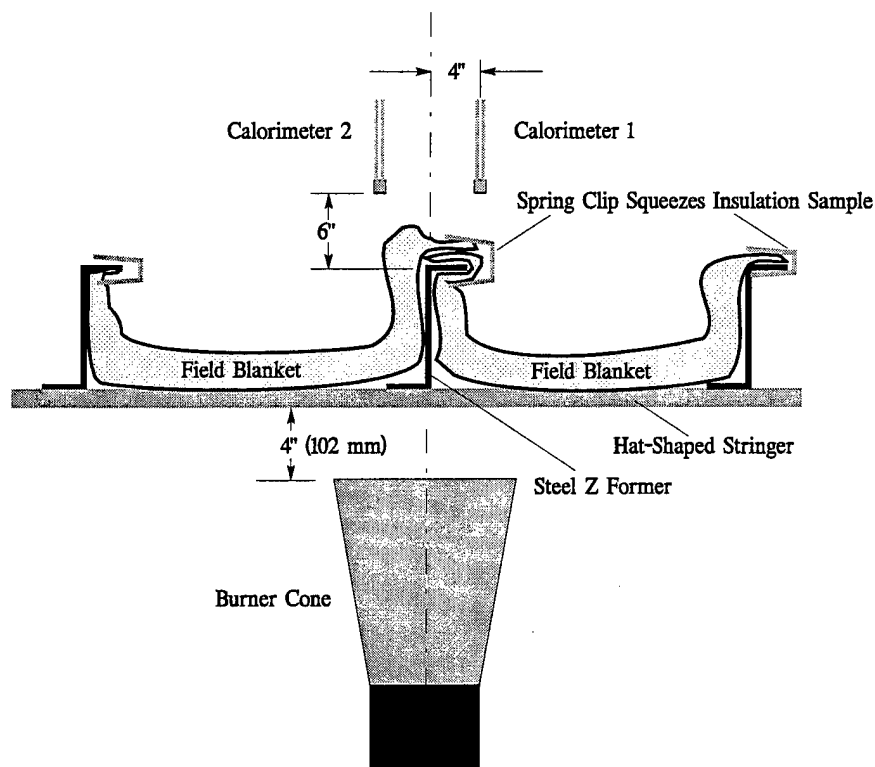
FIGURE B-7. TEST SPECIMEN INSTALLATION ON TEST FRAME
