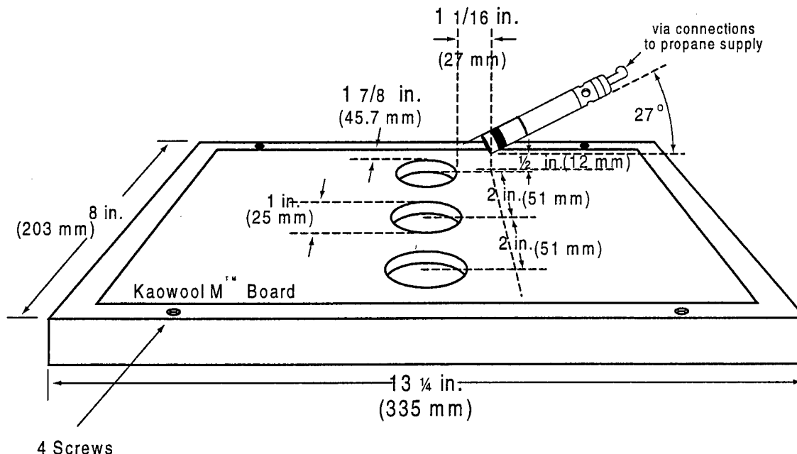
FIGURE A-8. CALORIMETER HOLDING FRAME
