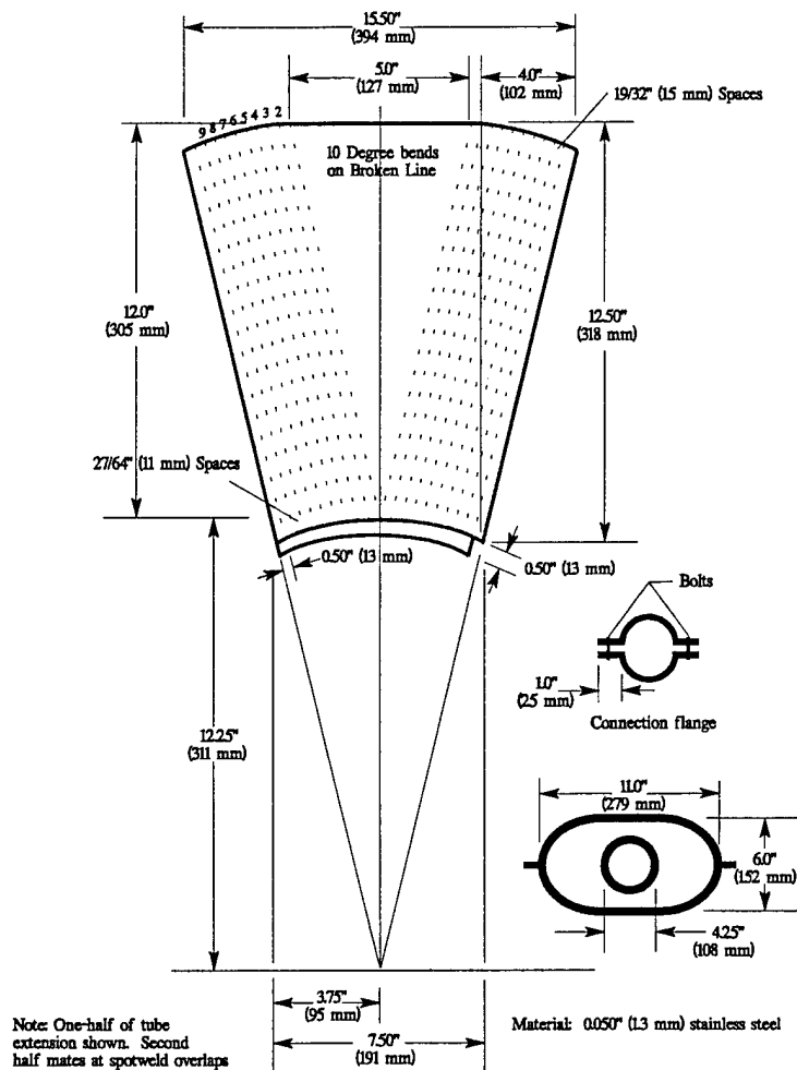
FIGURE B-3. BURNER DRAFT TUBE EXTENSION CONE
