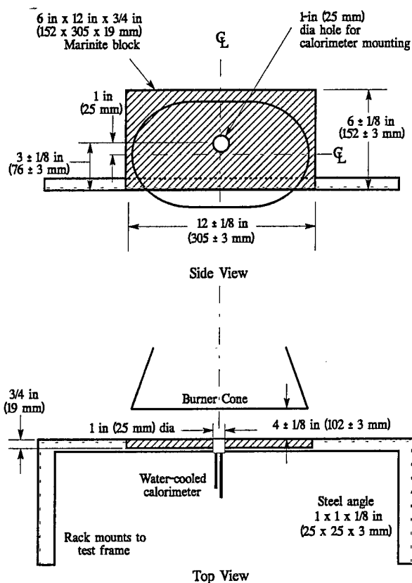
FIGURE B-4. CALORIMETER POSITION RELATIVE TO BURNER CONE
