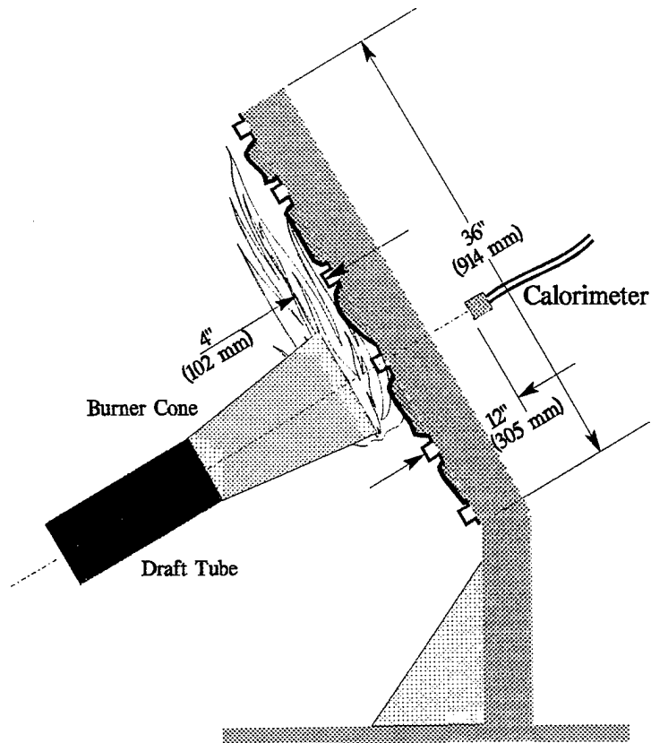
FIGURE B-6. POSITION OF BACKFACE CALORIMETERS RELATIVE TO TEST SPECIMEN FRAME
