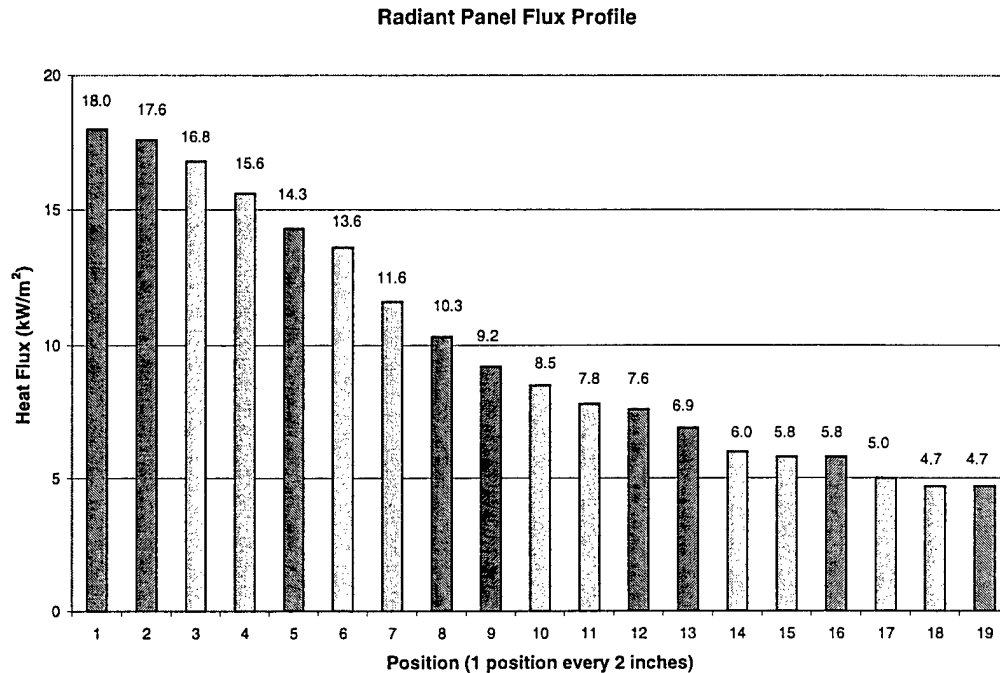
FIGURE 22. RADIANT PANEL FLUX PROFILE
