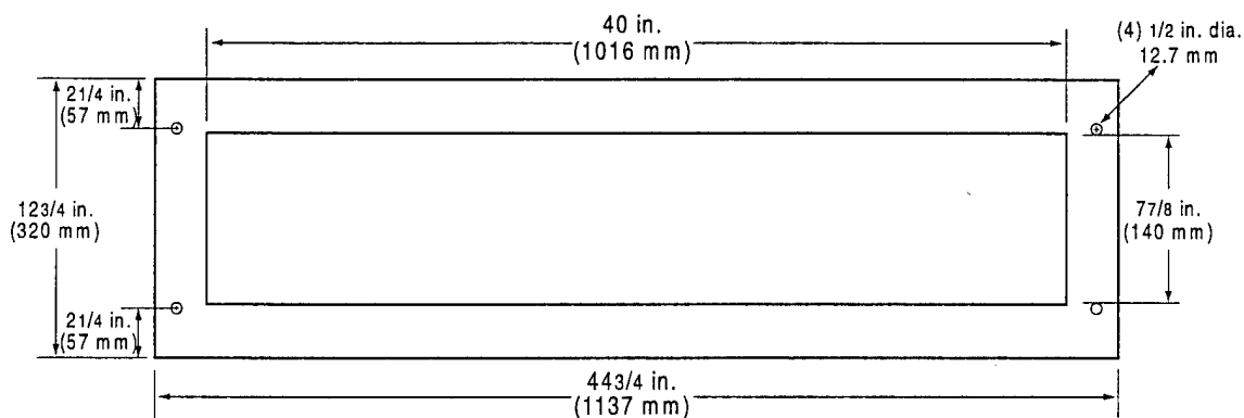
FIGURE A-5. RETAINNG FRAME
