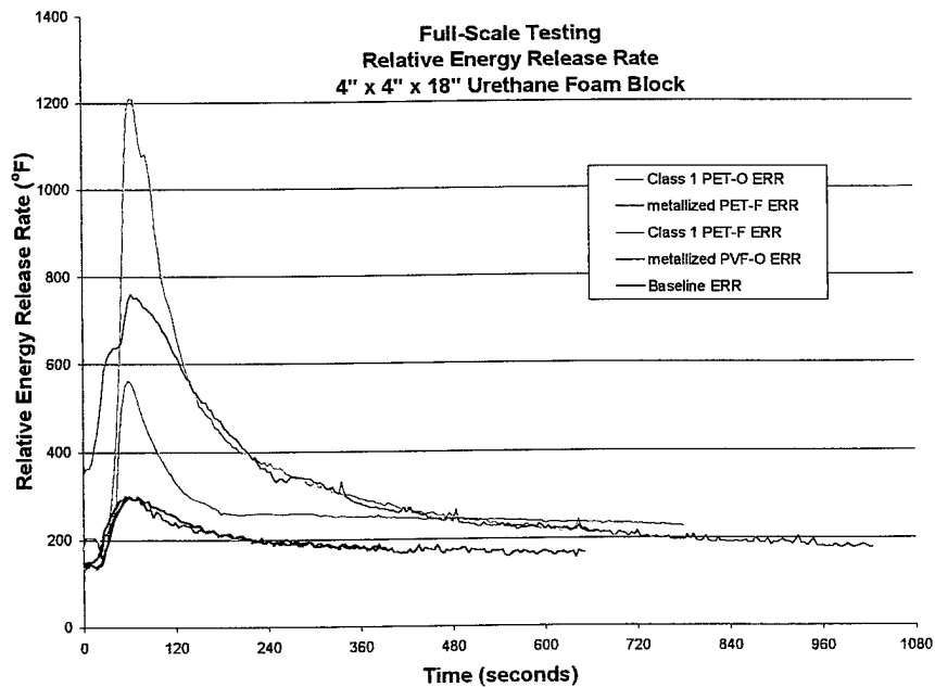
FIGURE 27. ESTIMATED ENERGY RELEASE RATES DURING FULL-SCALE TESTING
