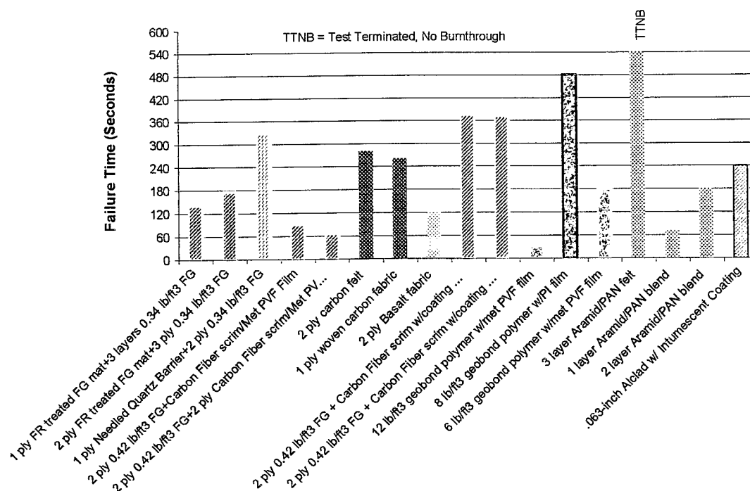
FIGURE 40. BURNTHROUGH TEST COMPARISON USING A 6-GPH BURNER AT 4 INCHES FROM THE TEST RIG
