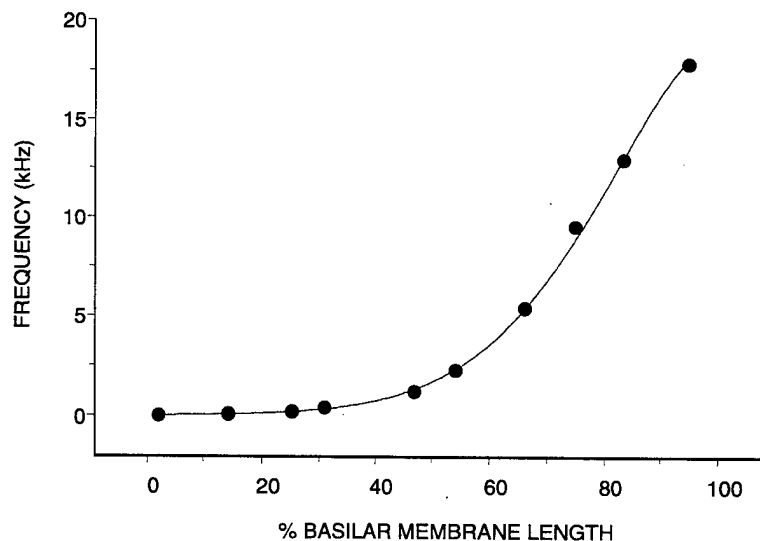
Figure 1. Frequency by relative position along the length of the basilar membrane for the humpback whale. A 3 rd order exponential function was fit to the data ( y = 0.08 * \exp(0.15x - (8.74e-4)x^2 + (1.63e-6)x^3) ) in order to create the frequency-position function.
