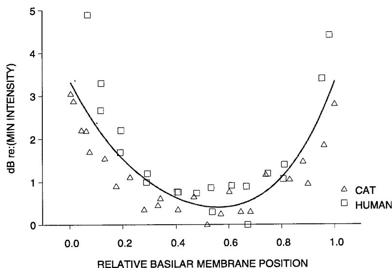
Figure 2. Relative thresholds of the cat and human as a function of relative basilar membrane length. The relationship was determined by integrating experimentally derived frequency-position functions for each species with their respective averaged frequency-dependent thresholds. The fitted function ( y = 3.36 - 12.4*x + 19.72*x^2 - 19.1*x^3 + 11.75*x^4 ) provides a predictive sensitivity-position function.
