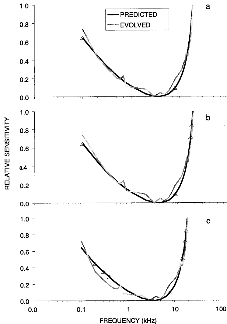
Figure 4. Comparison of the threshold of the three evolved ear models to the predicted threshold of the humpback whale. Triangles indicate frequencies at which maximum deviations between the two sensitivity curves occurred.
