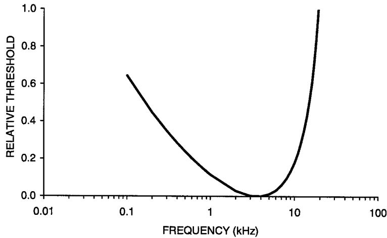
Figure 3. The predicted relative auditory threshold of the humpback whale. The threshold function was determined by integrating the humpback frequency-position function (figure 1) with the sensitivity-position function derived from cat and human audiometric and anatomic data (figure 2).
