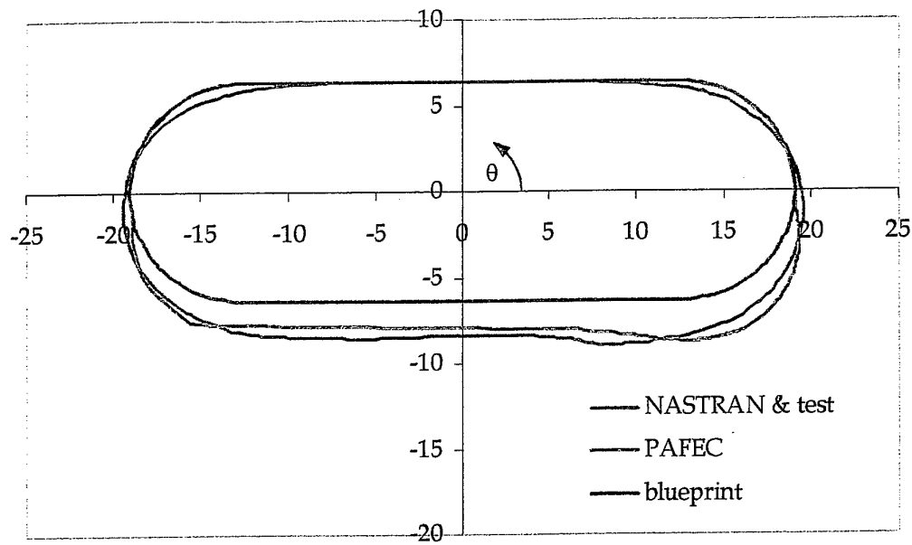
Figure 12: NASTRAN and PAFEC FE model FFWH #13 profiles
