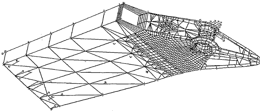
Figure 4b: Maximum applied load (at 7.33g) to full WPF PAFEC FE model
