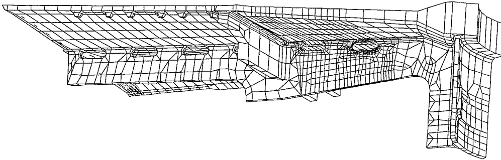
Figure 8: Stiffener #3 finite element mesh detail in NASTRAN model
