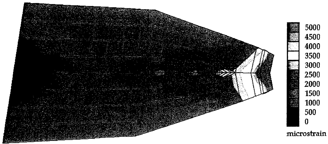
Figure 30: Contour plot of transverse strain ( \epsilon_{zz} ) in upper plate of PAFEC FE model at maximum CPLT load
