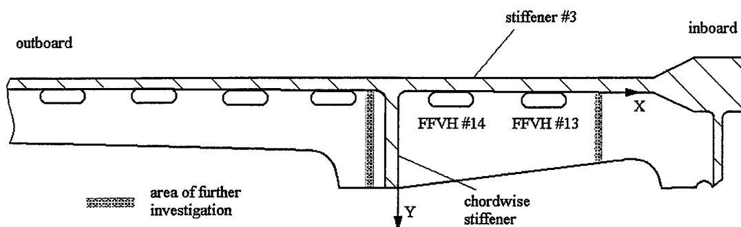
Figure 18: Locations in stiffener #3 for further detailed comparisons
