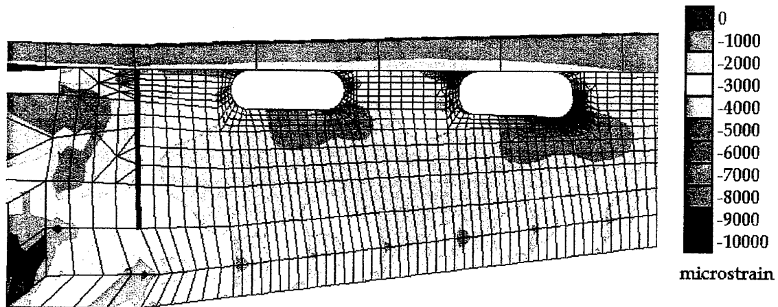
Figure 22: Contour plot of horizontal strain ( \epsilon_{xx} ) in stiffener #3 of PAFEC FE model at maximum CPLT load
