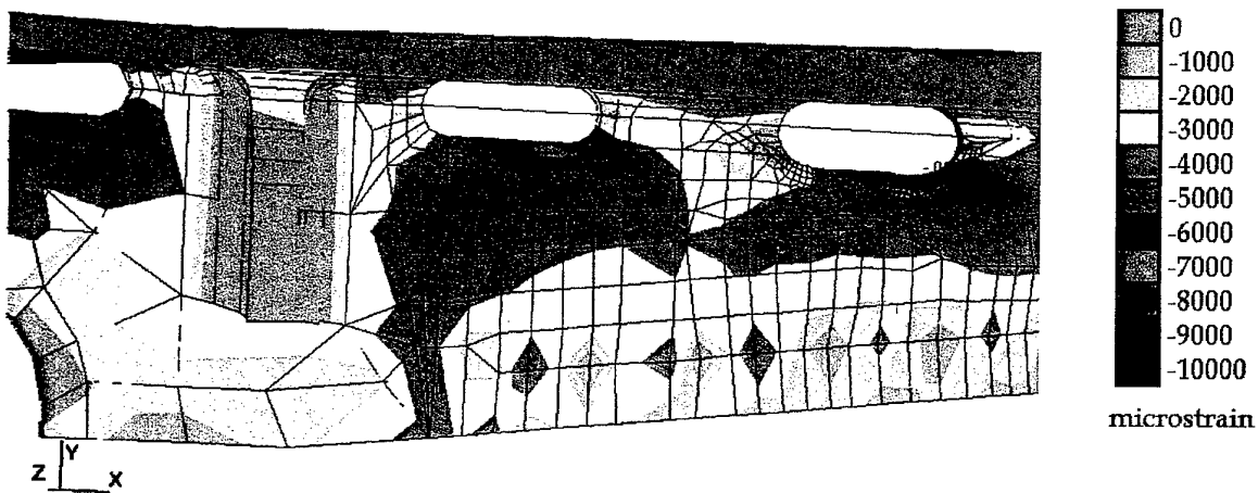
Figure 23: Contour plot of horizontal strain ( \epsilon_{xx} ) in stiffener #3 of NASTRAN FE model at maximum CPLT load
