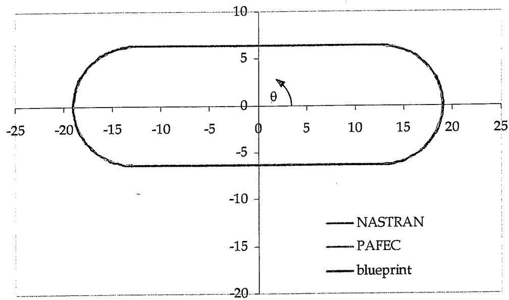
Figure 13: NASTRAN and PAFEC FE model FFWH #14 profiles
