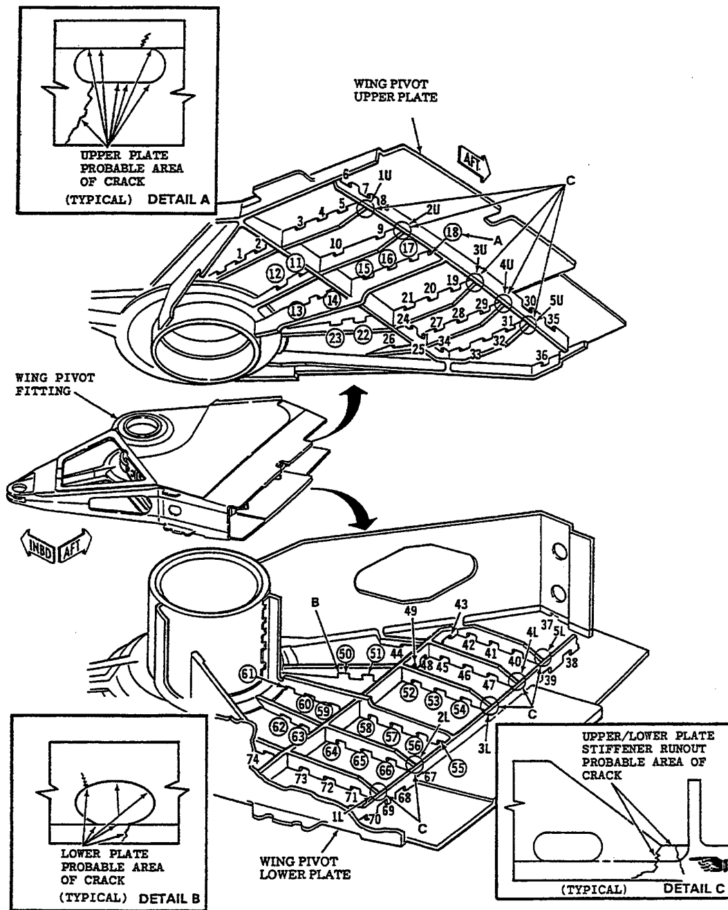
Figure 2: Internal view of the upper plate of the WPF (showing the FFVH locations)
