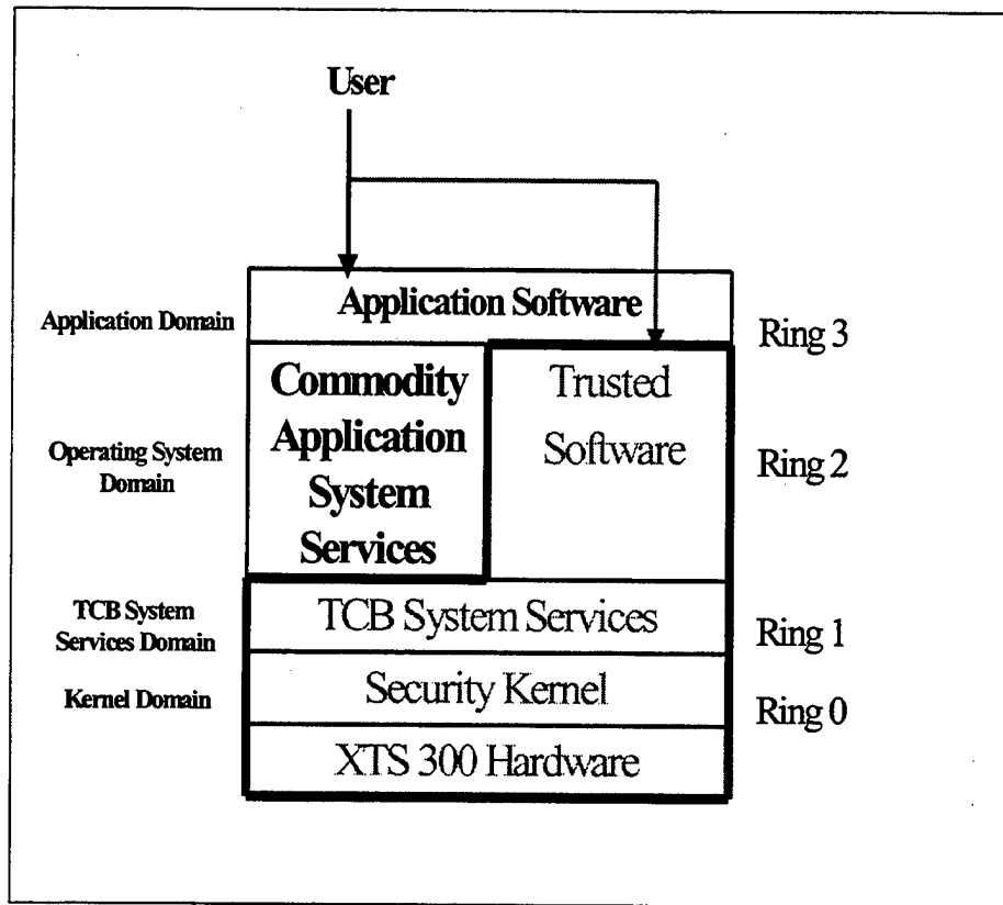
Figure 3. XTS 300 System [9]
