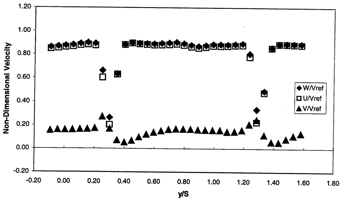
Figure 30. Wake LDV Survey Location 4 - Velocity Ratios
