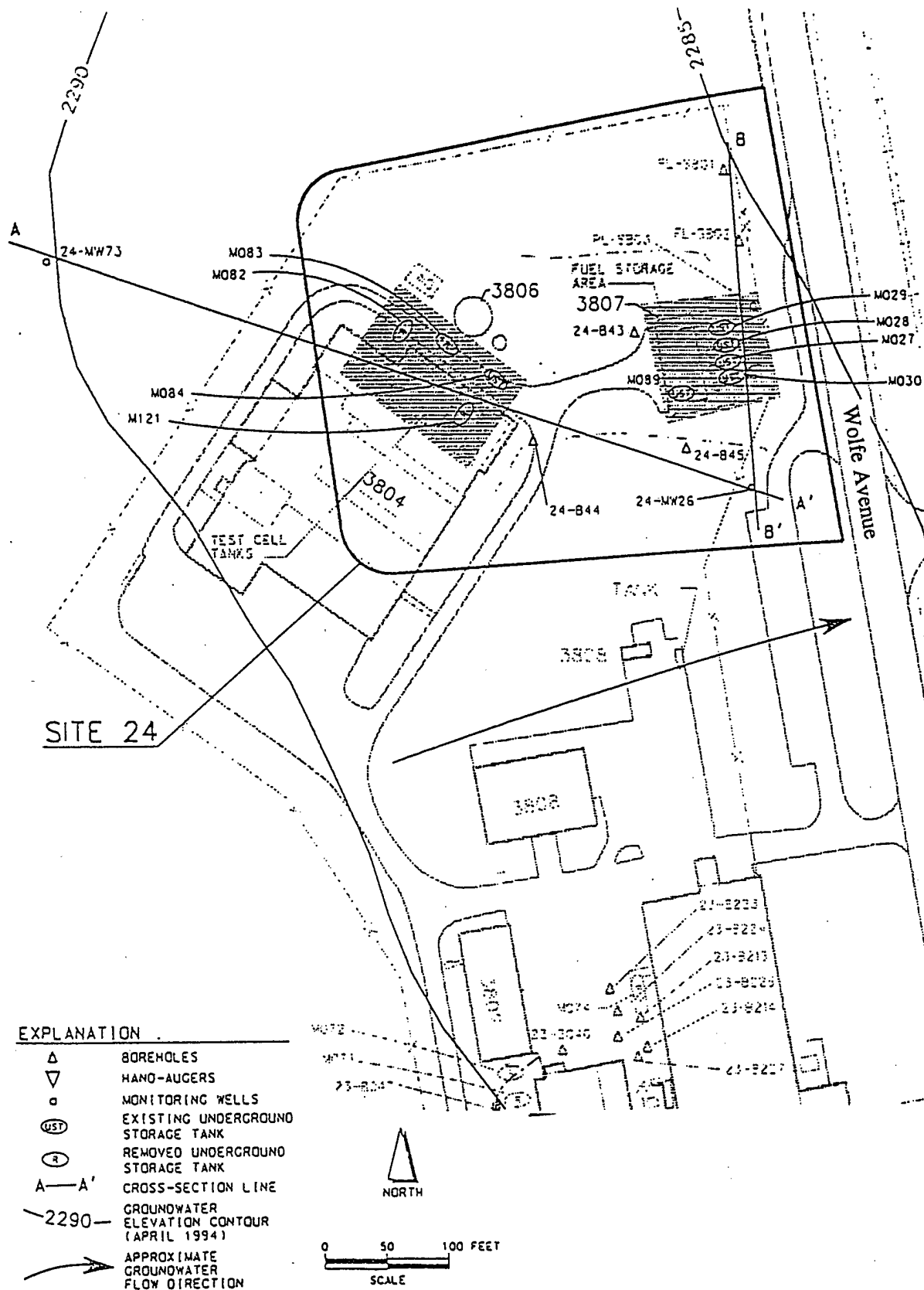
Figure 1. Schematic Diagram Showing Monitoring Well Locations at Site 24, Edwards AFB, California
