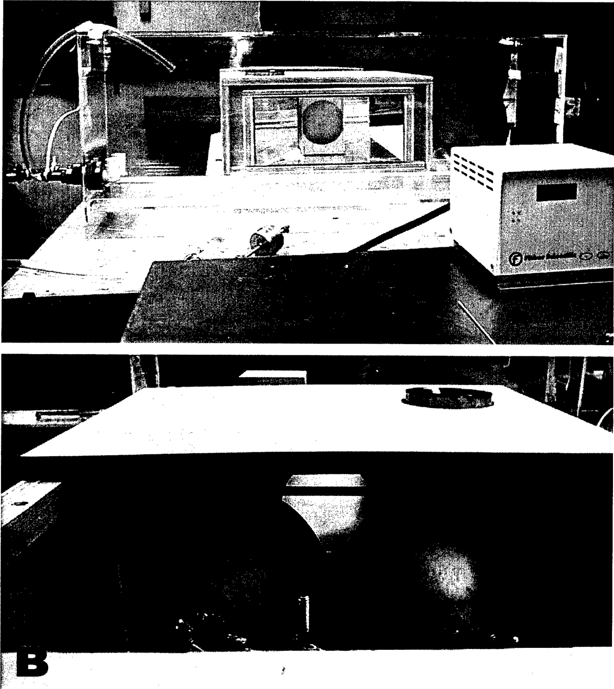
Figure 1. UV-PAR incubator system. (A) Front view: Solar simulator light source with mirrored front and Spectralon diffuser, UV-transparent Plexiglas tank for culture vessels, and water temperature control bath. (B) Internal view: Solar simulator light source with top removed showing PAR (tungsten/halogen) and UV (xenon) lamps with elliptical reflectors aimed at Spectralon diffuser.
