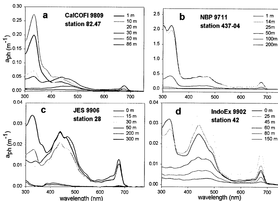
Figure 4. Spectral absorption coefficients from 300-750nm at six depths for stations in (a) California Current, (b) Ross Sea, (c) Japan East Sea, and (d) Indian Ocean. A peak in the UV range around 325nm that decreases with increasing depth is evident at all four stations.
