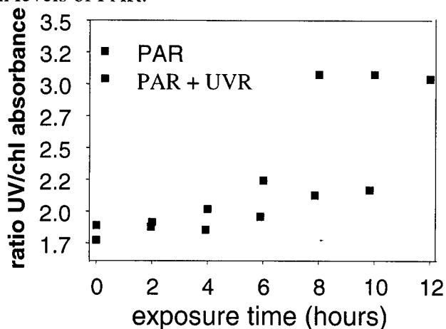
Figure 3. Chlorophyll specific UV-absorbance for Alexandrium tamarens exposed to PAR only or PAR-UVR.
