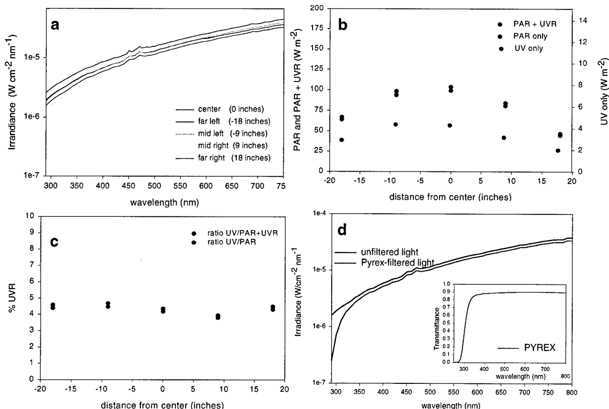
Figure 2. (a) Spectral shape measured at 5 locations along the front of the UV/PAR simulator (distance from center indicated in parentheses). (b) Flux of PAR + UVR, PAR only, and UV only at the five locations indicated in (a) (*Note different scale for UV-only values). (c) Ratio of UV to total (UV+PAR) and PAR-only at the same five locations in parts (a) and (b). (d) Spectral distribution of the incubator illumination (red) and the convolution with Pyrex culture vessel transmittance (blue). Experimental cultures are grown in Pyrex vessels to exclude short wavelength UVB flux to achieve a spectrum that is similar to natural fluxes in the environment.
