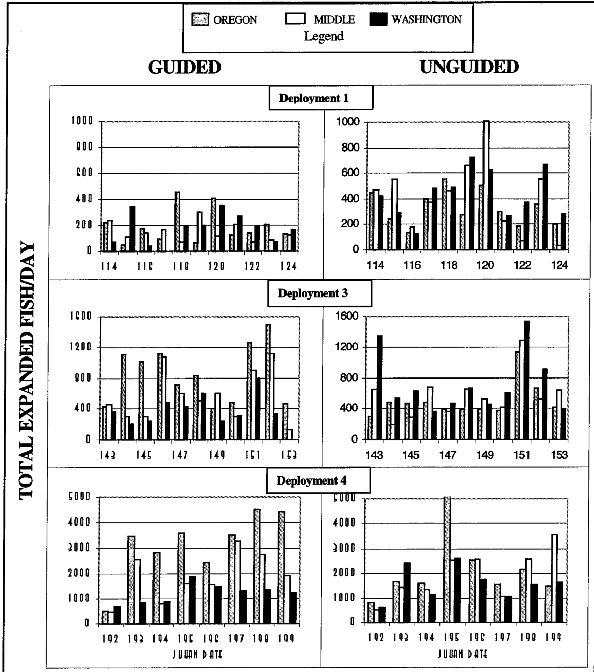
Figure 8. Horizontal distribution of fish across opening for Intake 8b as detected by the single-beam transducers. The intake was divided laterally into thirds: the Oregon side, the middle, and the Washington side.
