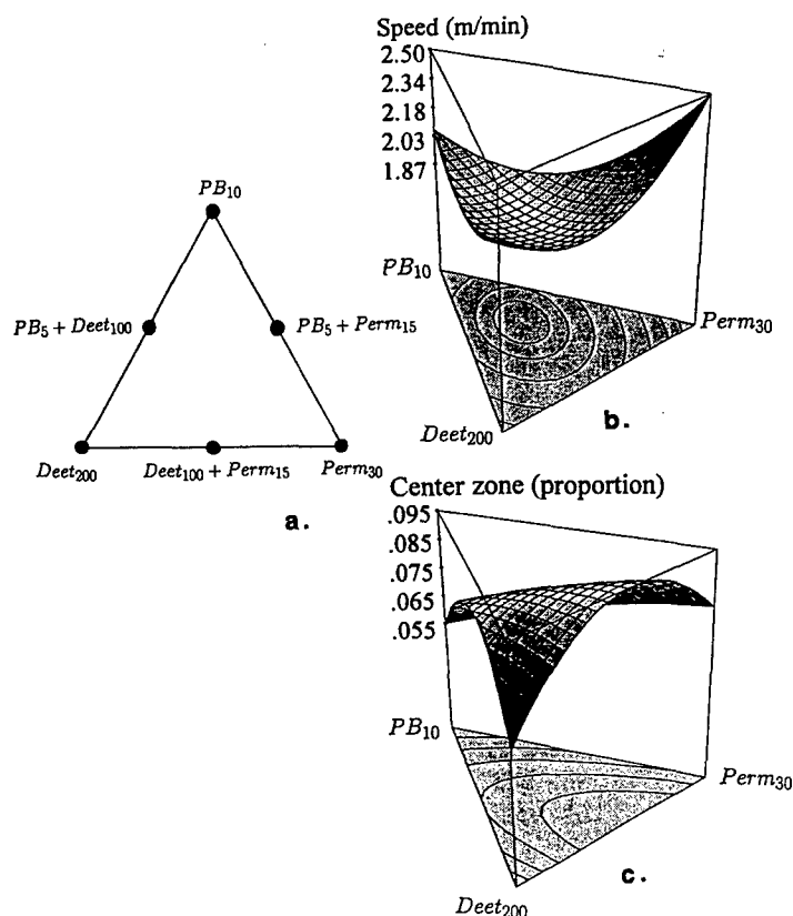
Figure 1. The 3-drug simplex and resultant isobolograms, illustrating a) the drug combinations, b) the isoblogram for male speeds, and c) the isoblogram for male center zone times.
