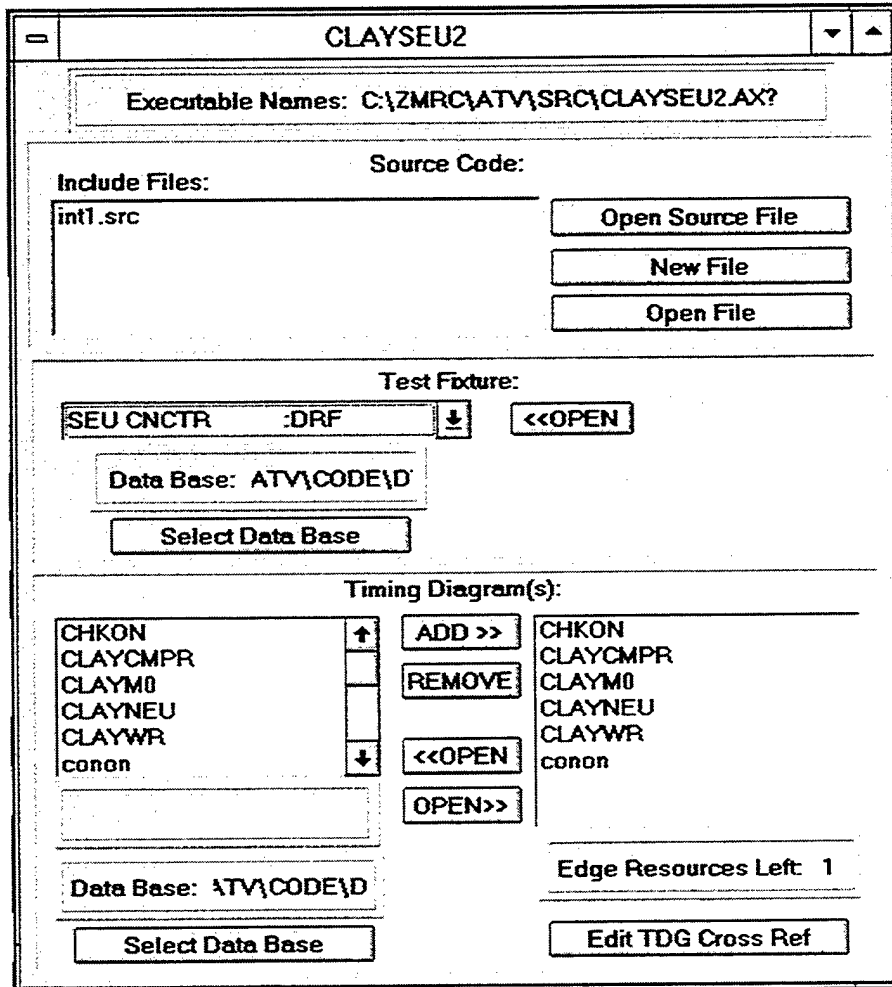
Figure 5-6. Algorithm project dialog box.
