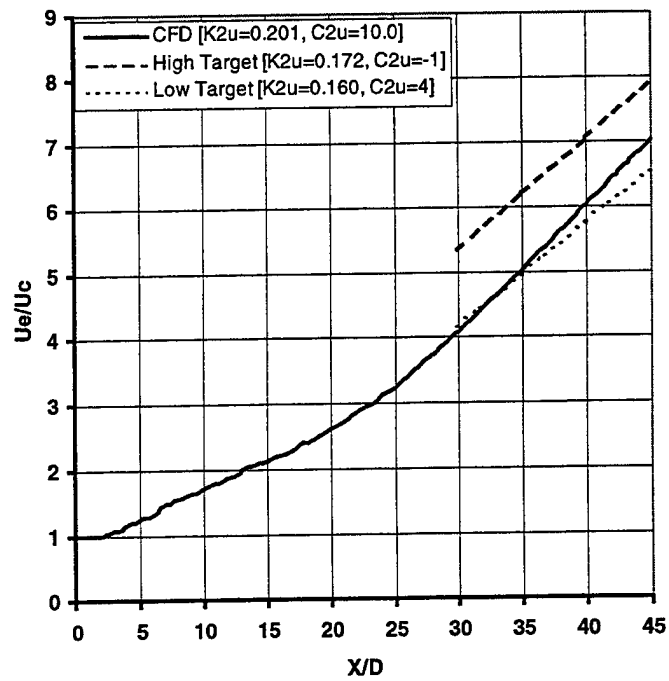
Figure 9. Round Jet Centerline Velocity Decay
