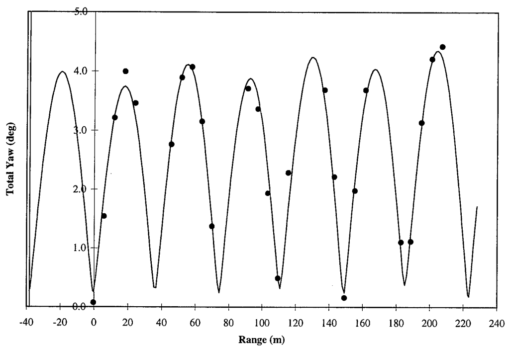
Figure 20. Total Yaw Versus Range, Shot 4.
