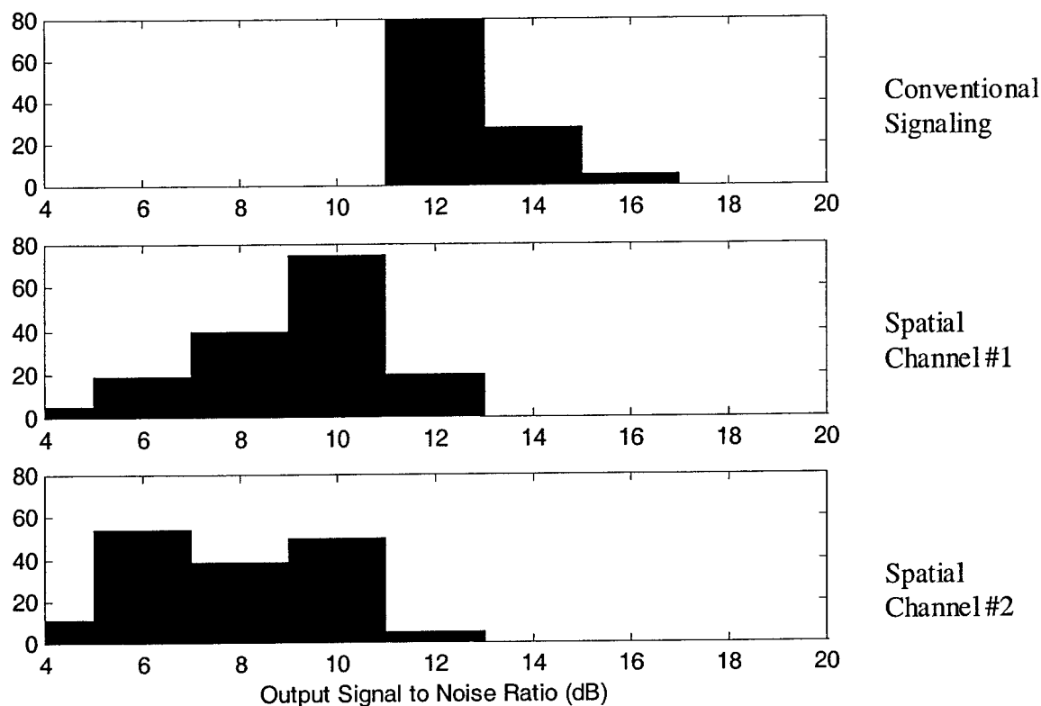
Figure 4.17. The output SNR for each of the 140 packets of Type 1 (a sub-arraying packet) transmitted during SM99 at site 1 is summarized here as a histogram. The single, spatial channel achieved an average SNR of 12 dB while each of the two spatially modulated channels achieved an average SNR of 8-9 dB
