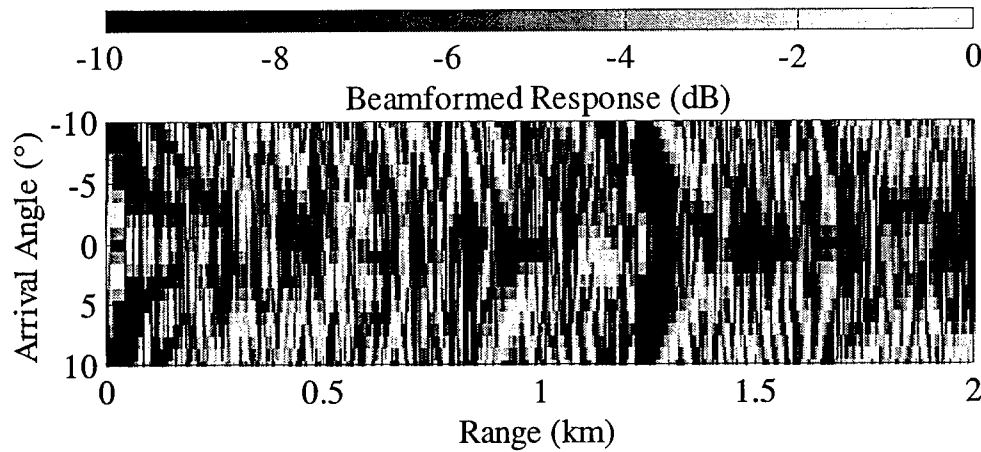
Figure 2.16. The result of applying a beamforming plane wave match filter to the first left singular vector of the decomposition (described in example 4) is shown here as a function of receiver range. The angular spread suggests that multiple rays are energized.
