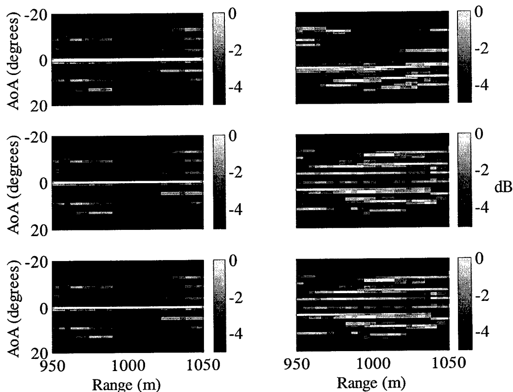
Figure 2.22. The receive array responses that result from an ensemble decomposition of the shallow ocean example are shown here transformed into angle space using a plane wave match filter. The left panels result from the first steering vector while the right panels result from the second. The top panels use measure 2, the middle panels use measure 3, and the bottom panels use measure 4.
