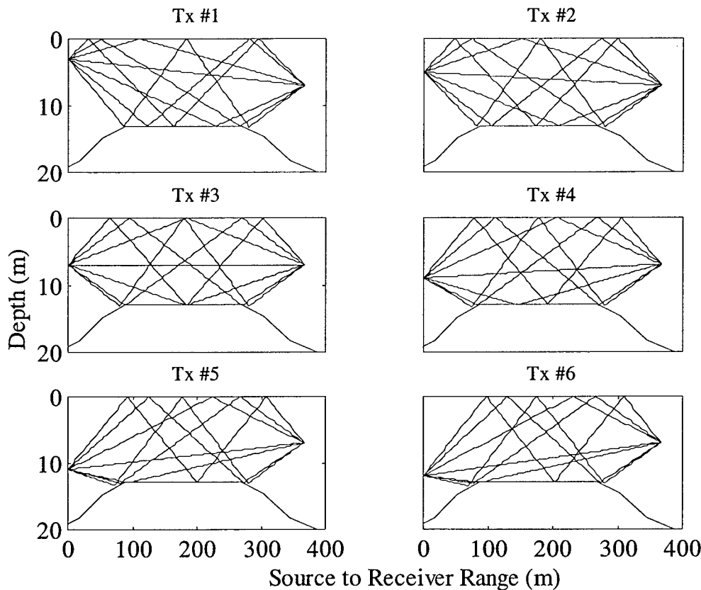
Figure 3.12. Using a uniform sound velocity profile in the SM00 experiment, a ray model was used to discern the propagation paths from each transducer to the receiver array. A direct arrival is evident for all transducers while off angle arrivals range from 1-4 degrees for upward arriving rays (positive angle) and 3-7 degrees for downward arriving rays (negative angle).
