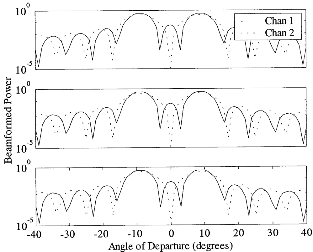
Figure 2.18. The steering vectors that result from an ensemble decomposition of the two eigenray example with random time-of-arrival are shown here transformed into angle space using a plane wave match filter, i.e. a beampattern. The top panel uses measure 2, the middle panel uses measure 3, and the bottom panel uses measure 4 (see text for definition of measures). The ensemble decomposition is not sensitive to relative phase of the eigenrays.
