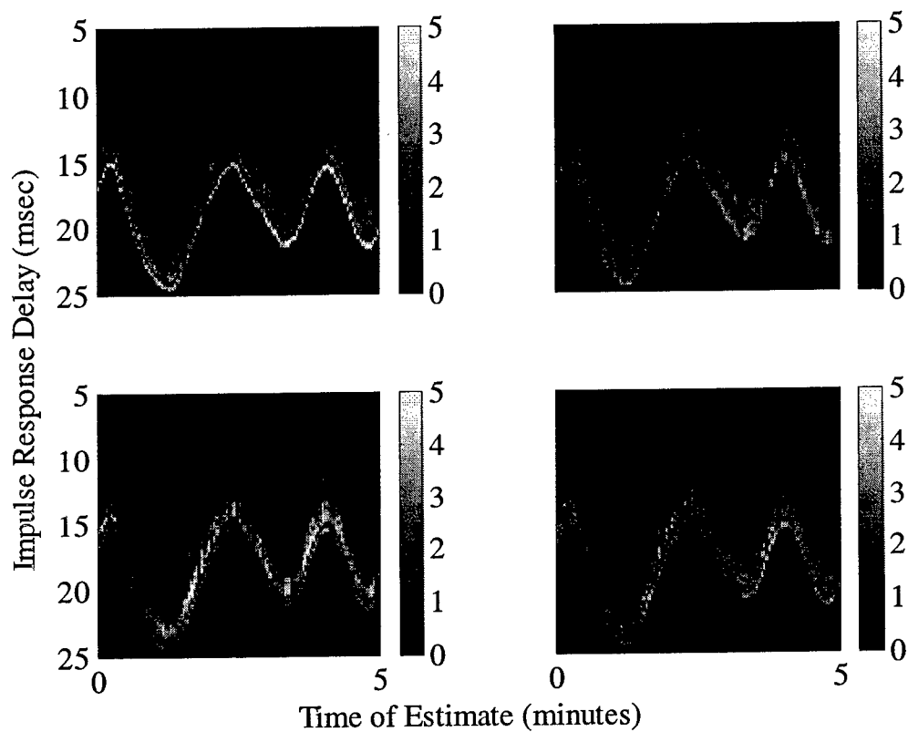
Figure 4.13. The combination of wind and current forcing on the R/V Mytilus conspired to generate a substantial, periodic oscillation at anchor that manifested itself in a wander of the arrival time. The dimensions are normalized amplitude. Clockwise from the top left panel, the impulse responses are for transmitter 1 to receiver 1, transmitter 1 to receiver 14, transmitter 6 to receiver 1, and transmitter 6 to receiver 14.
