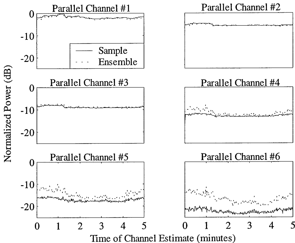
Figure 3.3. The normalized power transfer efficiency of the six parallel channels is shown here for each SM00 channel impulse response estimate (March 6) over a 5 minute observation interval at 1 second intervals. The curves labeled sample result from exciting the channel with the appropriate right singular vector of that sample's impulse response while the curves labeled ensemble result from using the fixed right singular vector of the channel ensemble, of \mathbf{T}^H(f)\mathbf{T}(f) . Each sample channel's power has a standard deviation ranging from 0.4 to 0.6 dB while the mean falls off linearly by about 4 dB per channel.
