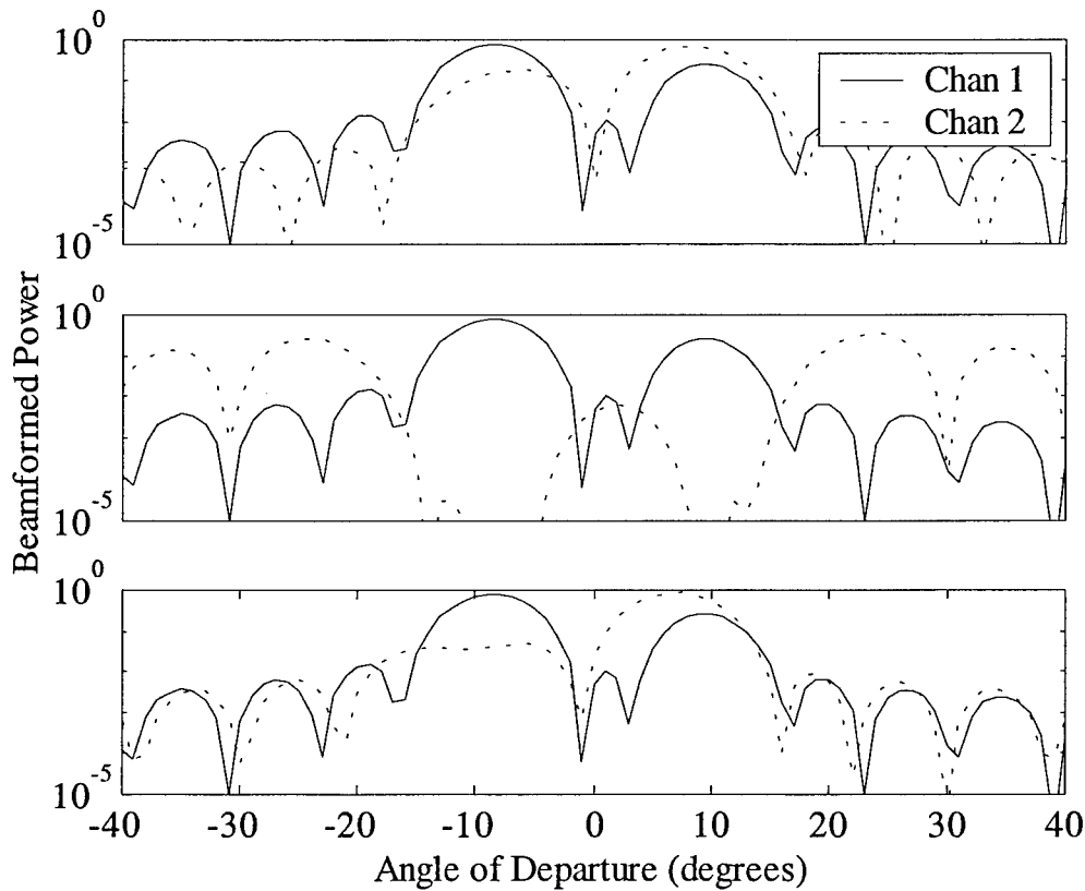
Figure 2.20. The steering vectors that result from an ensemble decomposition of the two eigenray example with wavenumber spread are shown here transformed into angle space using a plane wave match filter. The top panel uses measure 2, the middle panel uses measure 3, and the bottom panel uses measure 4 (see text for definition of measures).
