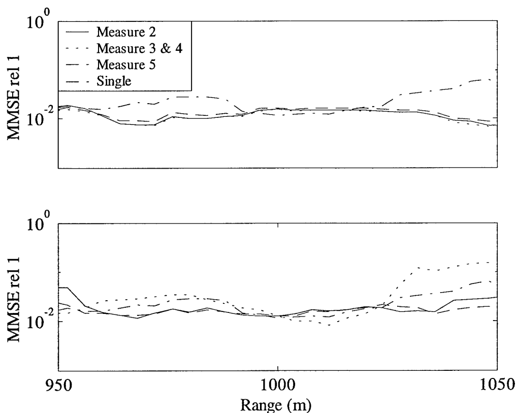
Figure 2.23. The mean square error (MSE) that results from using an ensemble decomposition of the shallow ocean example is shown for the various possible steering vectors. The MSE is relative to a signal power of 1. Measures 2, 3, 4, and 5 are as defined in the text. Measures 3 and 4 gave nearly identical results and are shown with a single curve. The curve labeled single refers to the use of steering vector derived from the single channel realization at 1000 m. The top panel is for the first parallel channel while the bottom panel is for the second
