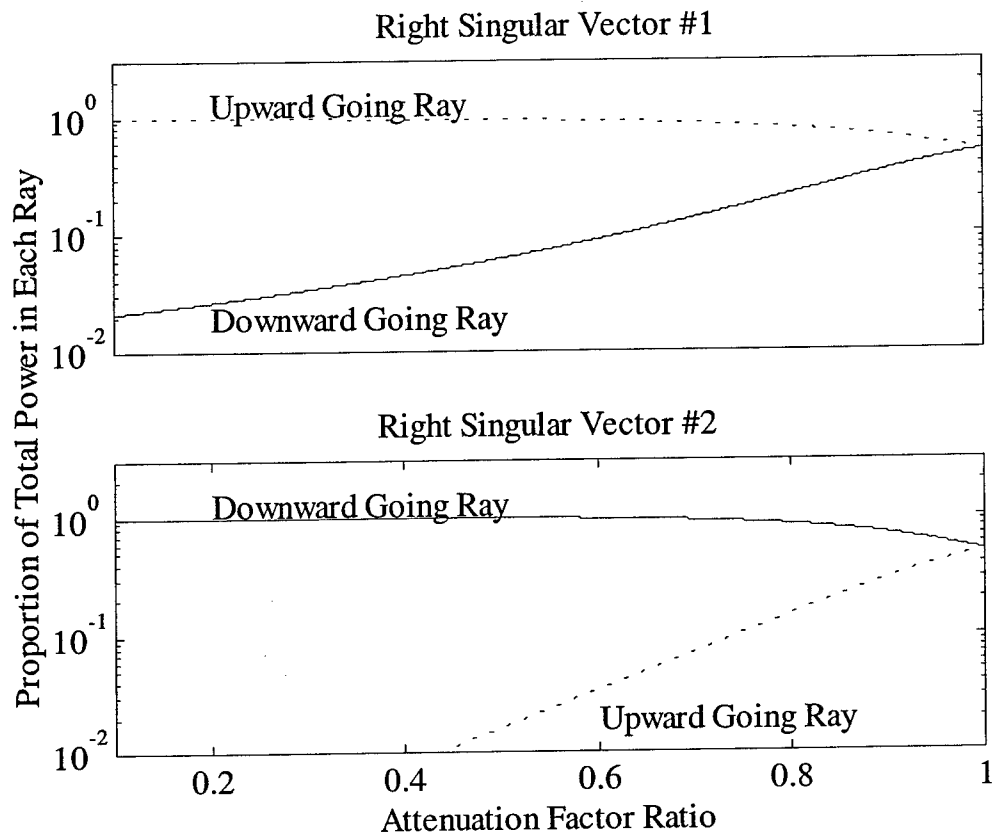
Figure 2.13. The behavior of the singular vectors is examined here as a function of the attenuation factor ratio between the two ray paths. For various ratios, the apportionment of power between the upward and downward going rays by the first right singular vector (upper panel) and the second right singular vector (lower panel) are shown. For equal attenuation factors (ratio = 1), each ray gets half of the power associated with the singular vector. For ratios less than \frac{1}{2} , the singular vectors essentially restrict themselves to a single ray.
