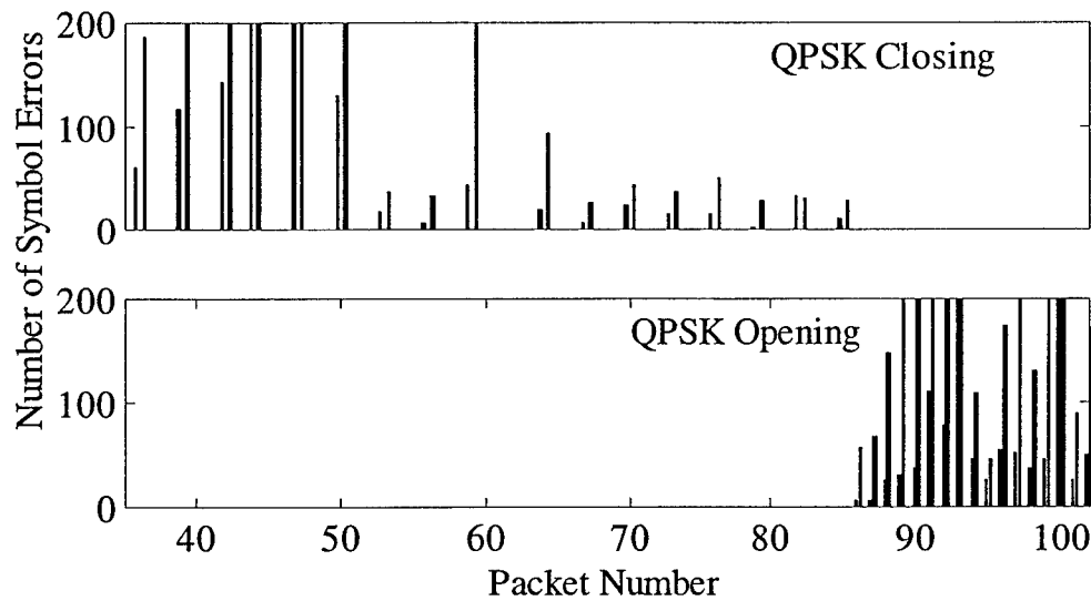
Figure 4.8. Symbol error rates for the closing and opening QPSK transmissions both with and without the superposition of the other QPSK signal. For each pair of bars, the left bar is the single signal case while the right bar is the two signal case. In most cases, the number of errors approximately doubles but decodable packets remain decodable thereby showing the successful use of two parallel channels. The performance degradation is almost entirely due to the 3 dB noise enhancement caused by the superposition of data sets.
