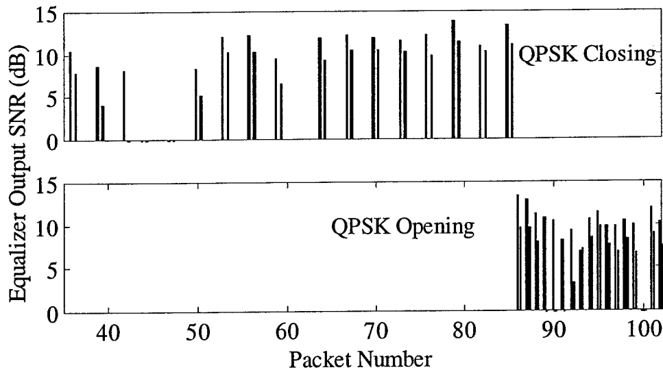
Figure 4.9. Synthesizing a three platform architecture by superposition of two data sets results in an artificial decrease of SNR by 3 dB. For each pair of bars, the left bar is the single signal case while the right bar is the two signal case. The above panels show the SNR of the symbol estimate from the equalizer for each leg when the other leg is superimposed. Note that the SNR decreases approximately 3 dB in all cases.
