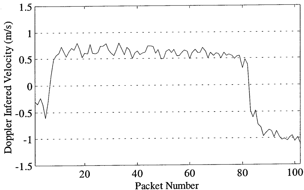
Figure 4.5.. Estimated line of sight velocity between transmitter and receiver based on frequency shift of the response peak in the ambiguity function for the training sequence of each packet. The shift from closing in range to opening in range is seen immediately after packet 80 in conjunction with a near doubling of speed. For reference, 1 knot is approximately 0.5 m/sec.
