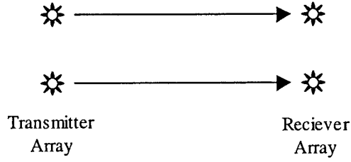
Figure 2.7. The double duct scenario is shown here where each transducers only couples to a unique hydrophone. The lines represent eigenray paths
