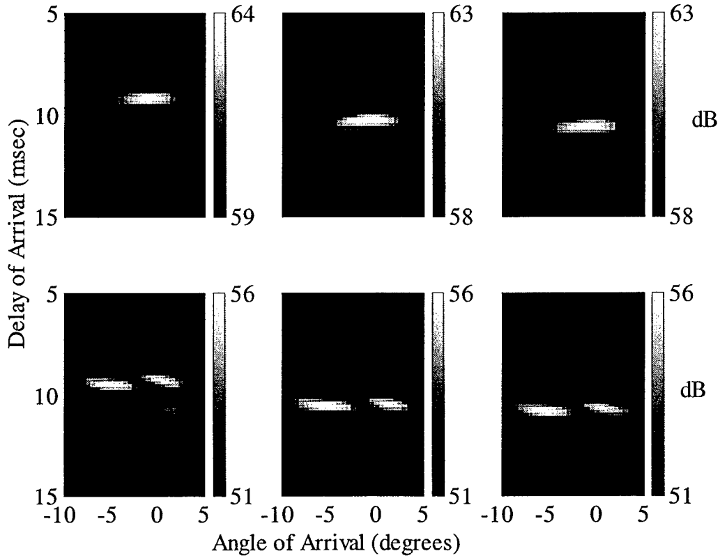
Figure 3.14. The scattering function in a delay-of-arrival versus angle-of-arrival space is shown for three channel realizations in the SM00 (March 6) experiment. The top three panels show the response due to the first singular vector of an SVD for the channel ensemble while the bottom three panels show the response due to the second singular vector. From left to right, the panels give the responses using three different channel measurements.
