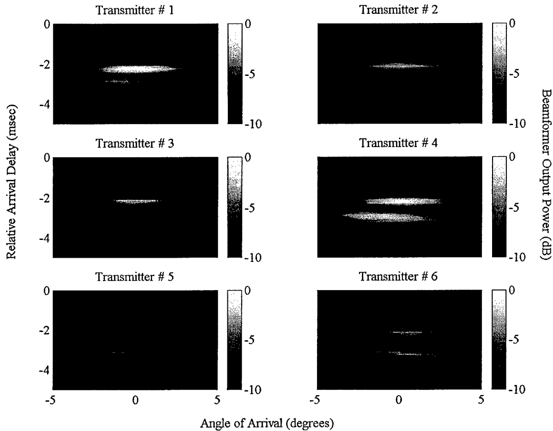
Figure 4.19 Using the measured impulse responses between transducer / hydrophone pairings, the relative power transferred by each transducer is shown in a delay of arrival versus angle of arrival space. Note the dominance of transducers 1 and 4 and their unique spatial structure.
