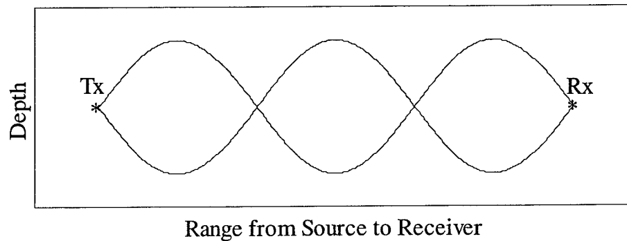
Figure 1.2. A simplified model of convergence zone propagation in the ocean is shown here. The existence of a sound velocity minimum causes energy leaving the transmitter to diffract into the “eye pattern” shown here. At specific locations, the existence of two, spatially distinct propagation paths that connect the source (Tx) and receiver (Rx) is evident.
