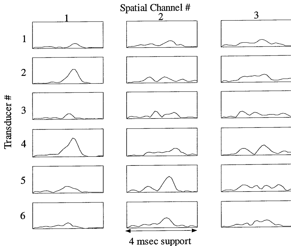
Figure 4.20. The magnitude of the broadband filters applied to each of the six transducers to create each of the three spatial channels is shown above. The magnitude is shown on a linear scale ranging from 0 to 0.5. The temporal support of the filters is approximately 4 msec (15 symbols). These filters were derived from measurements made on Day 3 of SM00 and used on Day 4.
