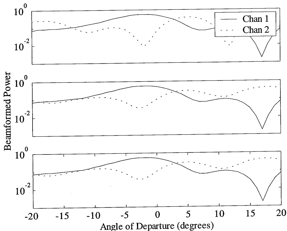
Figure 2.21. The steering vectors that result from an ensemble decomposition of the shallow ocean example are shown here transformed into angle space using a plane wave match filter. The realizations are different ranges between 950 m and 1050 m. The top panel uses measure 2, the middle panel uses measure 3, and the bottom panel uses measure 4 (see text for definition of measures). Note the peaks and nulls at -3 , 12 , and 17 degrees.
