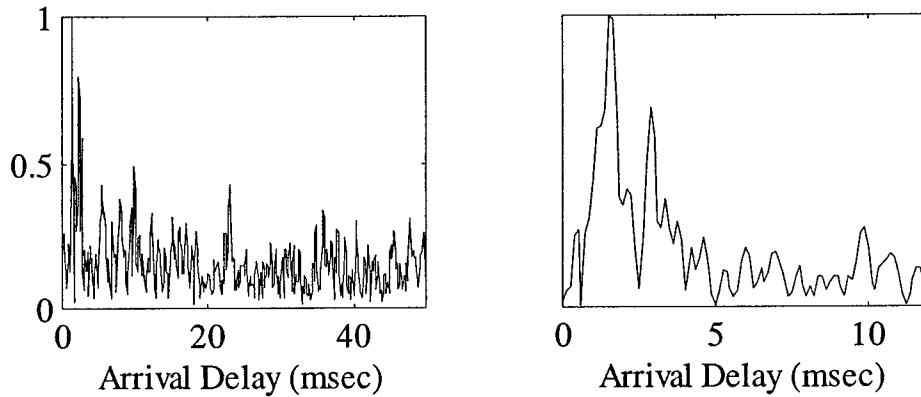
Figure 3.1. Typical impulse responses for the SM99 experiment (left panel) and the SM00 experiment (right panel) are shown here. The lower processing gain of the SM99 channel probe is evidenced by the pronounced noise. The shorter range of the SM00 experiment is likewise evidenced by the shorter total delay spreads.
