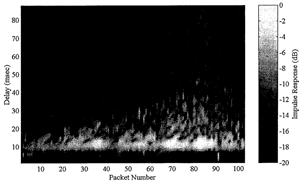
Figure 4.6. The impulse response evolution over the course of the experiment is shown here. Much of the energy is consistently within a delay spread of several symbols. The growing length of the reverberation tails is due to the decreased range and, therefore, decreased attenuation of the high angle rays that have multiple surface reflections. The range decreases linearly from 1 km initially to 100 m at packet 85 and opens to 500 m at packet 103.
