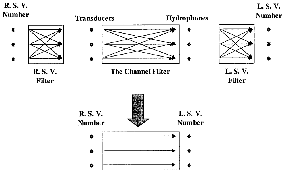
Figure 2.6. If the physical, time-varying channel varies “slowly enough” compared to the total delay spread it induces, the SVD analysis will yield a set of pre- and post- processing filters (the right and left singular vectors, R.S.V.’s and L.S.V.’s) that transform the physical channel into a set of parallel channels, each of which may be frequency selective.
