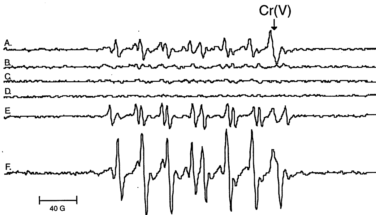
Fig. 8. ESR spectra obtained during the NADPH-dependent Cr(VI) reduction at 37°C by proteoliposomes under room air in the presence of DEPMPPO (50 mM). A: Proteoliposomes containing b_5 + P450 reductase, 400 \mu M Cr(VI), and the NADPH-generating mix. B: Same as A, minus NADP + . C: Same as A, minus Cr(VI). D: Same as A, except with catalase (5200 U). E: Same as A, except with ammonium formate (250 mM). F: Same as A, except with H 2 O 2 (400 \mu M). Similar spectra were obtained when substituting human microsomes for proteoliposomes (not shown). For all, the total volume was 0.2 ml in K 2 HPO 4 (pH 7.35)/ 3 mM MgCl 2 /0.35 M KCl. The reactions were immediately transferred to a quartz mini-flat cell and placed in the ESR cavity. Spectra were recorded every 1.5 min; the spectrometer settings were: field set = 3210 G, sweep width = 200 G, time constant = 0.128 s, scan time = 1 min, modulation amplitude = 1 G, modulation frequency = 100 KHz, receiver gain = 2X10 4 , microwave frequency = 9.023 GHz, and microwave power = 20 mW.
