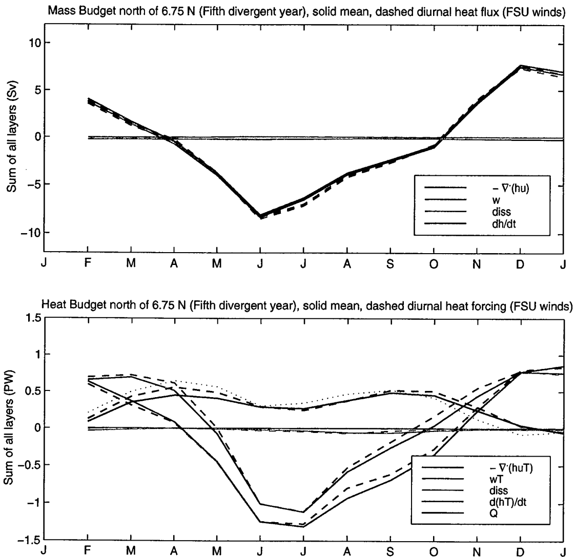
Figure 3.26 Monthly mean terms in the mass and heat budgets of the model, summer over all layers and over the area of the Arabian Sea north of 6.75^{\circ}\text{N} , from the last year of integration. Solid lines are run F, dashed run FD. For comparison, the dotted black line in the heat budget is the SOC climatology integrated over the Arabian Sea.
