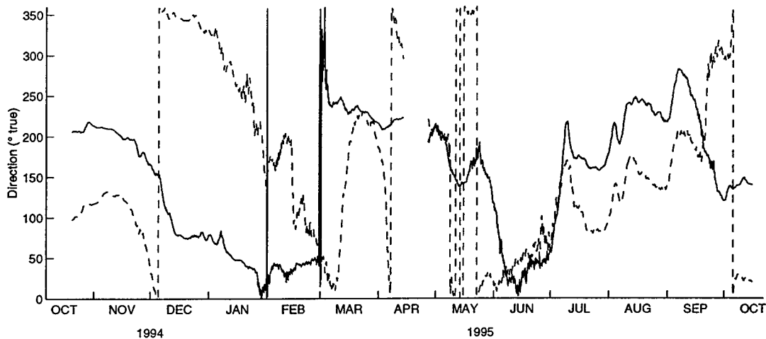
Figure 2.8 Direction of the temperature gradient ( solid ) and velocity ( dashed ) calculated from 48-hour lowpass filtered data at 80 m. During times of strong current the relationship between the two is very close to geostrophic.
