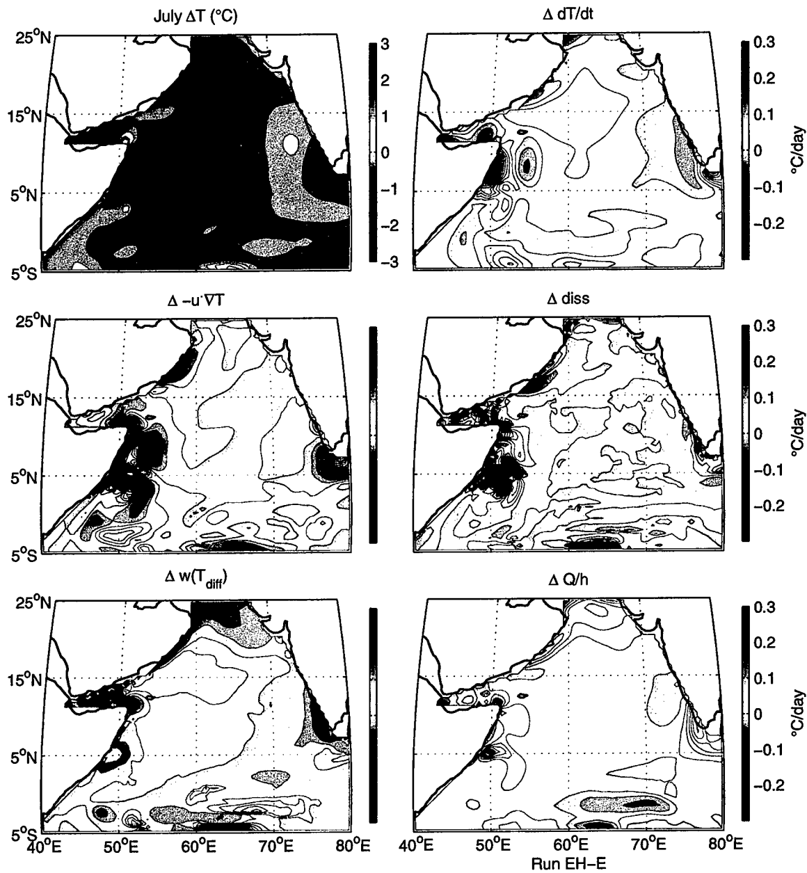
Figure 3.33 B July run EH - run E difference in the terms in the temperature budget of the mixed layer. As in Fig. 3.16B except for runs EH and E.
