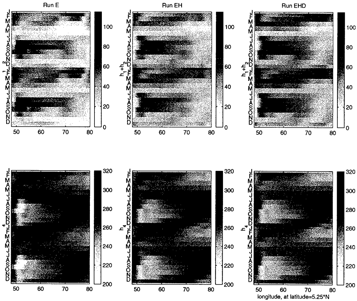
Figure 3.37 Westward propagation of layer depths h_1 + h_2 (top) and h_4 (bottom) in time at the fixed latitude of 5.25^\circ\text{N} , for Runs E, EH, and EHD. The last year of integration is repeated for clarity.
