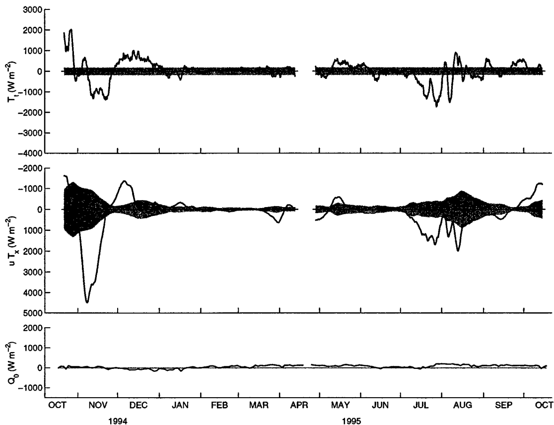
Figure 2.11 Terms in the heat budget, vertically integrated between the surface and 125m: the time trend ( top ), horizontal advection ( middle ), and the surface heat flux ( bottom ). The y-axis scale for horizontal advection is reversed, the temperature trend and horizontal advection terms tend to roughly cancel each other. Uncertainty is marked by the grey outline around the zero line.
