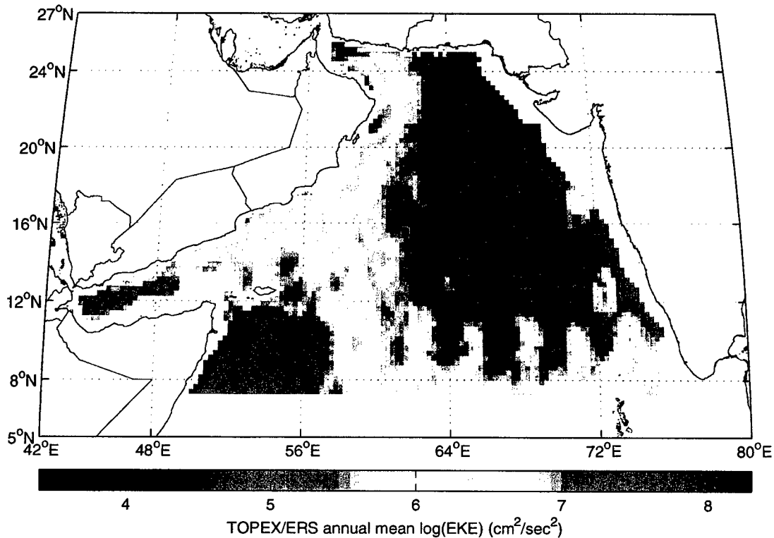
Figure 2.19 Mean eddy kinetic energy (in log scale) from the TOPEX/ERS anomaly field, calculated using data from the seven years 1992-1999. The dominance of the annually reversing Somali current system is apparent, and there are elevated levels along the Arabian coast and at low latitudes along the southernmost extent of the data. The region east of the mooring has low mean EKE.
