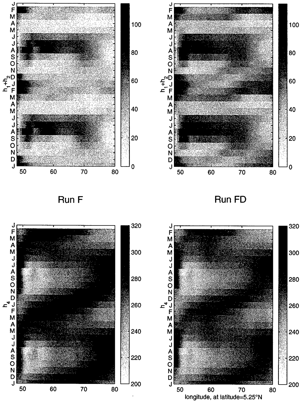
Figure 3.15 Propagation of h_1 + h_2 and h_4 at the fixed latitude of 5.25^\circ \text{N} , for run F ( left ) and run FD ( right ). The last year of the model solution has been repeated for clarity. The westward propagation of shallow mixed layers formed along the Indian coast during the SW monsoon is masked partially by the seasonal cycle in the upper layers. The surface layers are thicker in run FD, and the amplitude of the disturbance reduced.
