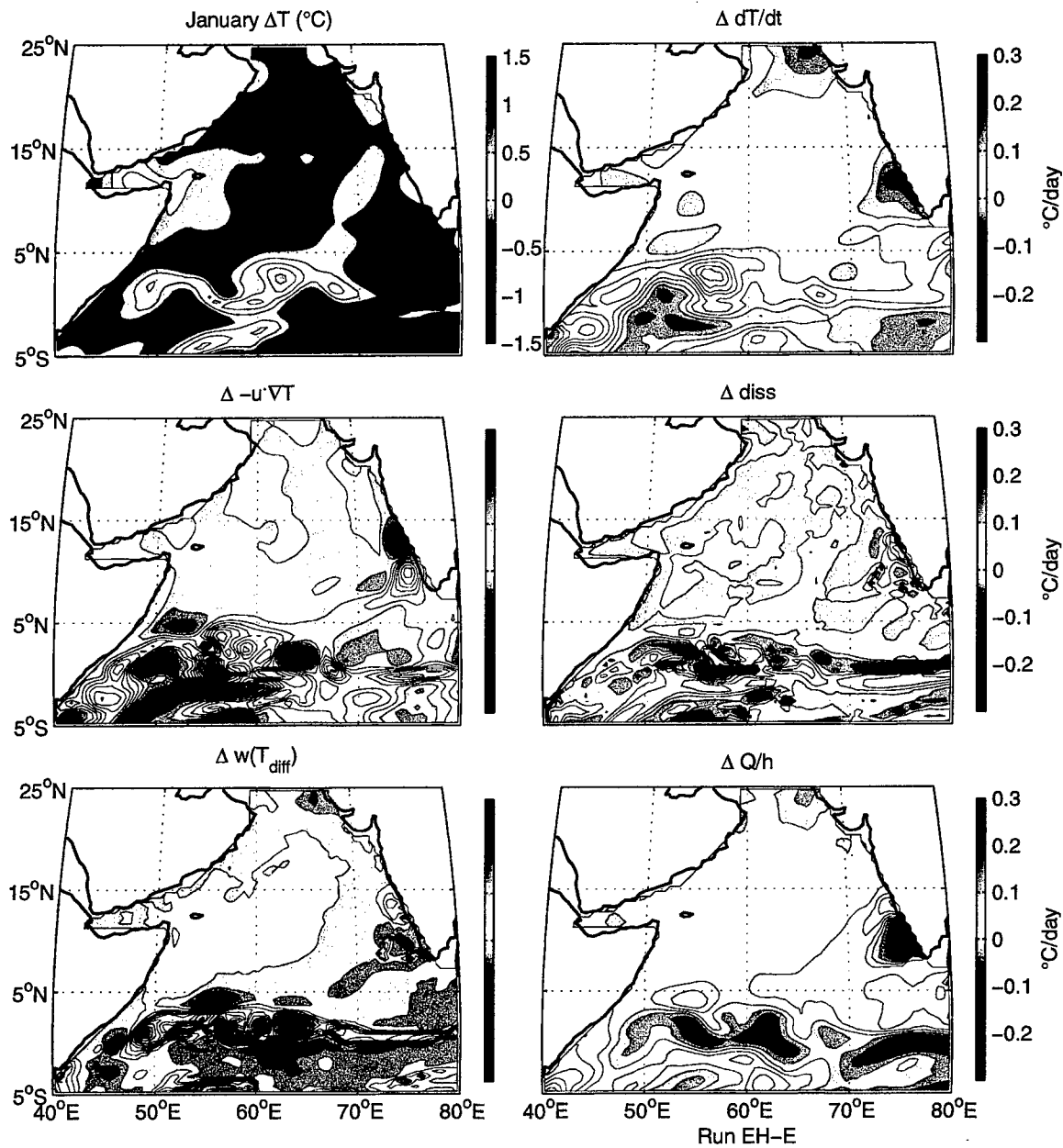
Figure 3.38 January run EH - run E difference in the terms of the temperature budget of the mixed layer. The largest differences come in equatorial regions, where run E has more entrainment cooling in a band stretching approximately along 3° N.
