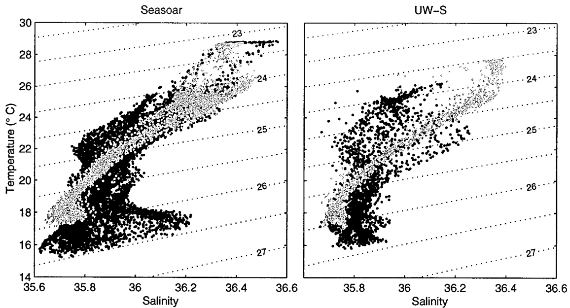
Figure 2.22 TS diagrams depicting the difference between the mean water mass during the SW monsoon ( gray ) and the coastally upwelled water ( black ). The left panel shows Seasoar spatial data, while the right panel shows the UW-S moored time series data. The distinguishing characteristics of the upwelled water are the two lobes above and below the mean water mass line. The lobe above is coastally upwelled water that has been in contact with the atmosphere, warming it, while the lobe below is remnants of the Persian Gulf outflow.
