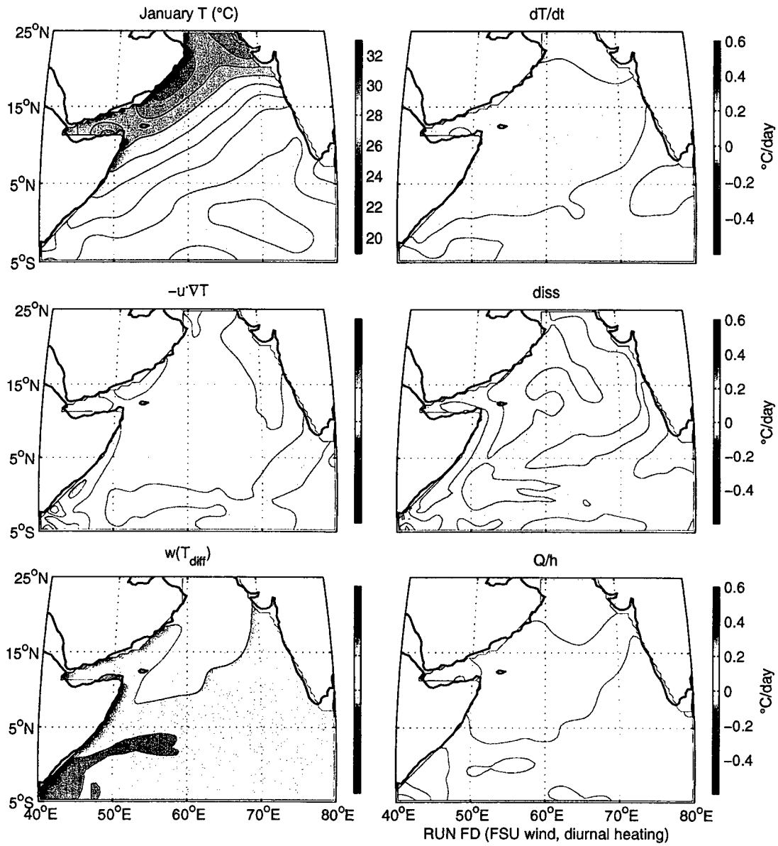
Figure 3.19 B January run FD, terms in the surface layer temperature budget. As in Fig. 3.19A except for Run FD.
