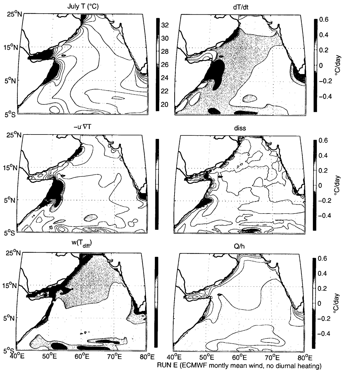
Figure 3.33 A July Run E, terms in the temperature budget. As in Fig. 3.16A except for run E.
