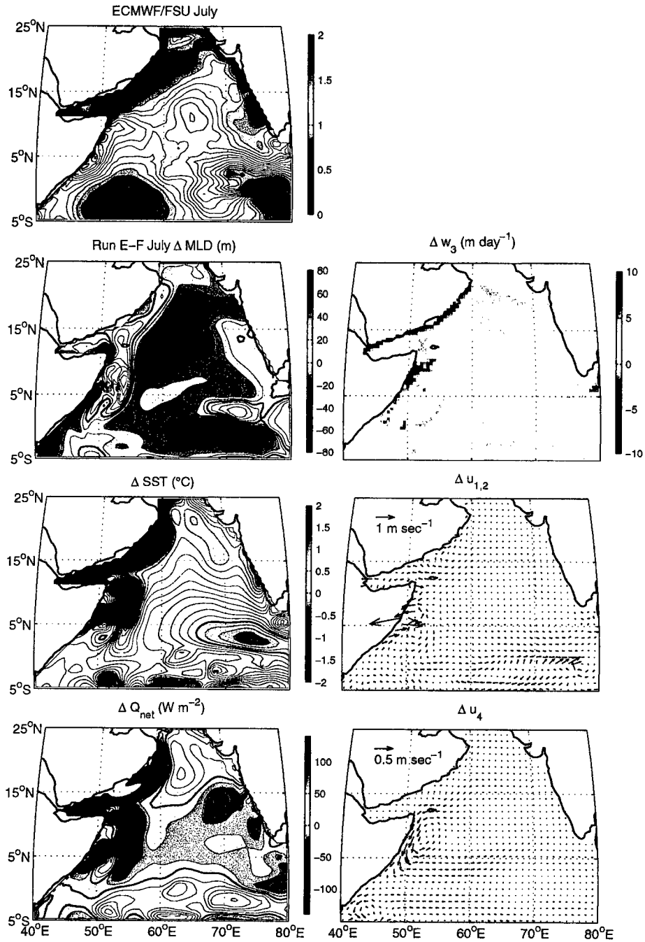
Figure 3.53 An overview of the differences between the model run E and model run F in July. The top left panel shows the scaled difference in the wind stress magnitude fields (ECMWF July 1995 divided by FSU July climatology, contours every 0.05, see Fig. 3.28 for the original fields): the ECMWF Findlater Jet is stronger, and more concentrated spatially than the FSU climatology. The rest of the panels are as in Fig. 3.14 and Fig. 3.32.
