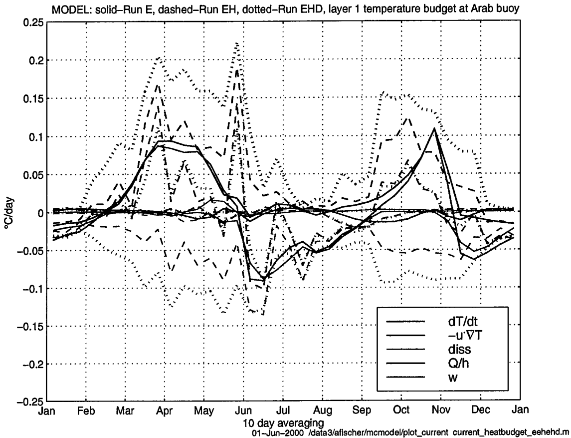
Figure 3.41 Terms in the surface layer temperature budget at the buoy (run E solid, run EH dashed, run EHD dotted). As in Fig. 3.21, except for the ECMWF-forced model runs.
