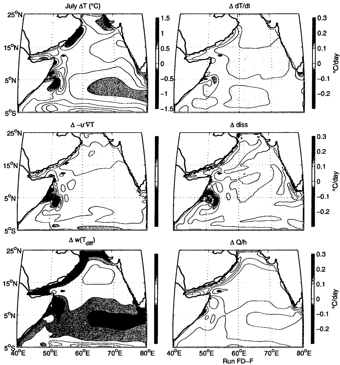
Figure 3.16 B As in Fig. 3.16A, except now the difference between Runs FD-F. Contours are now every 0.1^{\circ}\text{C} for \Delta T , and 0.02^{\circ}\text{C/day} elsewhere.
