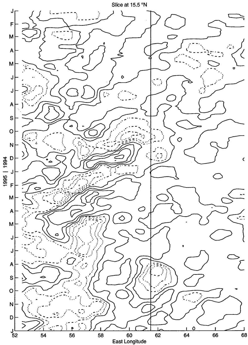
Figure 2.17 Time-longitude plot of ssh anomaly at the latitude (15.5 N) of the mooring, with the longitude of the mooring marked by the vertical line. Contours (positive solid) every 5 cm. There is evidence of westward propagation of anomalies. The coastal filament appears as a localized area of low ssh in July and August of 1995 at the longitude of the mooring.
