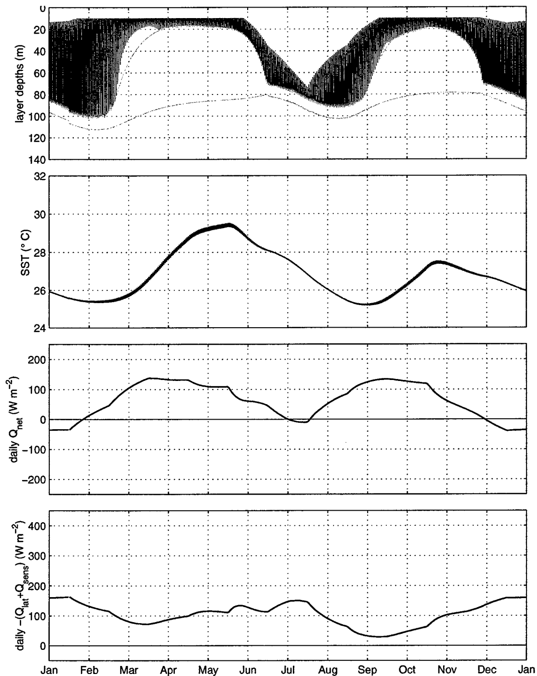
Figure 3.20 Run FD model solution at the mooring site. As in Fig. 3.11 except for run FD.
