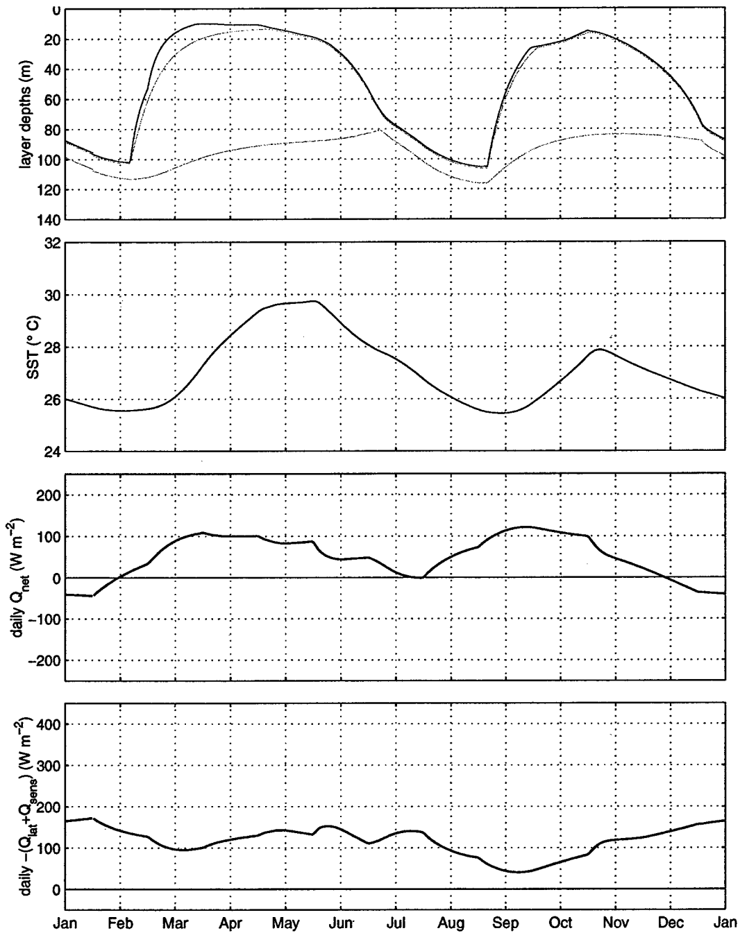
Figure 3.11 Run F Model solution at the site of the Arabian Sea buoy (61.5° E, 15.5° N). From top: the mixed layer depth (black) and the boundaries between layers 2, 3, and 4 (gray), the layer 1 temperature (SST), the daily average net surface heat flux, and the daily average sum of the surface latent and sensible heat losses.
