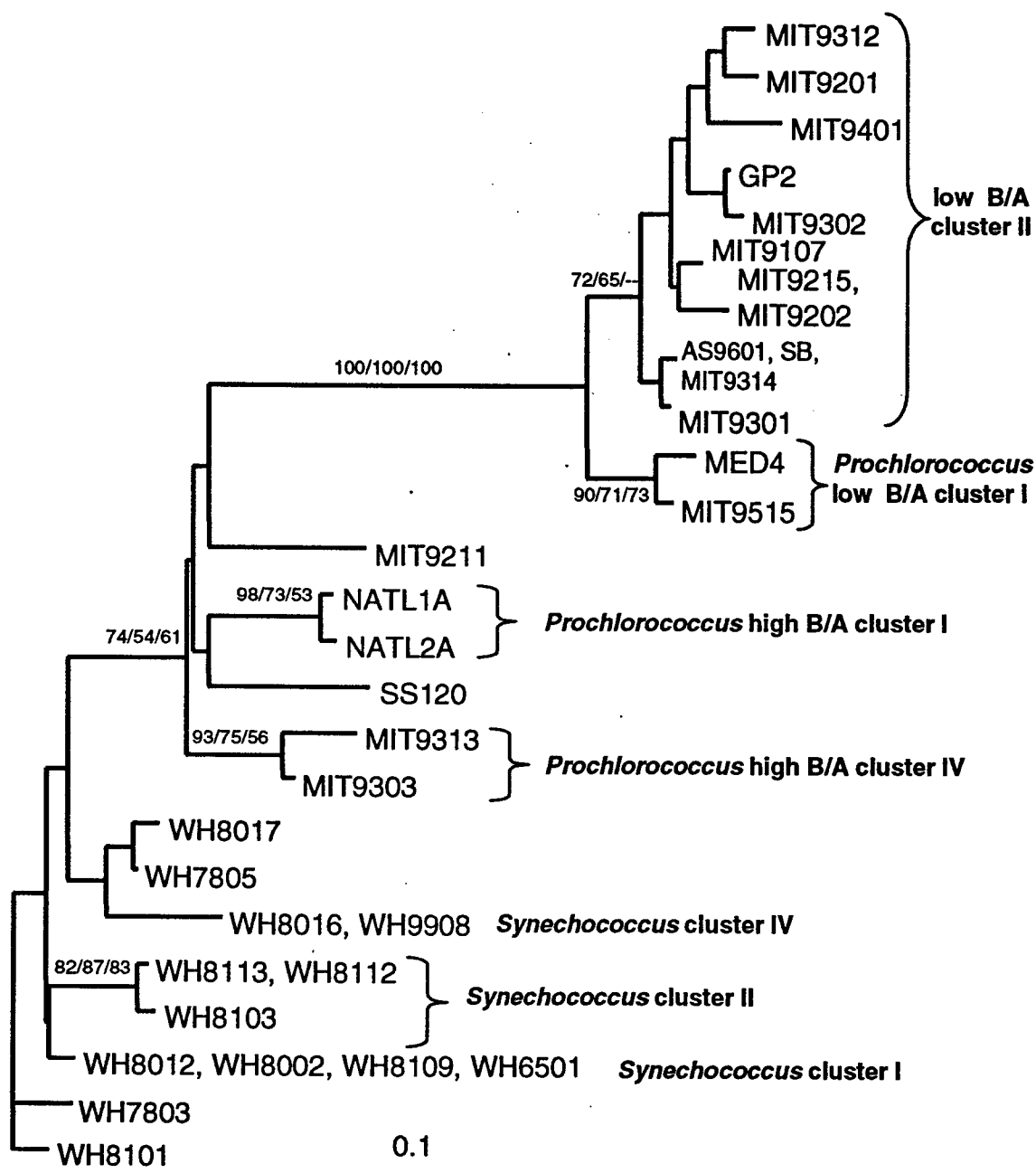
Figure 6. Evolutionary relationships of Prochlorococcus and Synechococcus isolates inferred using 103 positions of the 16S- tRNA Ile spacer. The phylogenetic framework was determined using paralinear distances (logdet) and minimum evolution as the objective function. Trees inferred using HKY85 distances resulted in identical clusters with essentially similar branching orders. Bootstrap values from [distance/maximum parsimony/maximum likelihood] analyses are listed to the left of each node, with values less than 50 not shown. The tree is arbitrarily rooted with WH8101.
