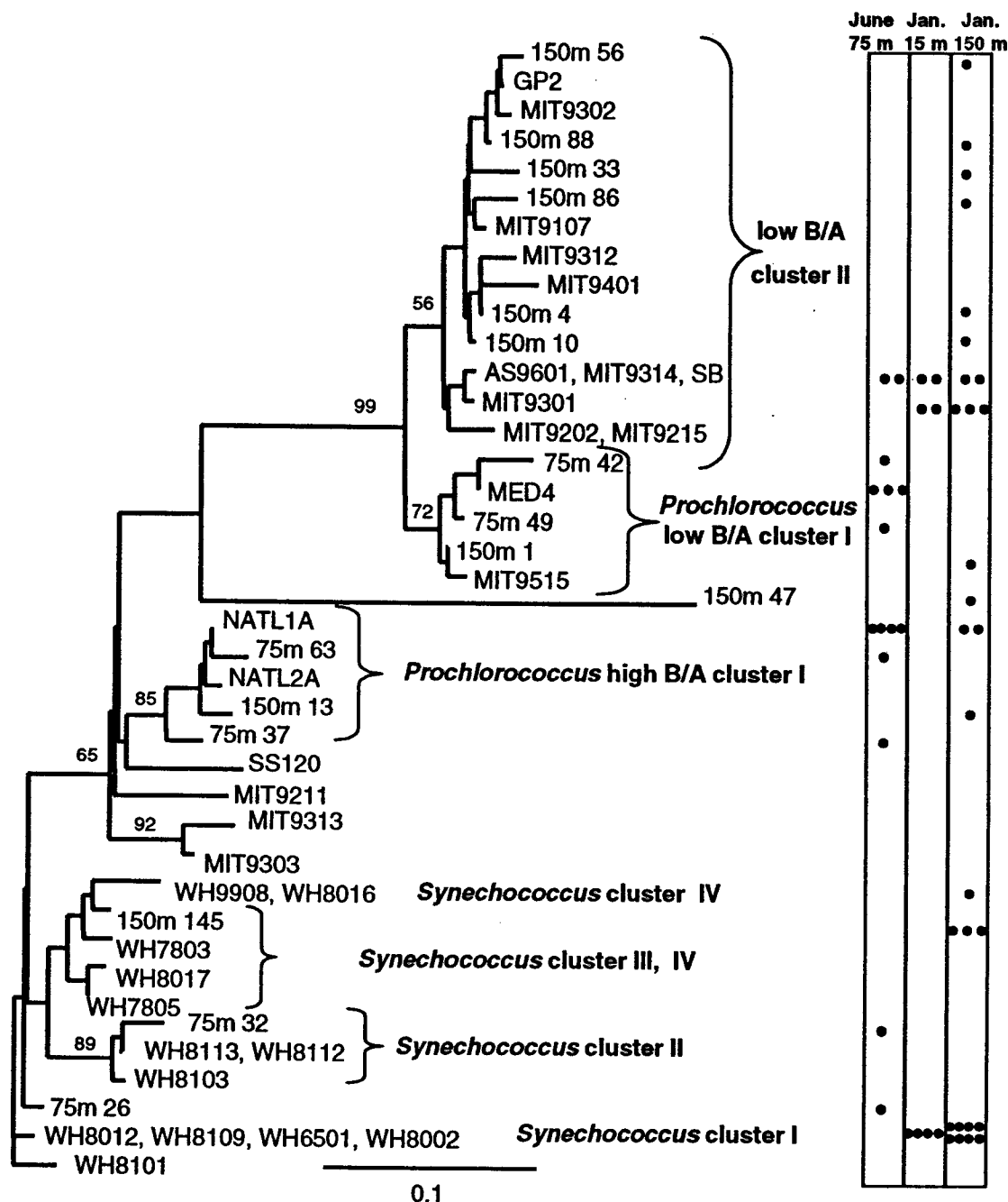
Figure 5. Evolutionary relationships of 51 environmental sequences with cultured isolates of marine cyanobacteria. Dots indicate sequences from clone libraries on tree, more than one dot on a line indicates sequences identical at the 103 positions of the 16S-tRNA Ile spacer used in the analysis. Phylogenetic framework inferred using a distance criterion with paralinear (logdet) distances and minimum evolution as the objective function. Bootstrap values from 100 resamplings are to the left of each node, values below 50 not shown. The tree found using likelihood methods assigned clones to same sequence clusters and was not significantly better as judged by the Kishino and Hasegawa test. Trees excluding low B/A Prochlorococcus and employing 146 positions of the 16S-tRNA Ile spacer resulted in essentially similar branching orders and exactly the same cluster assignments.
