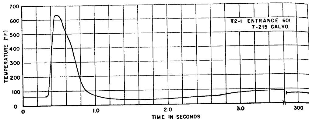
Temperature phenomena, Shelter 601, Experiment I 15
