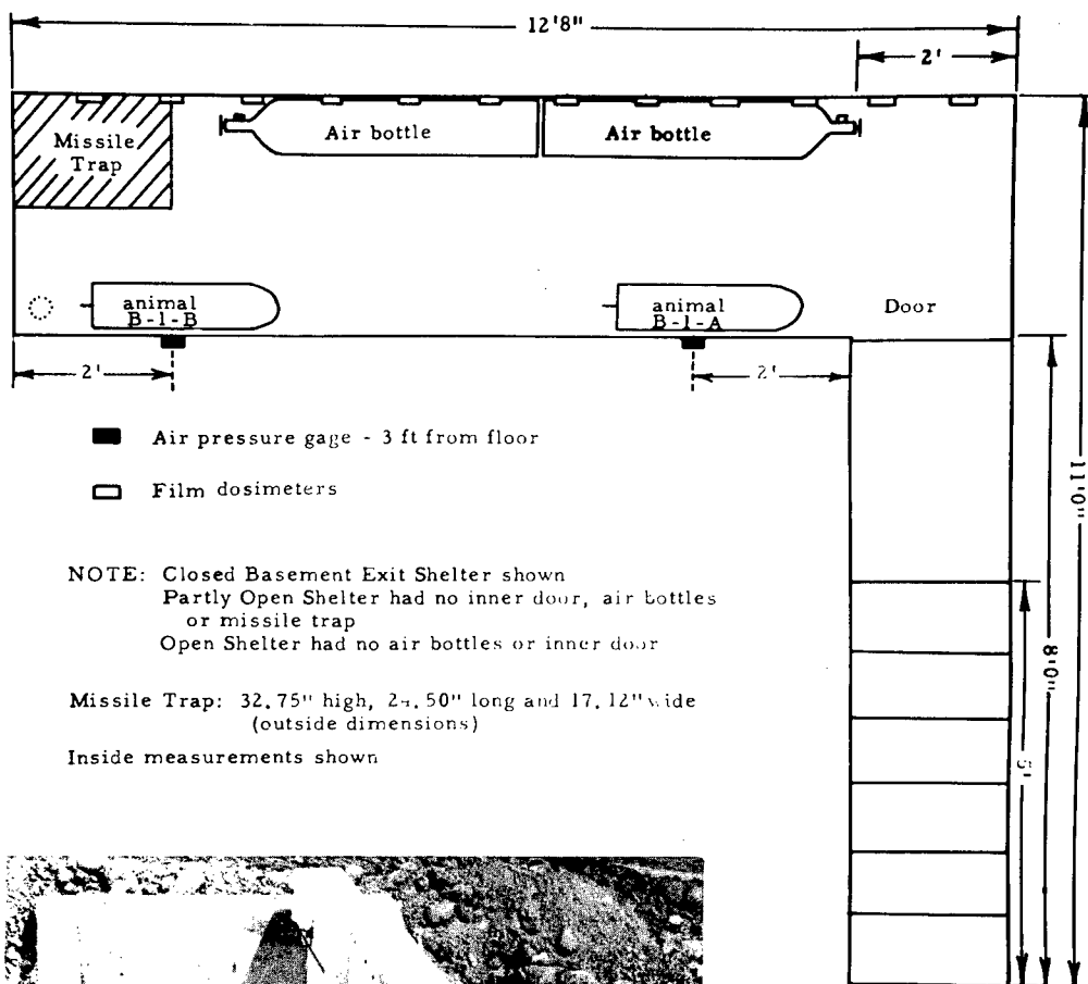
Basement exit shelter 4
