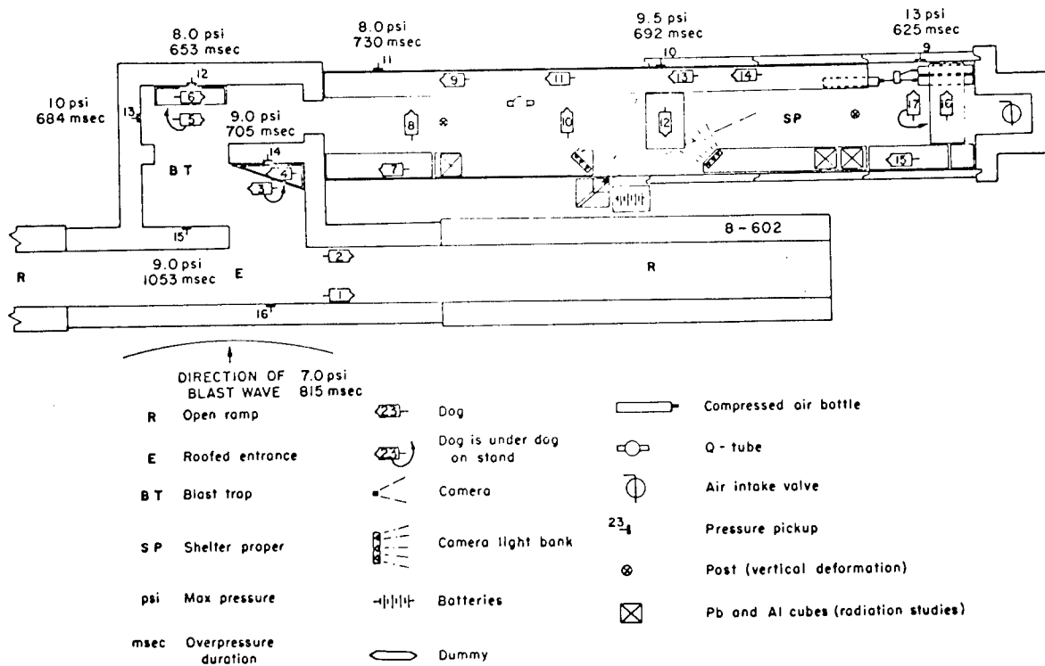
Plan view of 601 and 602 Shelters and contents as used on Experiment II. Maximum recorded overpressures and their durations also shown. 3
