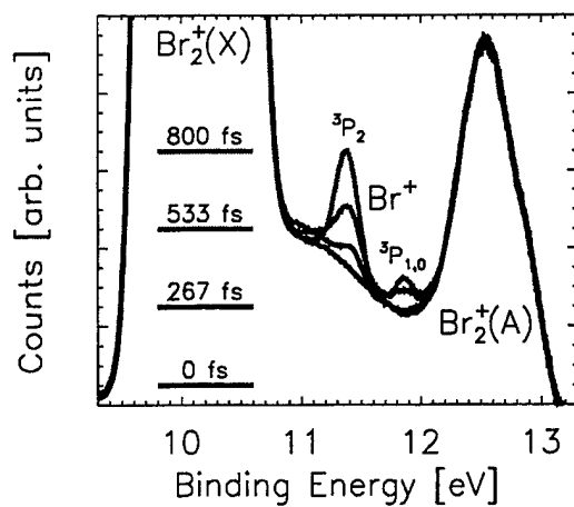
Figure 12 Time dependent signals of bromine dissociation. The new peaks are due to \text{Br} atoms during the dissociation.
