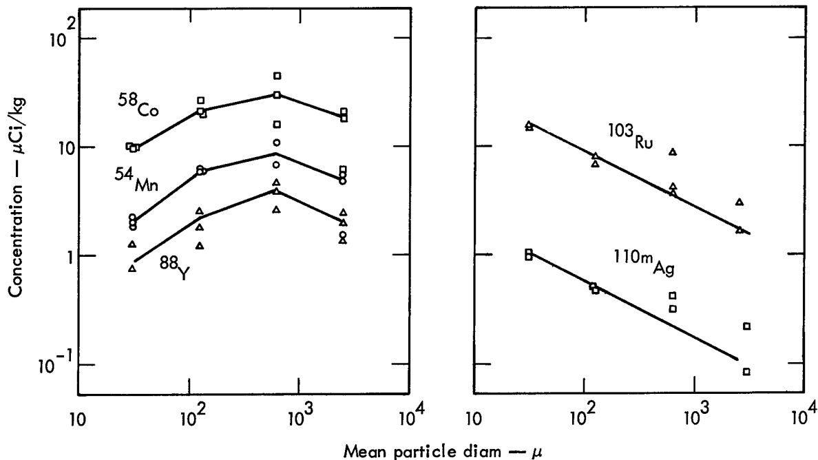
Fig. 48. Radionuclide concentrations in Schooner debris as a function of particle size. Left, ^{54}\text{Mn} , ^{58}\text{Co} , and ^{88}\text{Y} . Right, ^{103}\text{Ru} and ^{110\text{m}}\text{Ag} .
