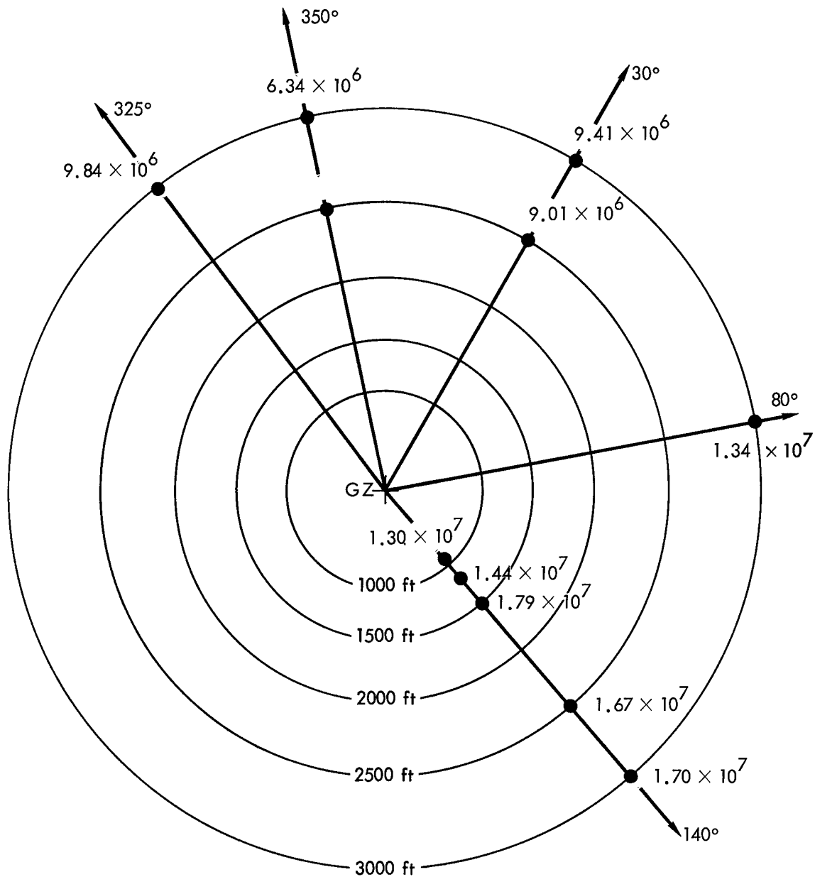
Fig. 41. Concentrations of ^{181}\text{W} in surface ejecta from the crater lip to 3000 ft. The data are in dis/min/g; N = 0 deg.
