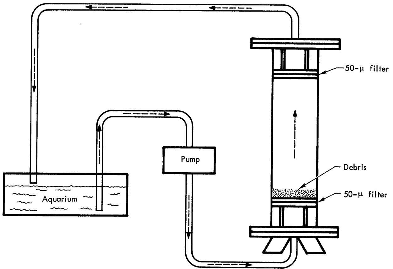
Fig. 49. Diagram of the system for determining the biological availability to aquatic organisms of radionuclides in debris.
