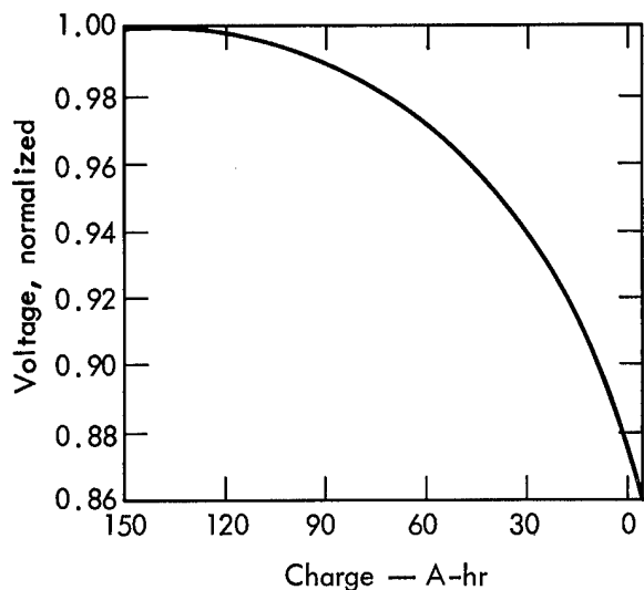
Fig. 7. Normalized battery voltage for a 150 A-hr lead-acid battery as a function of battery charge.
