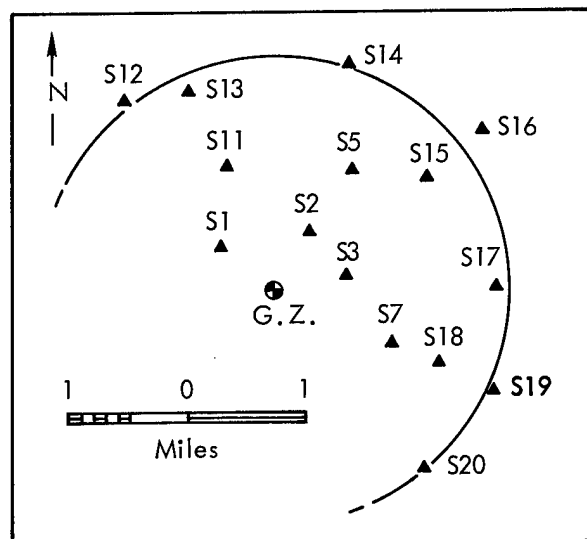
Fig. 35. The array of close-in fallout trays. Three trays were placed at each location. The arc is the 2-mile arc.
