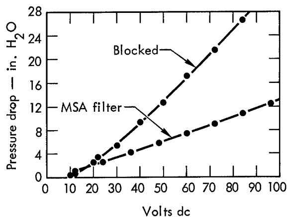
Fig. 6. The relationship between the pressure drop across the filter and a blocked filter as a function of voltage applied to the air pump (Sears Vacuum Cleaner Model-7150).
