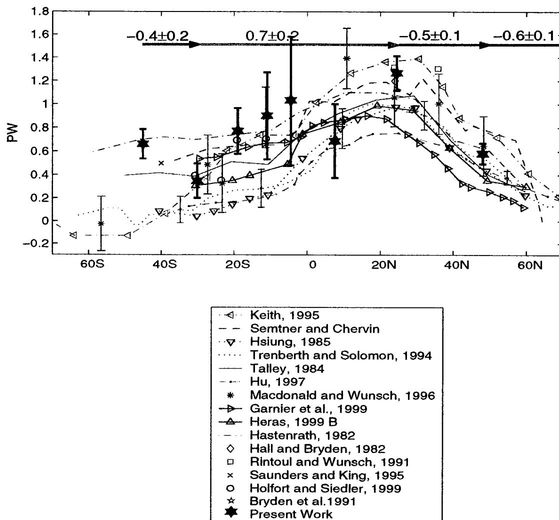
Figure 4-4: Atlantic energy transports (black stars with thick error bars) and residuals between selected latitudes (numbers above the northward-pointing arrows, positive for heating). (The energy flux at 7.5°N is probably noisy due to variability in the North Brazil Current region.) Errorbars from Holfort and Siedler (1999) are of \pm 0.3 PW; Rintoul and Wunsch (1991), \pm 0.2 PW; Hall and Bryden (1982), \pm 3 PW; and Saunders and King (1995), \pm 0.1 PW. (Adapted and completed from Macdonald and Wunsch (1996) and Heras and Schlitzer (1999).)
