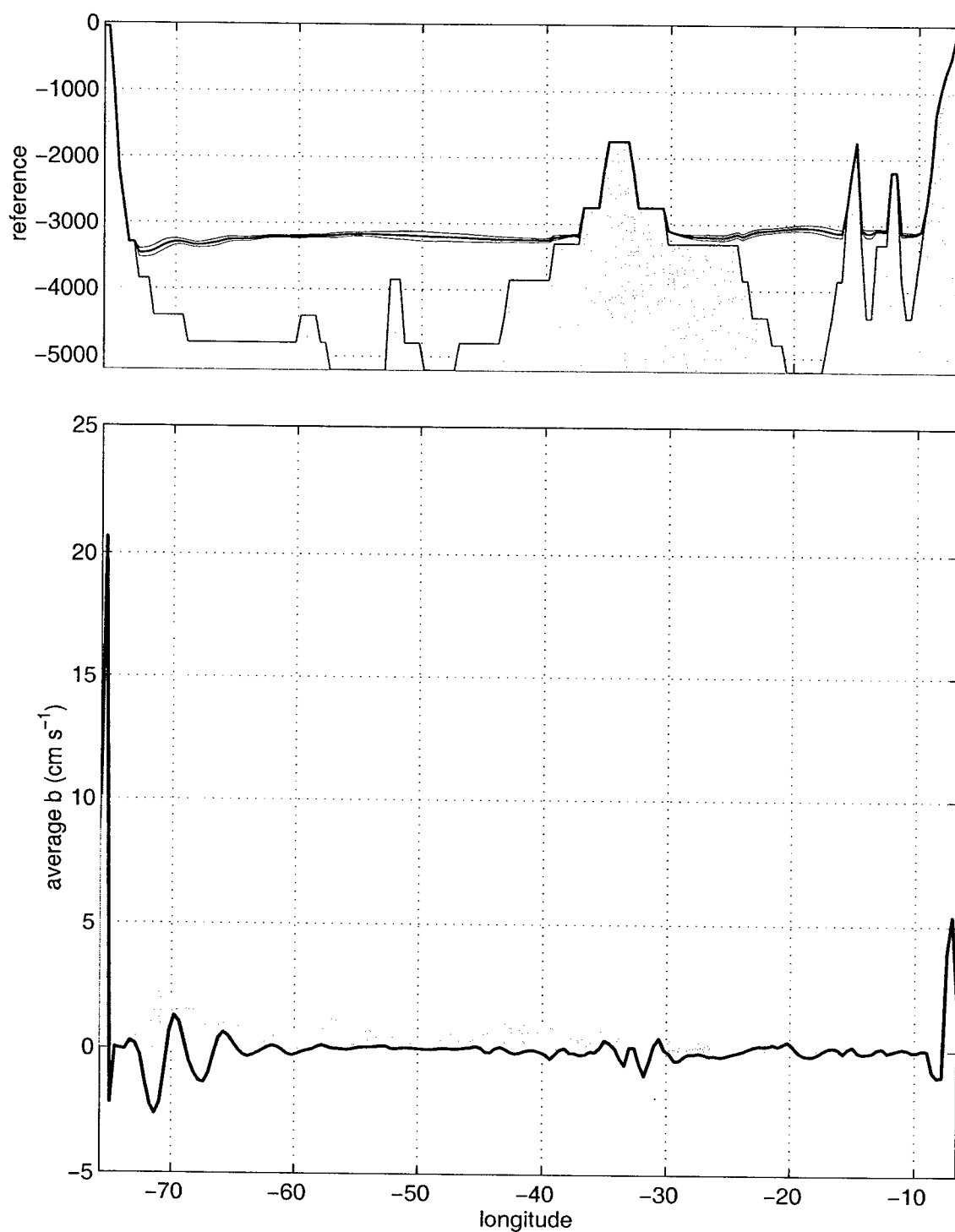
Figure 2-11: Upper panel: reference isopycnal ( \sigma_4 = 45.81 ) for section 36^\circ\text{N} . The isopycnal oscillates by less than 100 m around its mean position (thick line). One standard deviation is indicated by the thin lines. Lower panel: mean reference velocities (thick line) and variance (1std. dev, shaded area).
