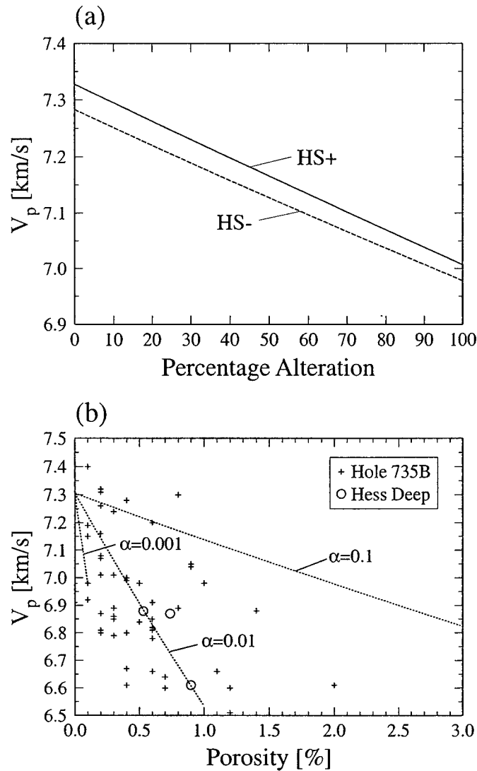
Figure 3-10. (a) Effect of hydrothermal alteration on gabbro velocity. Unaltered gabbro composition used here has 47% plagioclase ( An_{60} ), 35% clinopyroxene ( Di_{80} ), and 18% olvine ( Fe_{75} ), which is the average of oceanic gabbroic rocks recovered from ODP Hole 735B, as reported by Dick et al. [1991]. We assume hydrothermal alteration simply results in the replacement of clinopyroxene with hornblende. Elastic moduli and density are first calculated for each mineral at 100 MPa and 100°C, and Hashin-Shtrikman bounds for mineral assemblage are then calculated. (b) Effect of residual crack porosity on gabbro velocity. We first calculated effective elastic moduli of dry porous rock with different pore aspect ratio (0.1, 0.01, and 0.001) using the formula of Kuster and Toksöz [1974], and then applied the Gassmann low-frequency relations to obtain effective moduli for fluid saturated porous rock [e.g., Mavko et al. , 1998]. Elastic moduli for seawater are taken from Wilkins et al. [1991], and elastic moduli for pore-free gabbro are taken from the average of Hashin-Shtrikman bounds as calculated in (a). The results are shown as dotted lines. Also shown are velocity-porosity data of gabbroic rocks recovered from ODP Hole 735B (cross) [ Iturrino et al. , 1991] and Hess Deep (open circle) [ Iturrino et al. , 1996]. While porosity data are measured at atmospheric pressure, velocity data are measured at 200 MPa.
