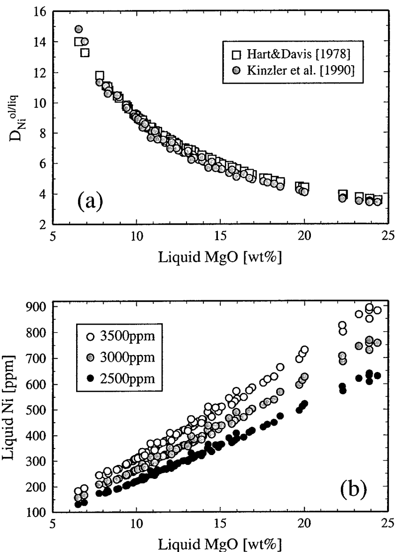
Figure 4-4. (a) A range of molar D_{Ni}^{ol/liq} (defined as X_{NiO}^{ol}/X_{NiO}^{liq} , which is 1.5 times smaller than the definition of Kinzler et al. [1990], X_{Ni_2SiO_4}^{ol}/X_{NiO}^{liq} ) are calculated using the equation of Kinzler et al. [1990] and the compositions of experimental mantle melts used in Figure 4-2. The result based on the equation of Hart and Davis [1978] is also shown. (b) The Ni concentration of liquid in equilibrium with olivine with 2500-3500 ppm Ni is shown as a function of liquid MgO, using the equation of Kinzler et al. [1990] and the same experimental mantle melts used in (a).
