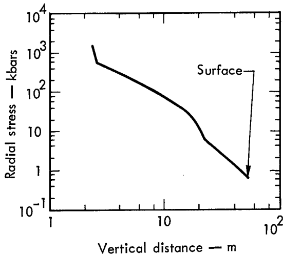
Fig. 26. Predicted peak radial stress as a function of distance about the Cabriole shot point.
