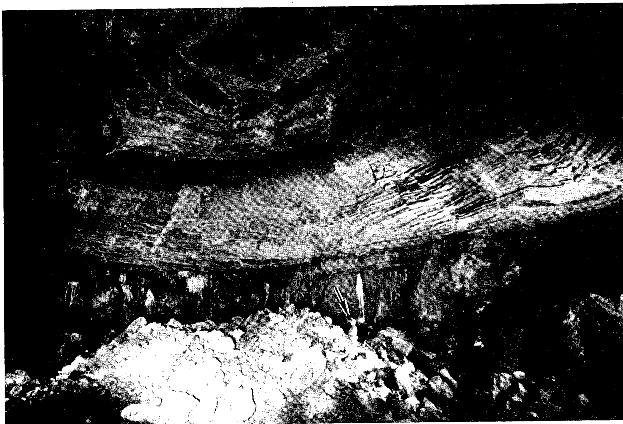
Fig. 1. Cavity formed by an underground nuclear explosion. The man standing on the rubble pile (arrow) indicates the scale.
