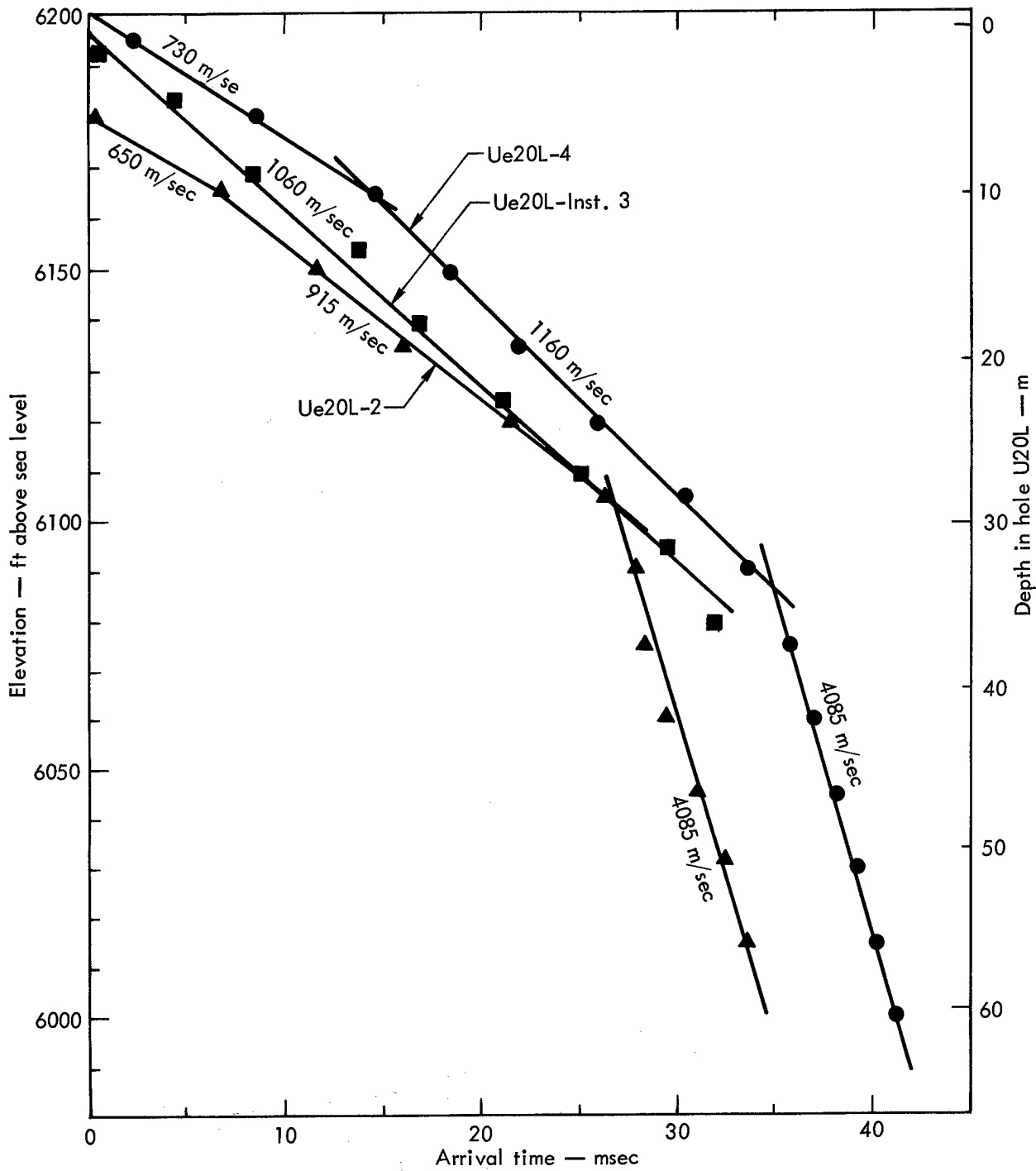
Fig. 24. Seismic velocity data from Cabriolelet site.
