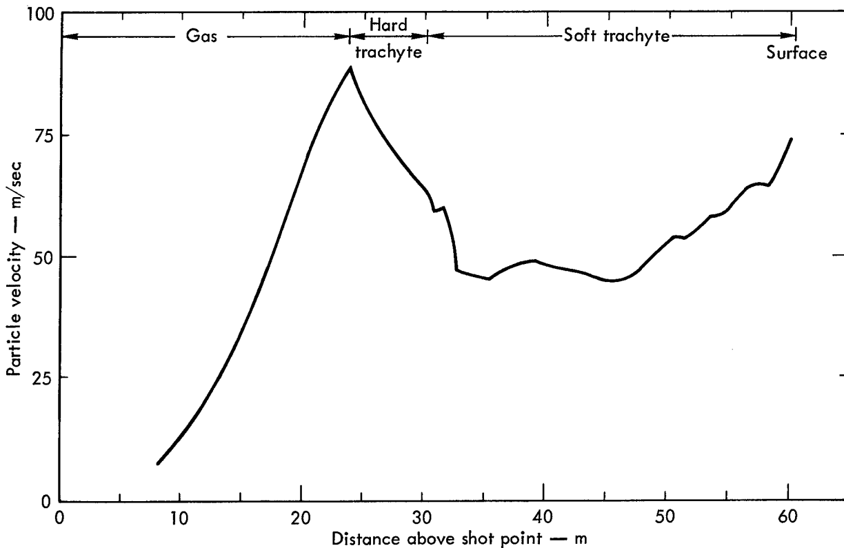
Fig. 27. Calculated particle velocity versus distance above Cabriole shot point at 135 msec.
