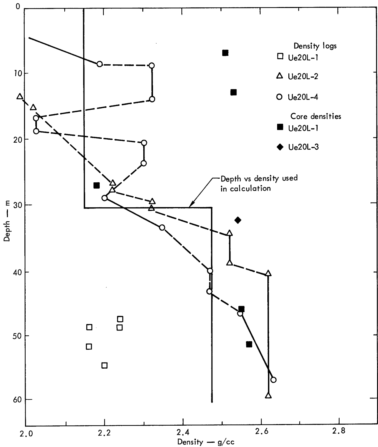
Fig. 25. Density measurements in the vicinity of the Cabriole emplacement hole .
