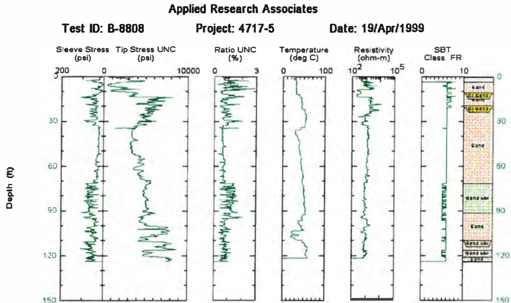
Figure 44. Static CPT data collected at Hanford using the newly developed digital CPT cone and SMR module. Sonic data were recorded at depth beginning at 105 ft.
