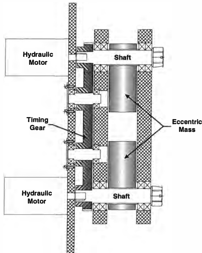
Figure 19. Preliminary testing demonstrated the importance of insuring that the eccentric masses were synchronized. This was accomplished by adjusting the helical-cut gears on their respective shafts to assure that the centroid of each eccentric weight reaches the apex of rotation simultaneously.
