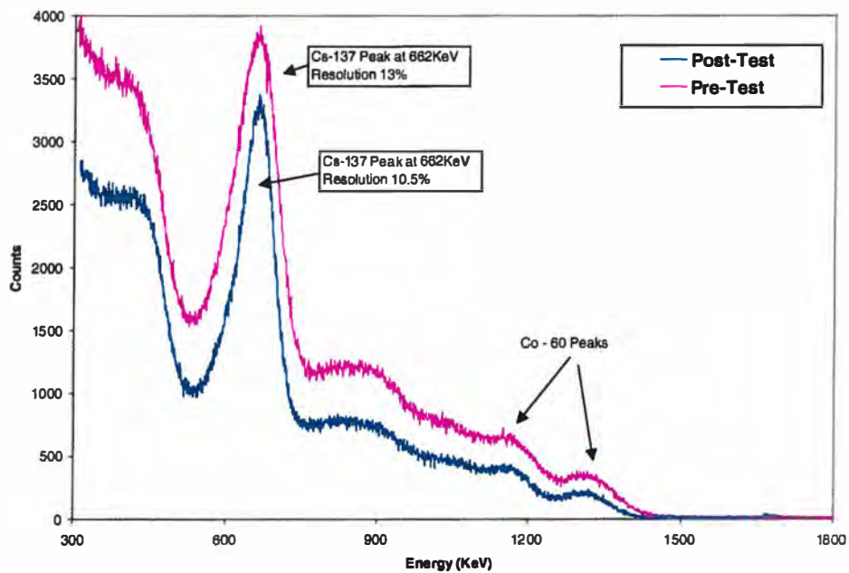
Figure 45. Cesium and cobalt spectra collected with the sonic gamma probe before and after field testing.
