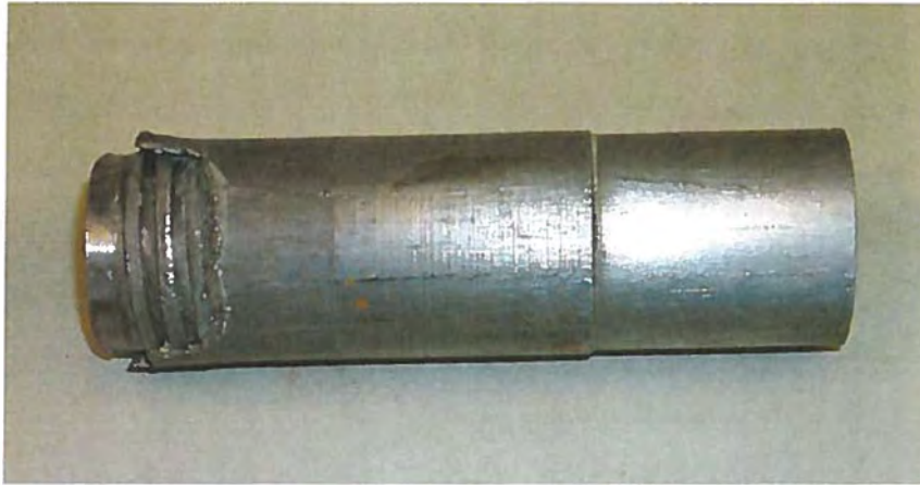
Figure 41. Photo illustrating the breakage of a core barrel. The failure occurred at the shoulder of the male thread on the up-hole end, where it threads into the adapter.
