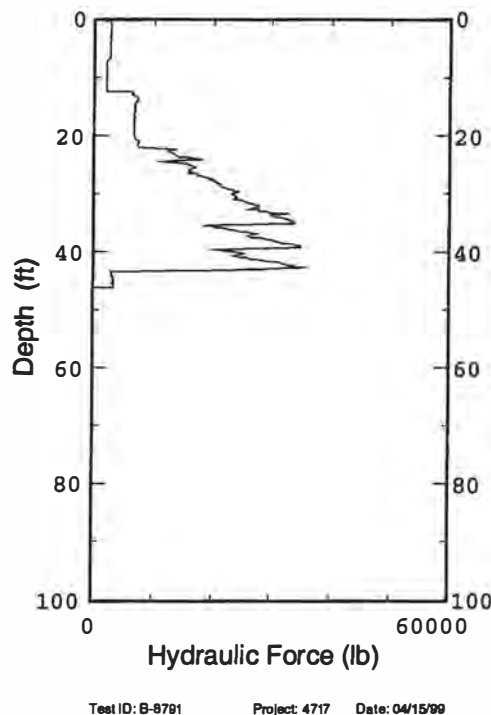
Figure 43. Hydraulic force verses depth for the penetration conducted at location B8791.
