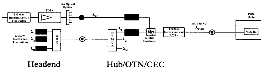
Figure 3 – Dual-hub-receiver (DHR) design.
