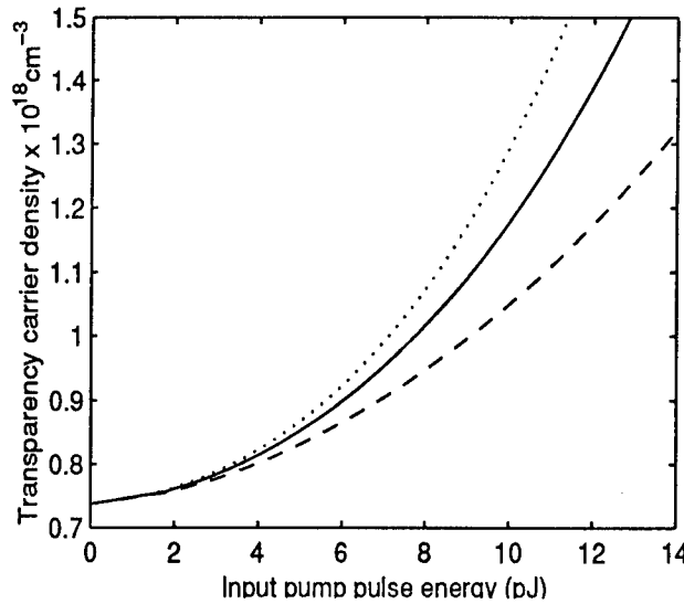
Figure 1: The transparency carrier density as a function of the input pump pulse energy for different SOA lengths. The SOA lengths for the dotted, solid and dashed lines are 125 \mu\text{m} , 250 \mu\text{m} and 500 \mu\text{m} respectively.
