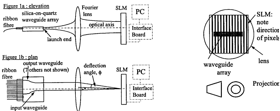
Figure 1: Operation of the ROSES 1 \times 8 holographic routing switch.
