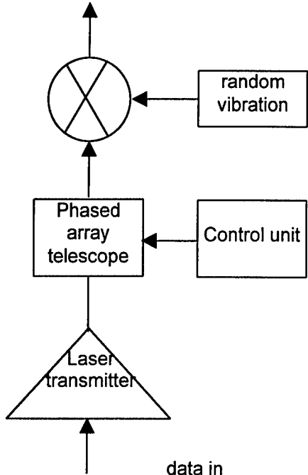
Fig. 2. Transmitter model
