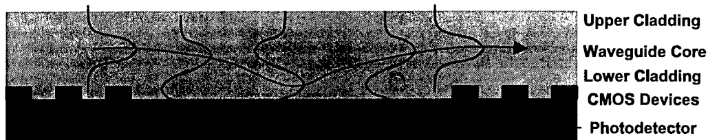
Figure 3: Side view cross section of the optical tap, showing multimode oscillation
