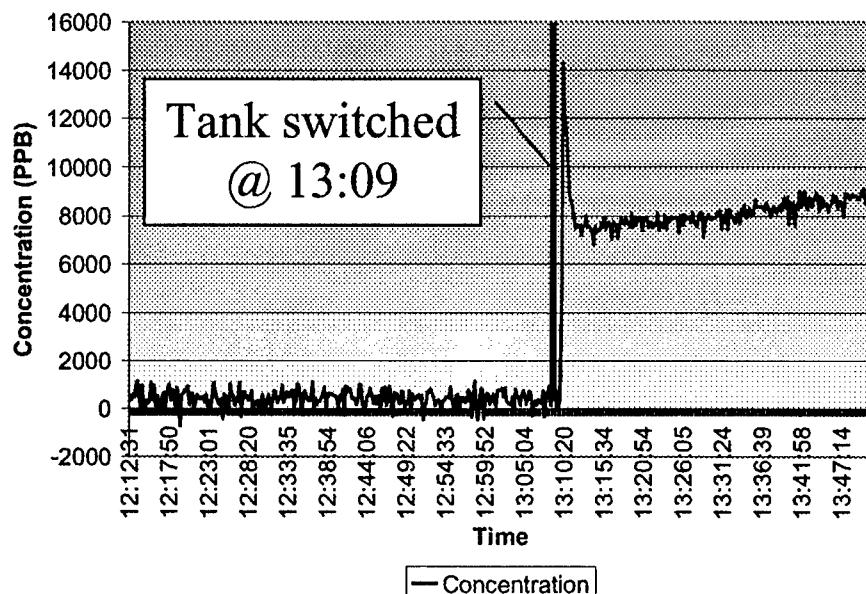
Figure 3 Illustration of Fast-Response Detection of Moisture by SpectraStream™
