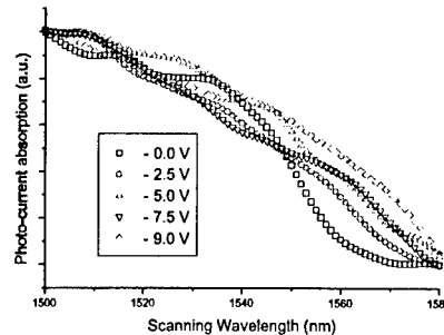
Figure 2 Photo-current absorption for modulator, with energy band-gap shifted by 24nm (channel 6) under 0.0 – 9.0 V bias.
