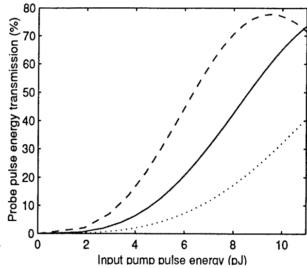
Figure 2: The probe pulse energy transmission versus the input pump pulse energy in a TSOA-NOLM. The SOA lengths for the dotted, solid and dashed lines are 125 \mu\text{m} , 250 \mu\text{m} and 500 \mu\text{m} respectively.
