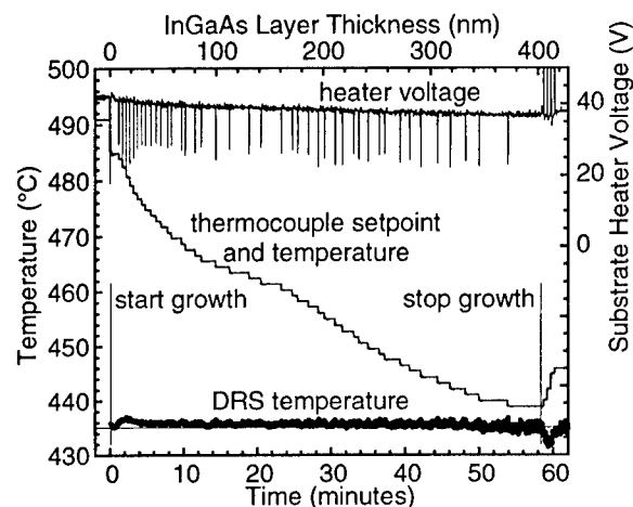
Fig. 4. Real-time control of substrate temperature during the growth of lattice-matched InGaAs on semi-insulating InP, using diffuse reflectance spectroscopy (DRS). The substrate setpoint is 435^\circ\text{C} .
