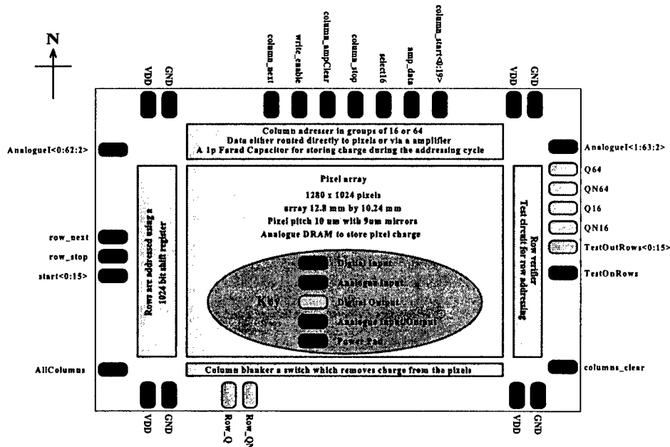
Figure 2 Backplane schematic
