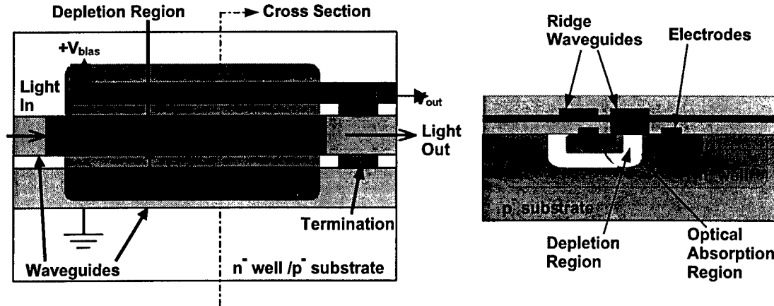
Figure 2: Detailed top and cross sectional views of the tap design. Note the high-speed traveling wave design for the photodetector for high speed optical to electrical conversion.
