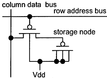
Figure 3. Pixel circuit
