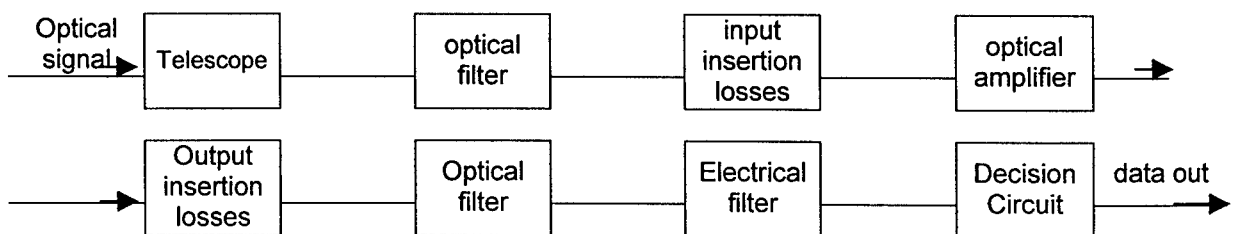
Fig. 1. Receiver scheme
