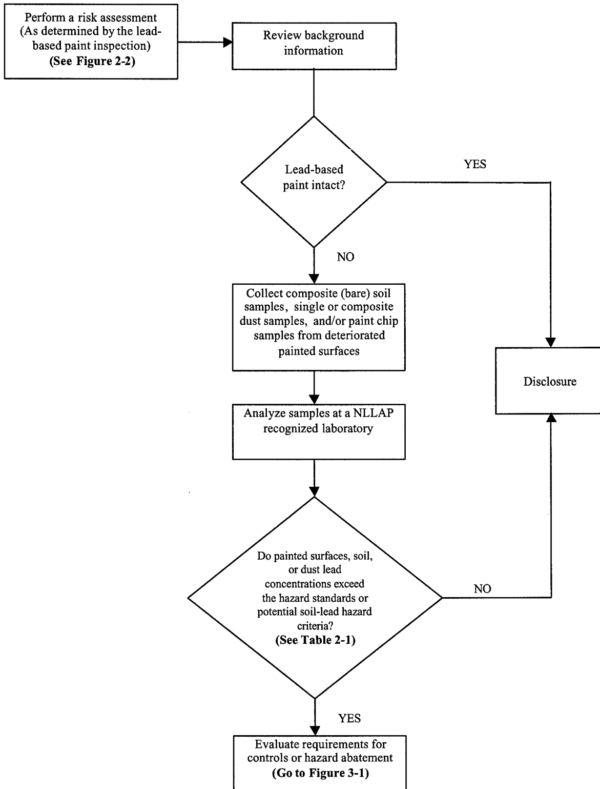
Figure 2-3. The Risk Assessment Process
