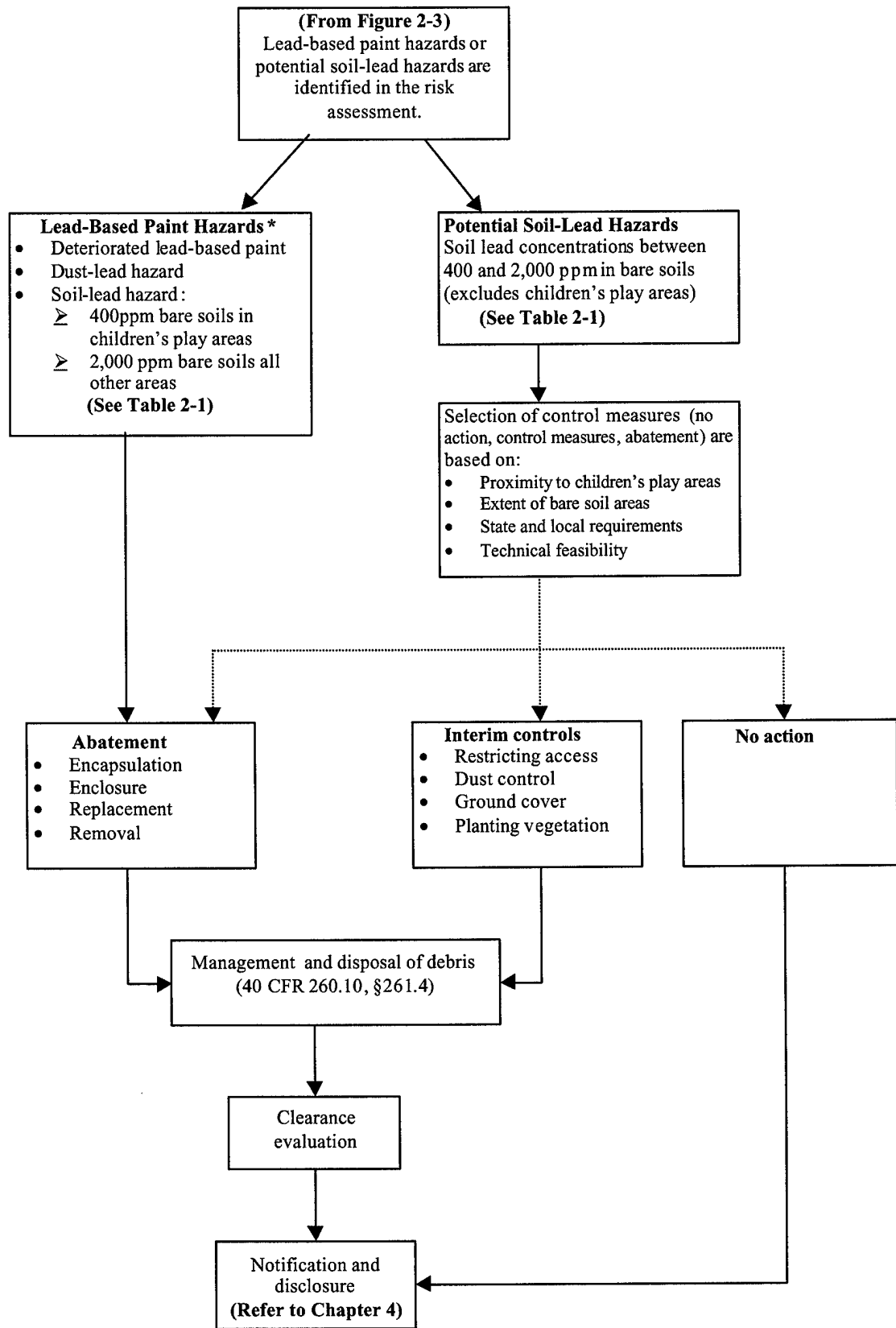
Figure 3-1. Control and Hazard Abatement Measures
