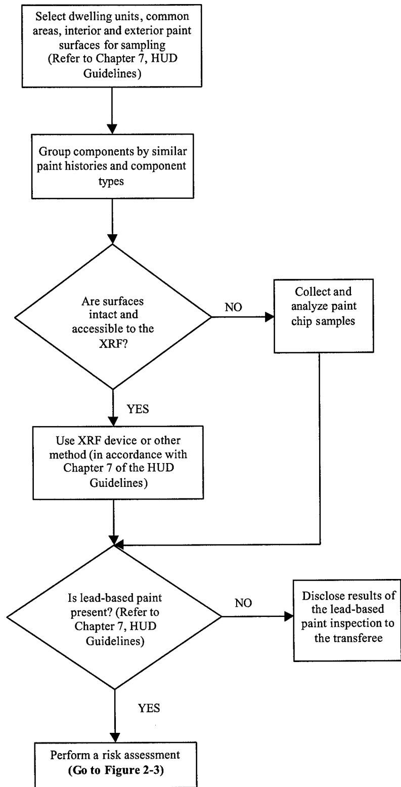
Figure 2-2. The Lead-Based Paint Inspection Process
