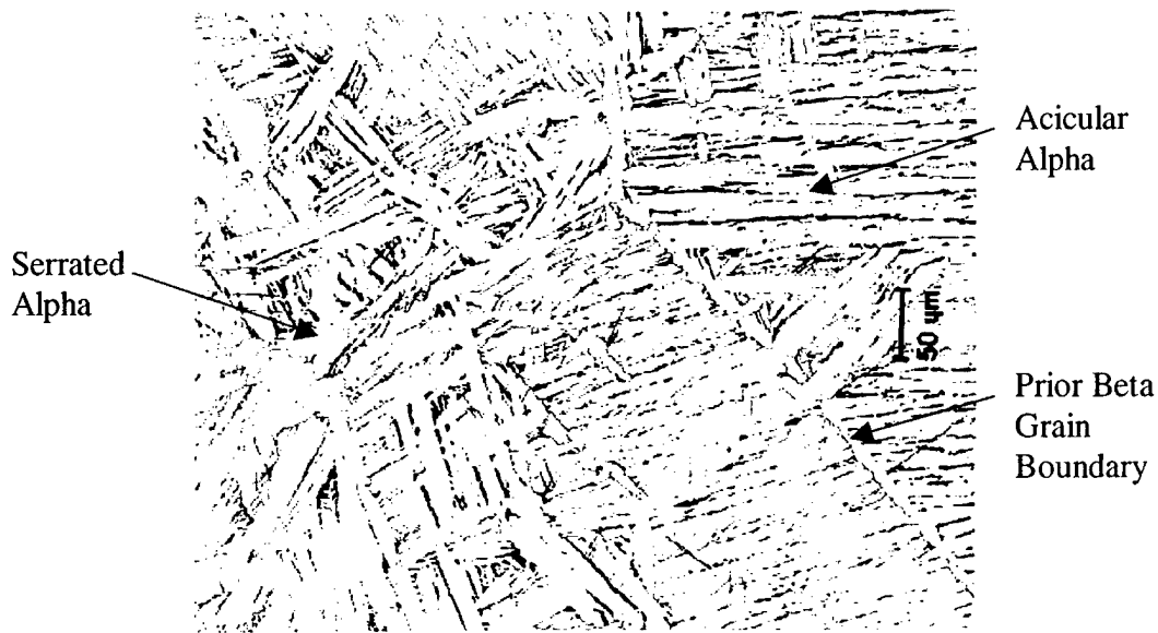
Figure 3. Microstructure of PPT-2 weld deposit.
