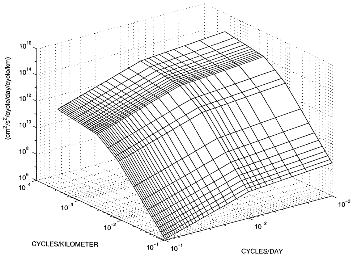
Figure 9-1: Two-dimensional zonal-wavenumber and frequency spectrum. Meridional-wavenumber and frequency spectrum is the same.
