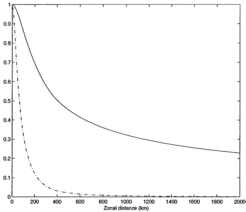
Figure 6-4: The normalized \sigma_{[\theta]}^2(L, n, \lambda, \phi) (solid line) and \sigma_{[v]}^2(L, n, \lambda, \phi) (dashdot line) as a function of L . \sigma_{[\theta]}^2(L, n, \lambda, \phi) and \sigma_{[v]}^2(L, n, \lambda, \phi) are normalized by \sigma_{[\theta]}^2(L = 0, n, \lambda, \phi) and \sigma_{[v]}^2(L = 0, n, \lambda, \phi) , respectively.
