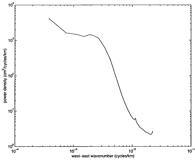
Figure 4-9: The scalar zonal-wavenumber spectra.
