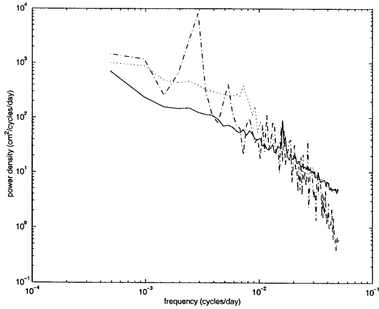
Figure 4-11: The frequency spectra of eastward-going (solid line), westward-going (dotted line) and standing motions (dashdot line). The frequency spectrum of standing motions is dominated by annual cycle.
