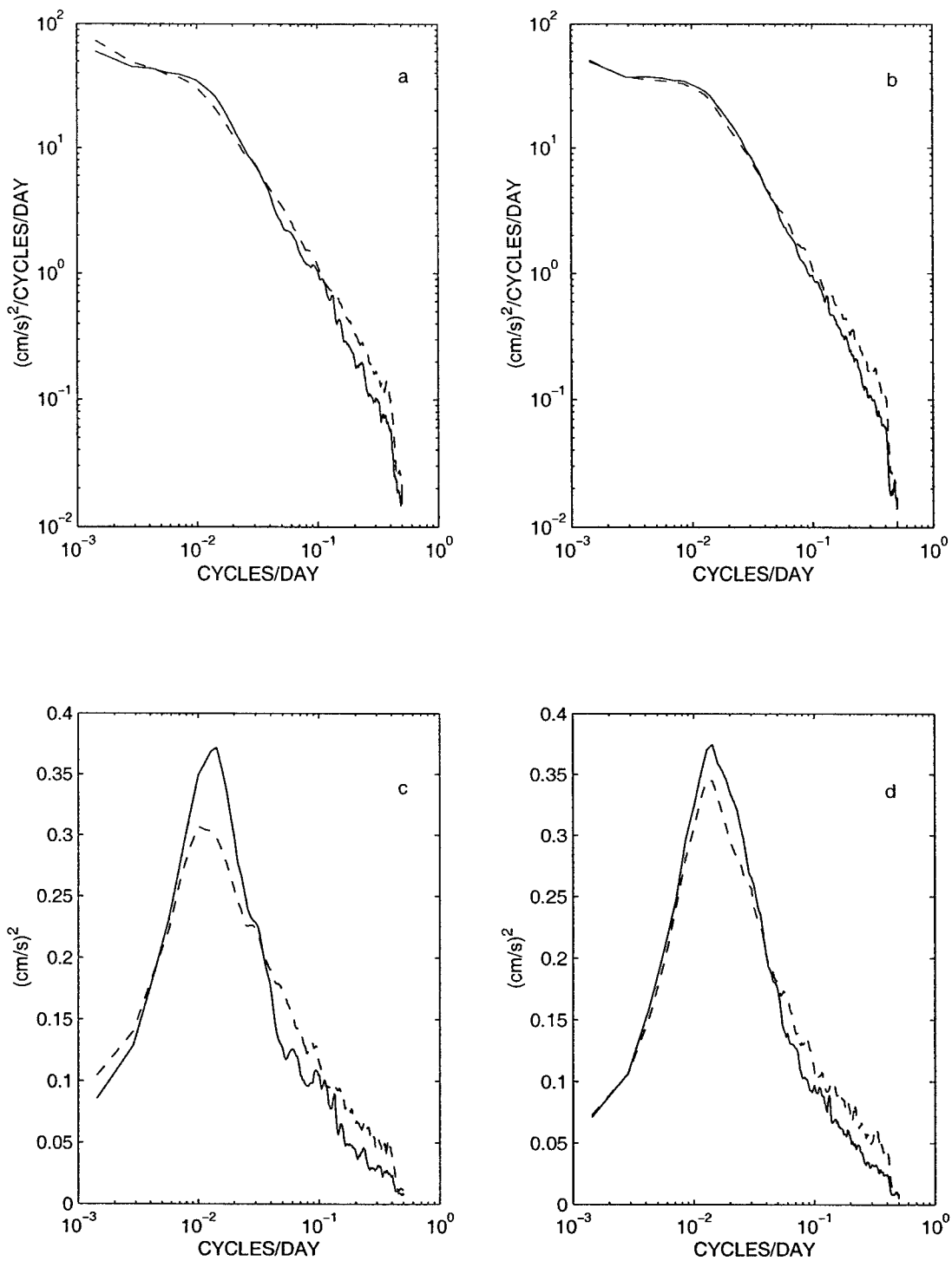
Figure 4-15: The mean normalized frequency spectra of zonal (a) and meridional (b) velocities in the barotropic (solid line) and first baroclinic modes (dashed line) from 105 current meter measurements (see Wunsch 1997). The variance-preserving form of zonal (c) and meridional (d) velocities. At each site, the spectra have been normalized by their total energy before the spatial average is done.
