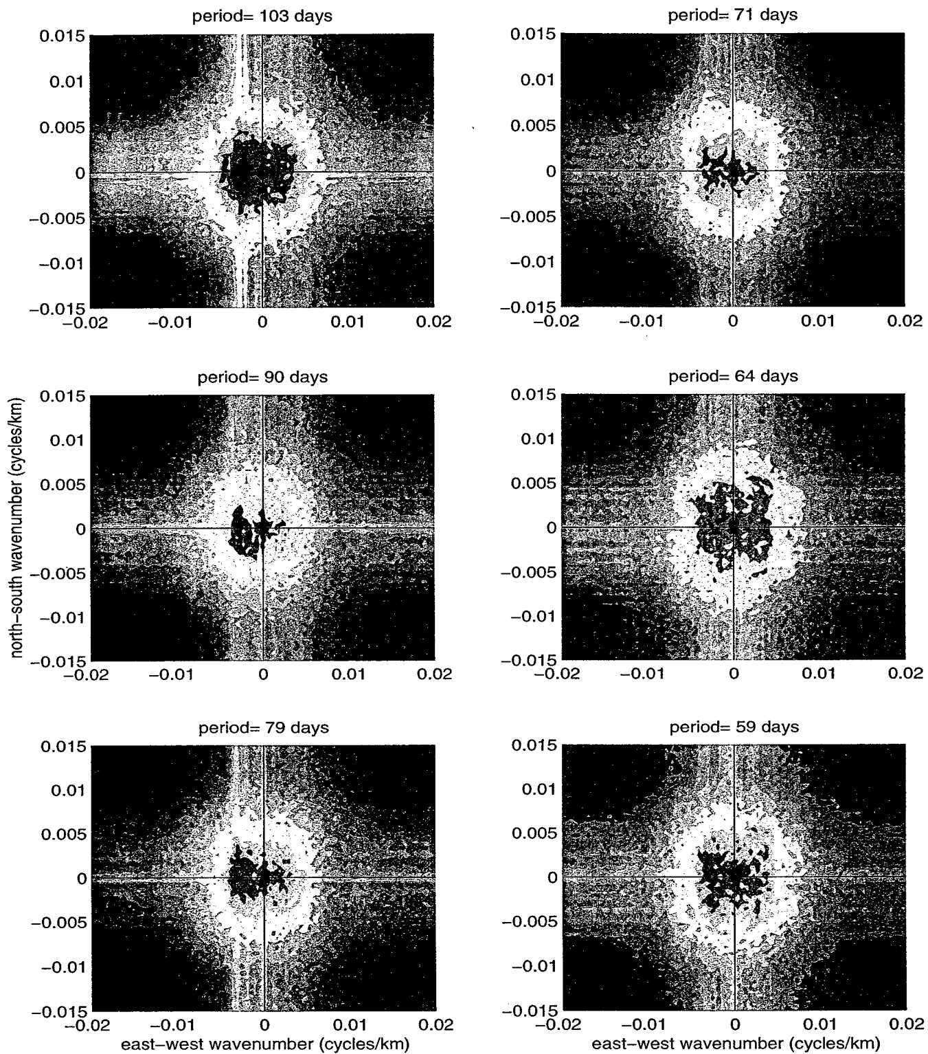
Figure 4-4: The smoothed three-dimensional spectra at periods longer than 59 days. The spectra at shorter periods are similar except that the energy distribution is nearly isotropic.
