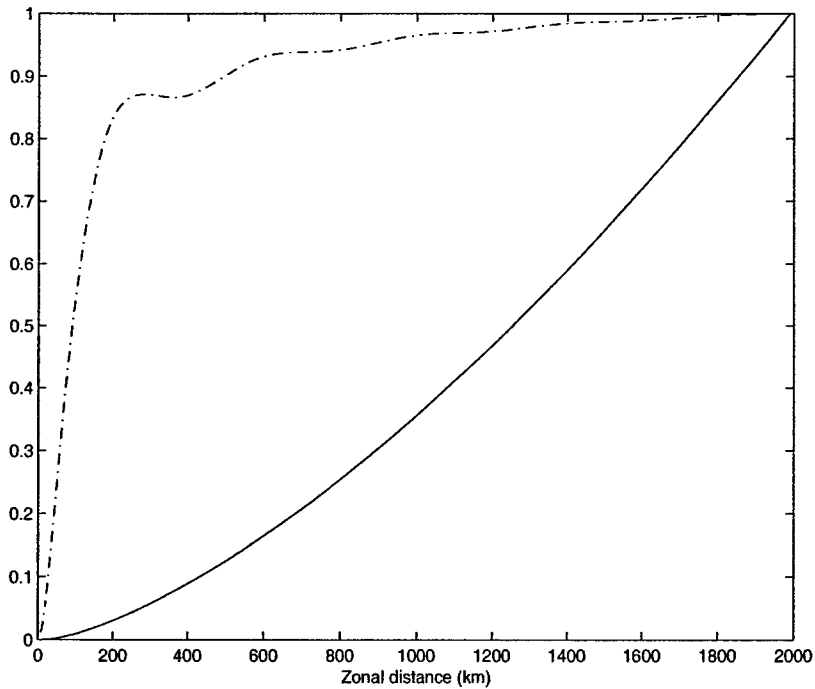
Figure 6-5: The normalized \sigma_{\Theta}^2(L, n, \lambda, \phi) (solid line) and \sigma_V^2(L, n, \lambda, \phi) (dashdot line) as a function of L . \sigma_{\Theta}^2(L, n, \lambda, \phi) and \sigma_V^2(L, n, \lambda, \phi) are normalized by \sigma_{\Theta}^2(L = 2000, n, \lambda, \phi) and \sigma_V^2(L = 2000, n, \lambda, \phi) , respectively.
