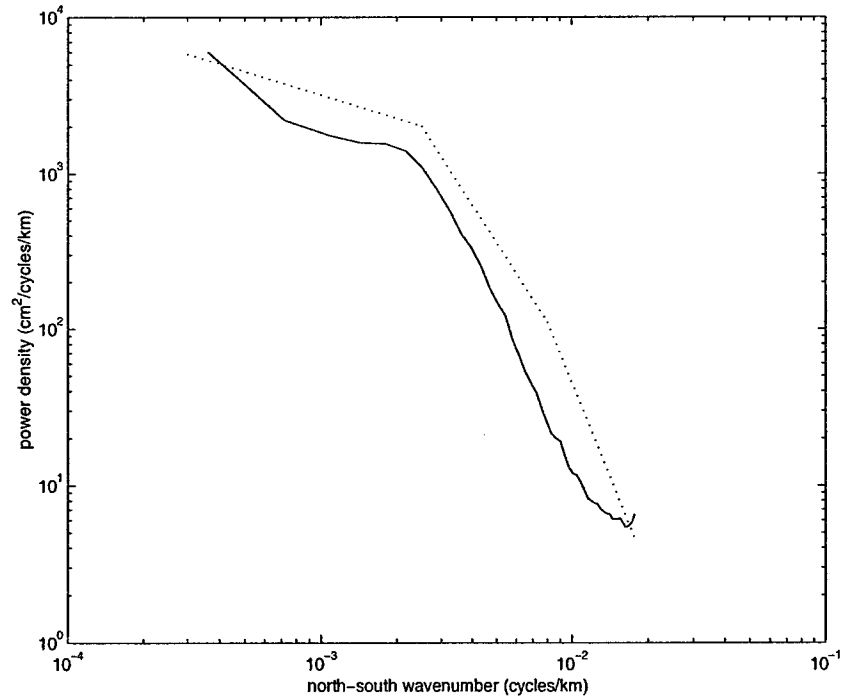
Figure 7-3: Scalar meridional-wavenumber spectrum of sea surface height. Solid line is the observed spectrum. Dotted line is the corresponding model spectrum.
