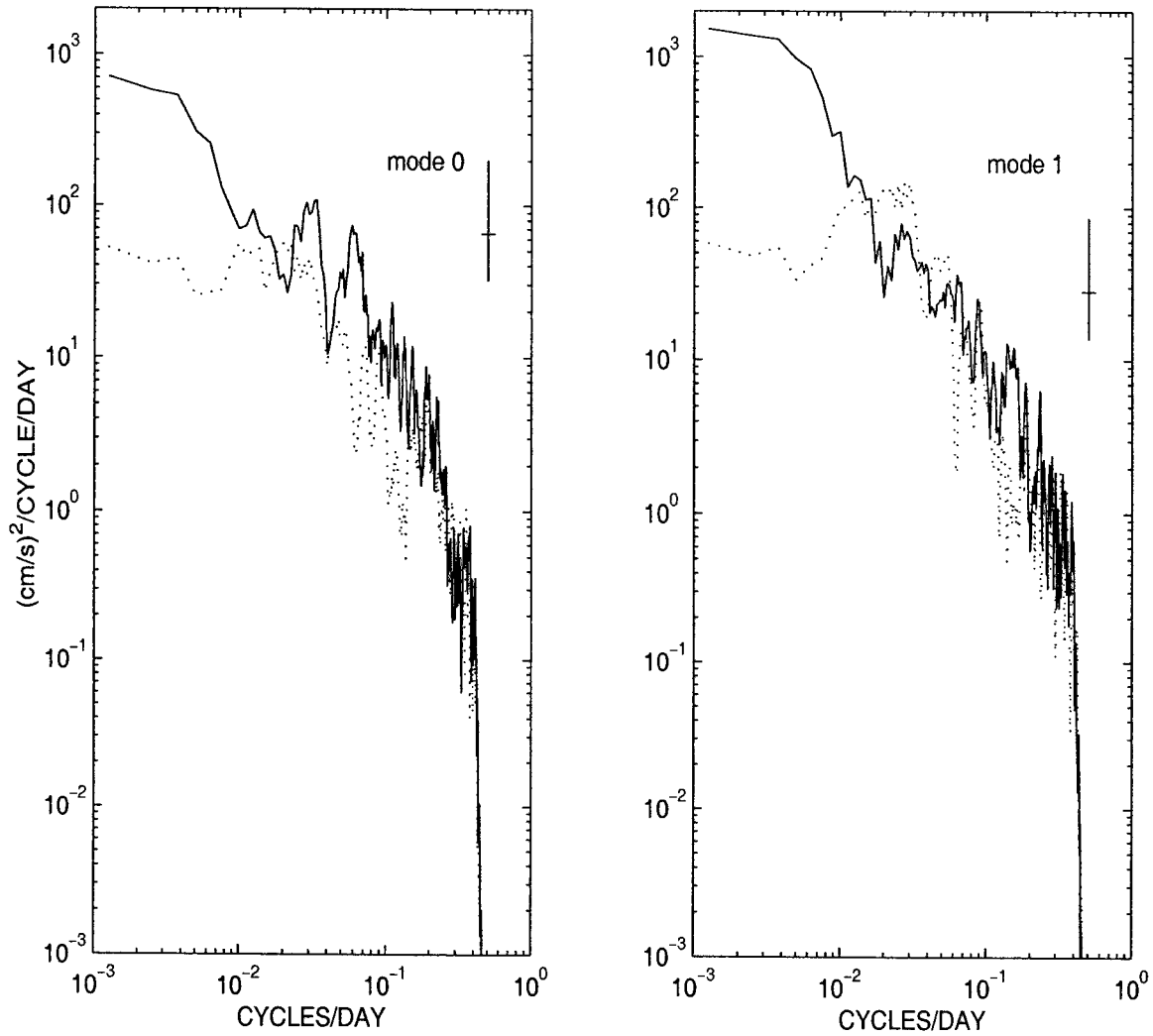
Figure 4-16: Frequency spectra for the zonal (solid line) and meridional (dotted line) component of horizontal velocity in the barotropic and first baroclinic mode at 38.8^\circ\text{N} , 68.1^\circ\text{W} . The spectra are estimated using D. Thompson's multitaper method (Percival and Walden, 1993). The ratio of the variance of zonal component to that of meridional component in the barotropic and first baroclinic mode is 3.5 and 2.7, respectively.
