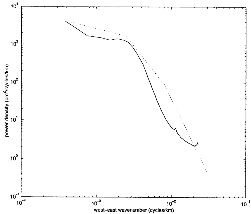
Figure 5-1: Zonal-wavenumber spectrum of sea surface height. Solid line is the observed spectrum. Dotted line is the corresponding model spectrum.
