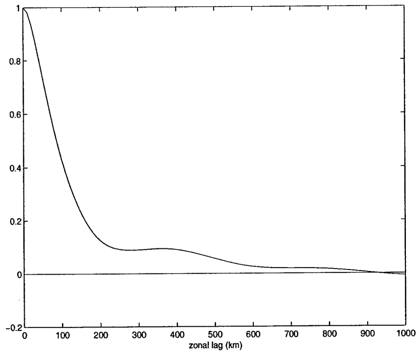
Figure 6-1: Temperature autocorrelation as a function of zonal separation distance.
