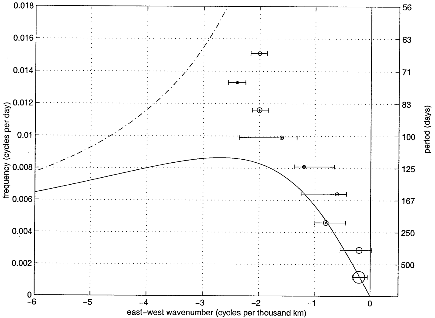
Figure 8-5: Frequency-zonal wave number spectra of region 4. The peak in each frequency band in Fig.8-4 is indicated by a dot here. The magnitude of each peak is denoted by the size of the circle around that peak. The dash-dot and solid curves denote the barotropic and first baroclinic Rossby wave dispersion curves with l = 0 , respectively. At the lowest frequencies, the barotropic curve is visually indistinguishable from k = 0 . Uncertainty estimates are derived from the 95% confidence interval (Capon and Goodman, 1970) for the peak values. The zonal wavenumber interval represents those wavenumbers where the background energy surrounding the apparent peak is larger than or equal to the lower limit of the confidence interval.
