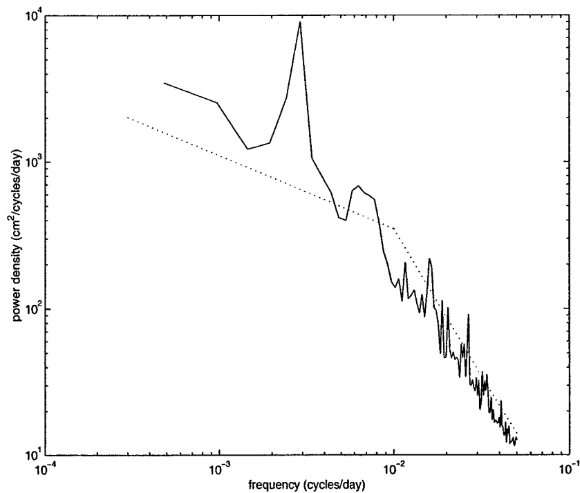
Figure 5-3: Frequency spectrum of sea surface height. Solid line is the observed spectrum. Dotted line is the corresponding model spectrum. There is a striking peak at the annual period on the observed spectrum.
