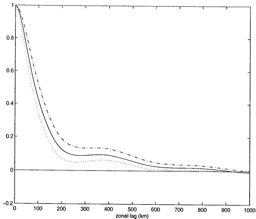
Figure 6-3: Uncertainty of the autocorrelation function. The solid line represents the autocorrelation function corresponding to the universal wavenumber spectrum in my model. The dashdot and dotted line correspond to the wavenumber spectrum with a slope of 15% more and 15% less than the slope of my universal spectrum, respectively.
