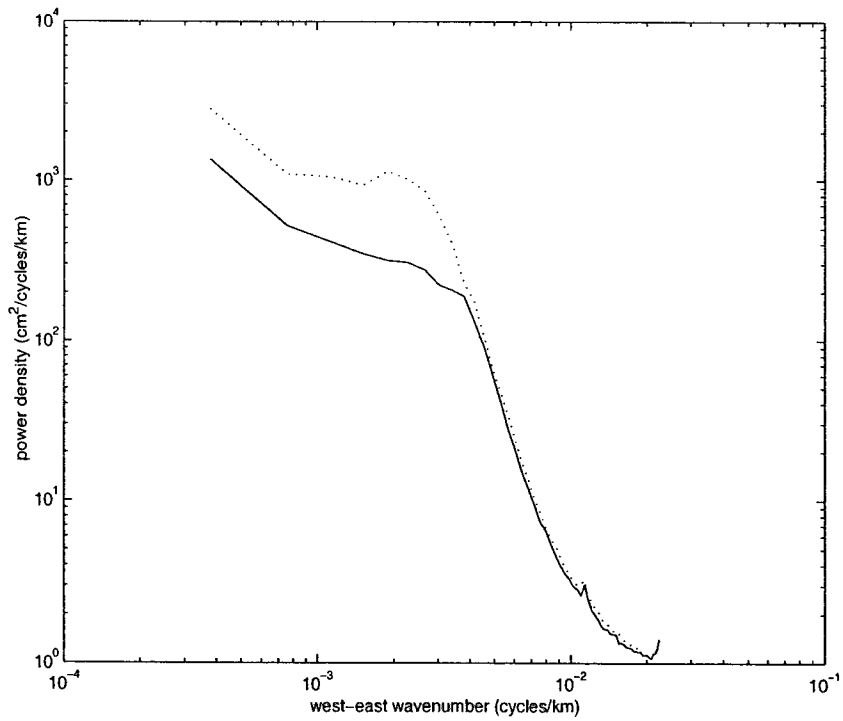
Figure 4-7: The zonal-wavenumber spectra of eastward-going (solid line) and westward-going motions (dotted line) in the T/P data.
