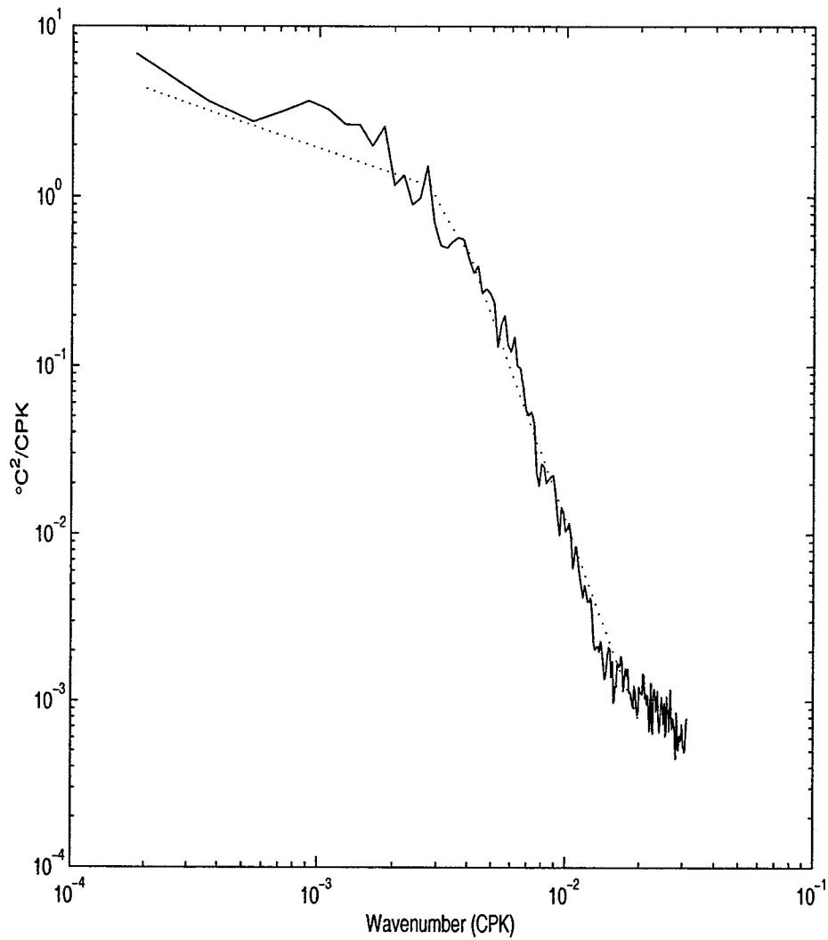
Figure 7-6: Scalar zonal-wavenumber spectrum temperature. Solid line is the observed spectrum. Dotted line is the corresponding model spectrum.
