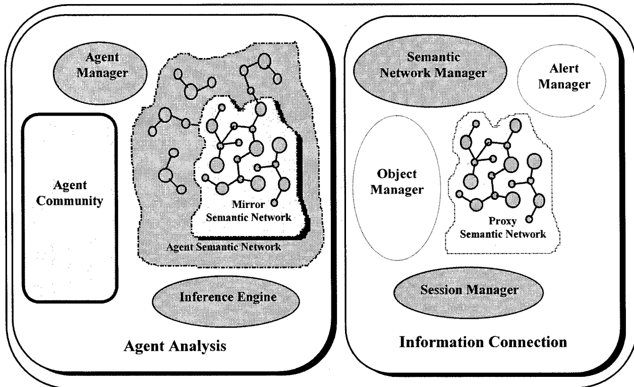
Figure 3 - Agent Session Architecture
