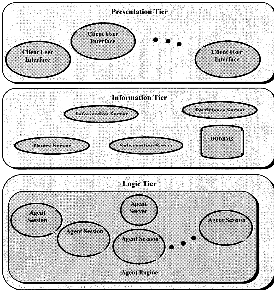
Figure 1 – 3-Tier Architecture
