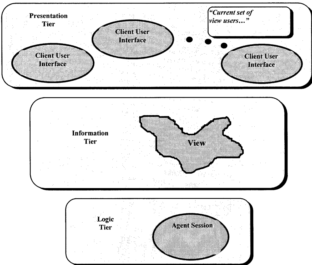
Figure 2 - Multiple users can interact with a view which in turn is analyzed by a single Agent Session
